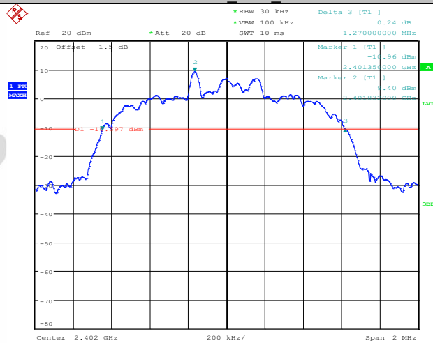
2DH5_Ant1_2402
