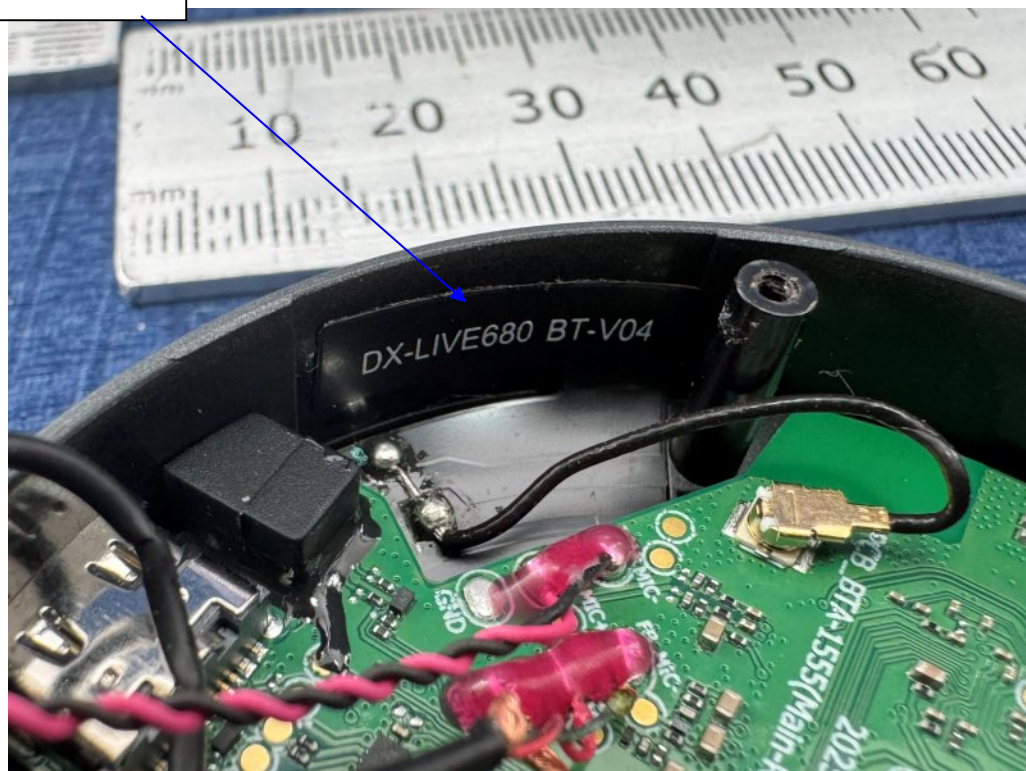
Bluetooth Antenna
