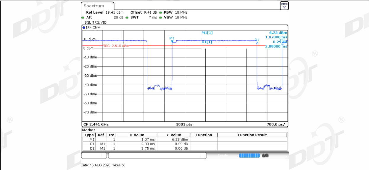
2DH5_Right_2441
