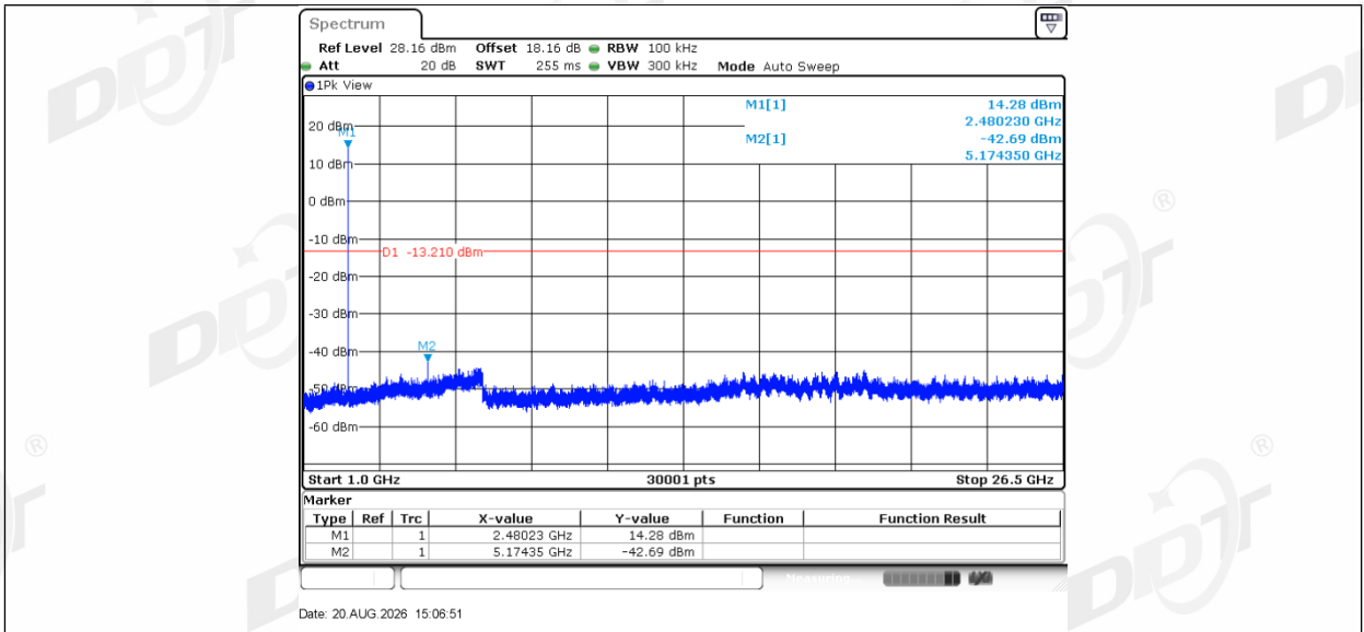
DH5_Right_2480_0~Reference
