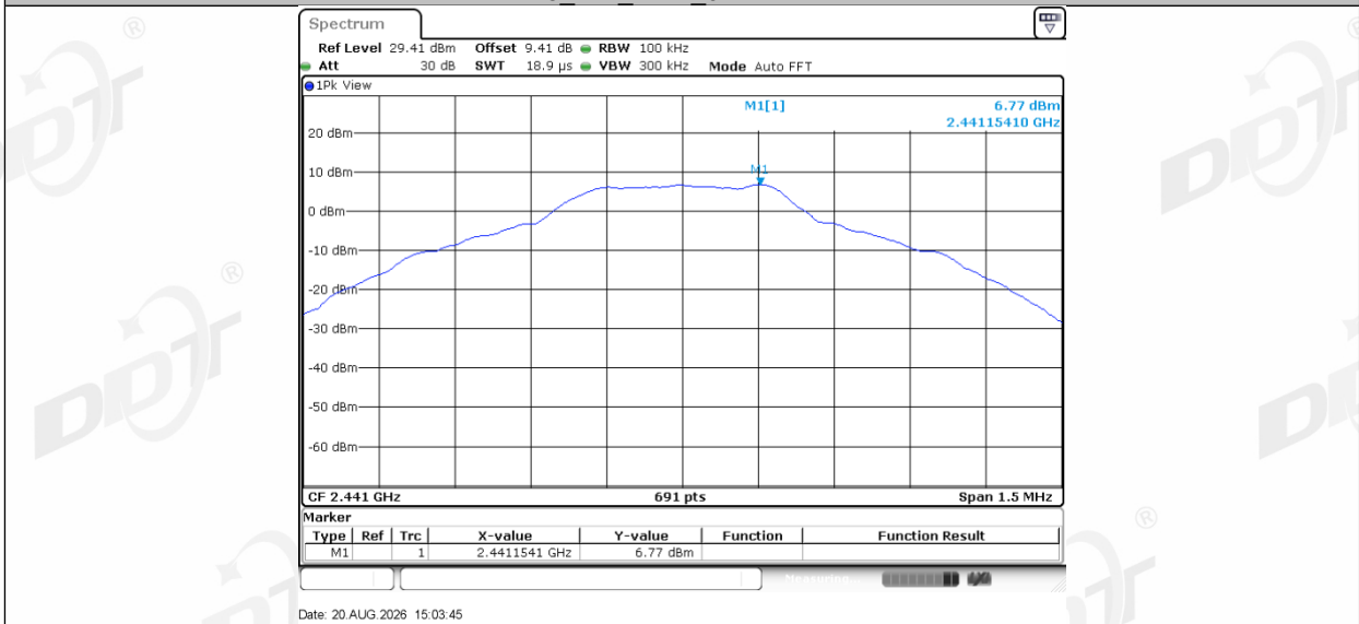
DH5 Left 2441_30~1000
