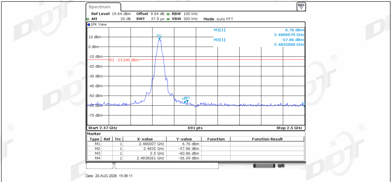
DH5 Right High 2480
