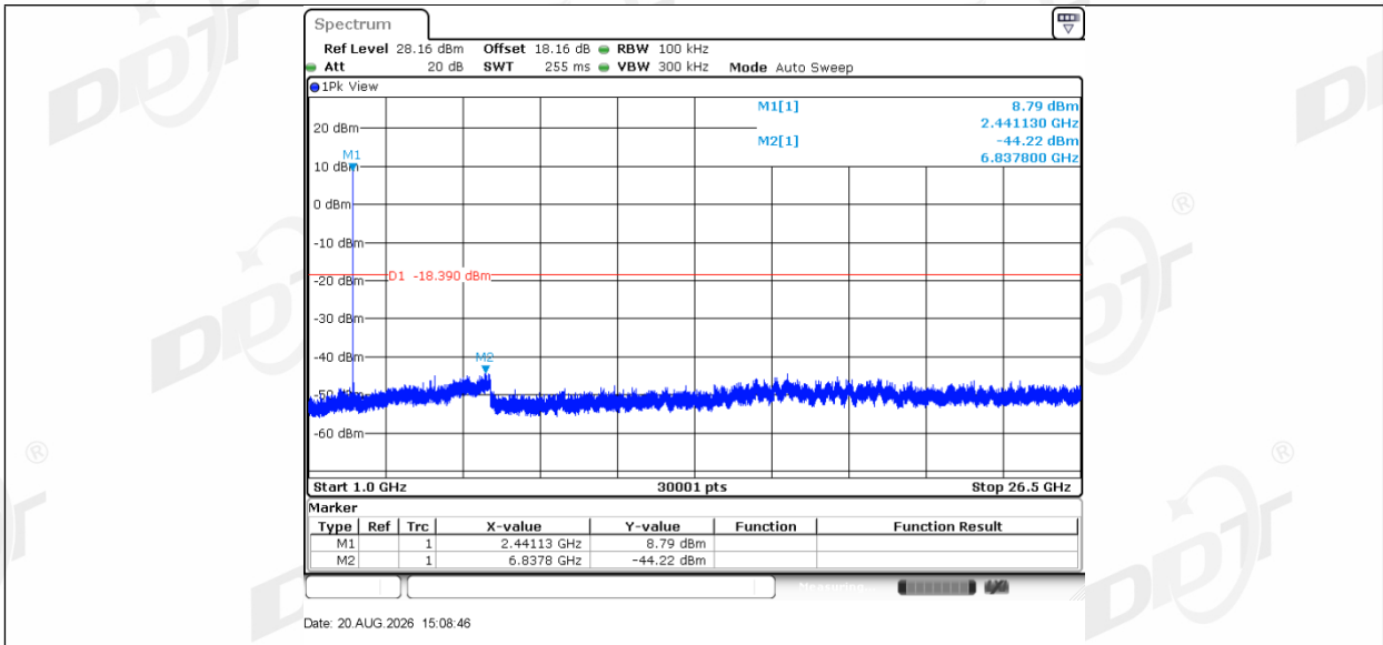
2DH5_Right_2441_0~Reference
