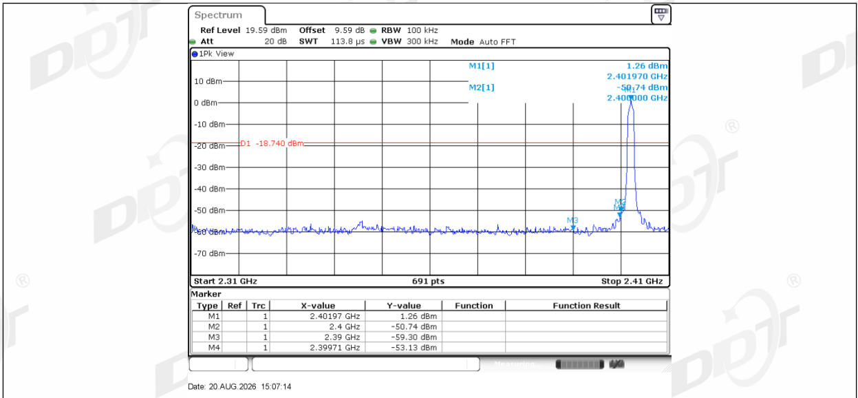
2DH5 Right Low 2402
