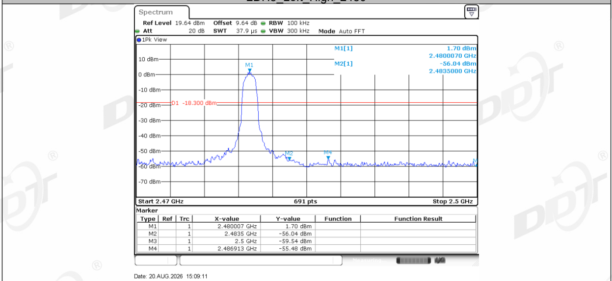
2DH5 Right High 2480
