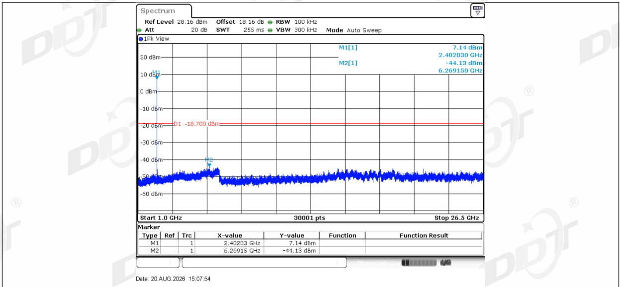
2DH5_Right_2402_0~Reference
