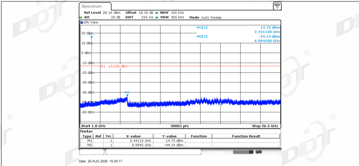
DH5_Right_2441_0~Reference
