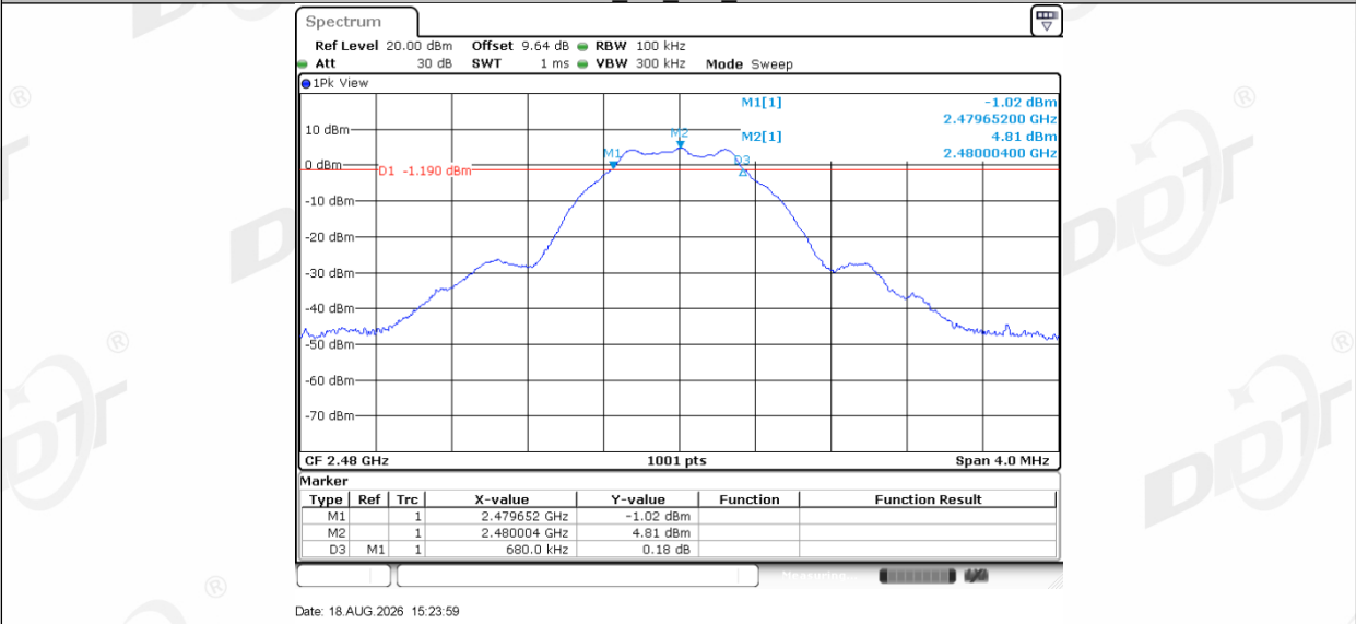
BLE_1M_Right_2480
