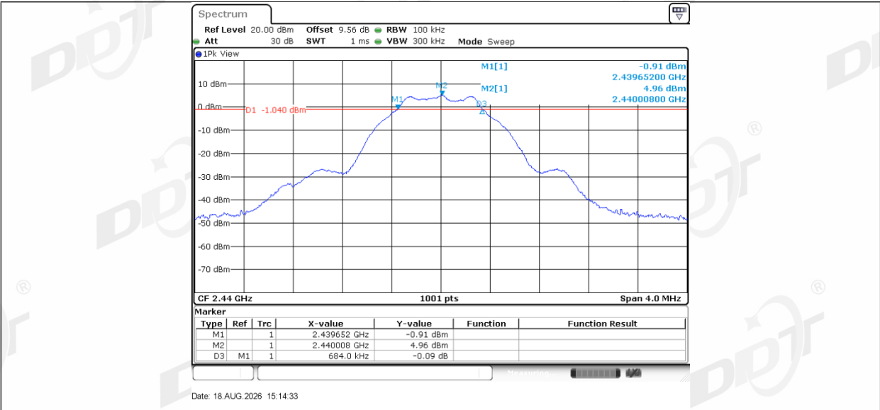
BLE_1M_Right_2440
