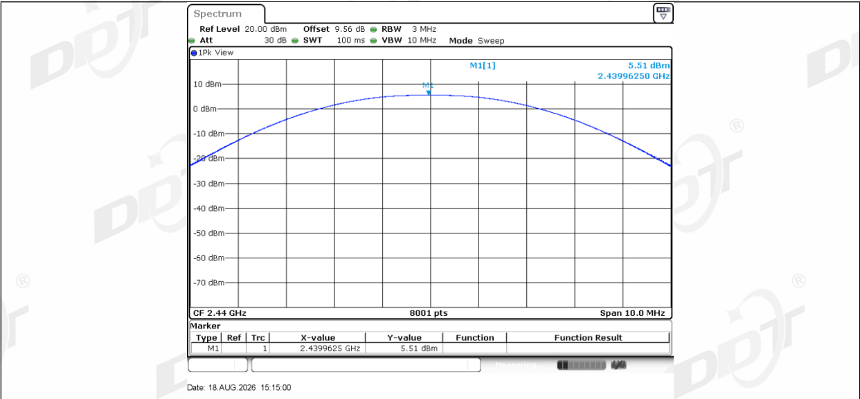
BLE_1M_Right_2440
