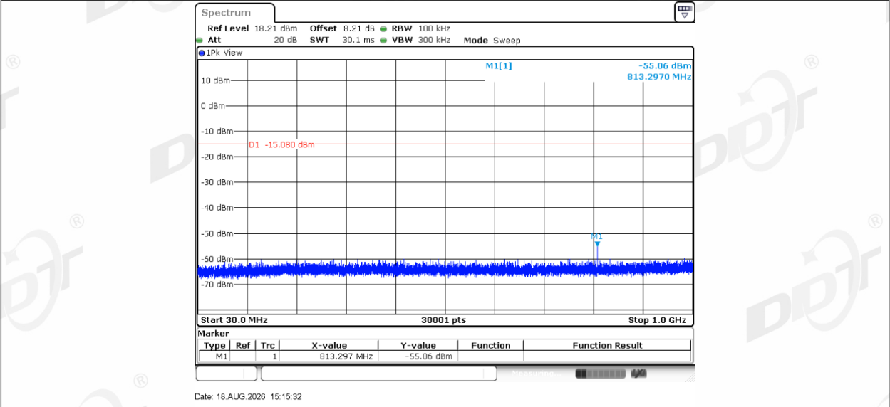
BLE_1M_Left_2440_1000~26500
