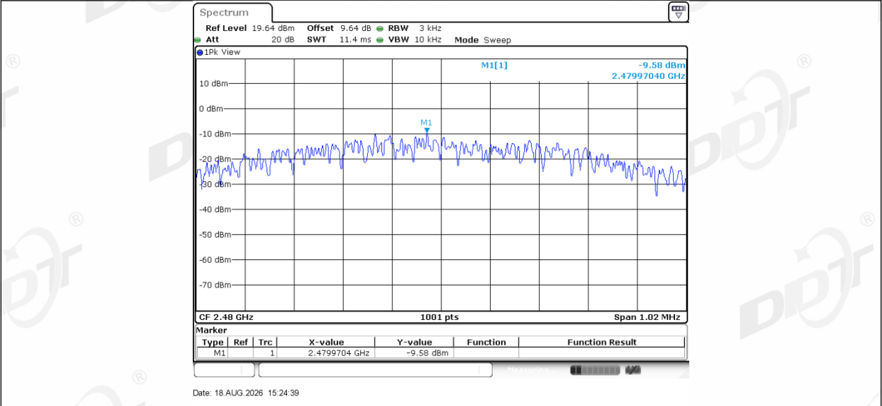
BLE_1M_Right_2480
