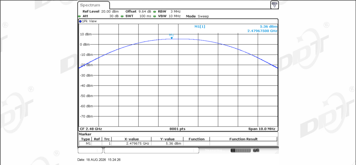
BLE_1M_Right_2480
