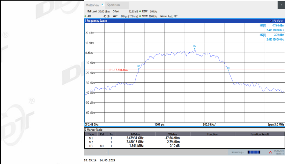
3DH5_Left side_2480
