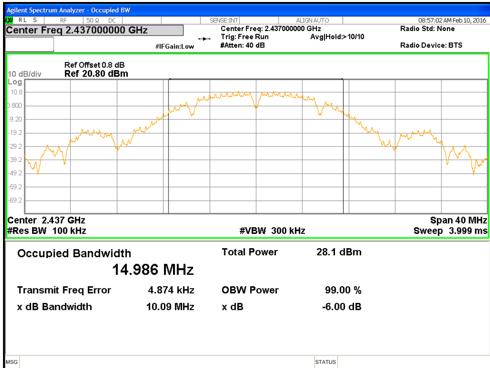
Figure 5: 6dB & 99% Occupied Bandwidth, 2437 MHz at 802.11b
