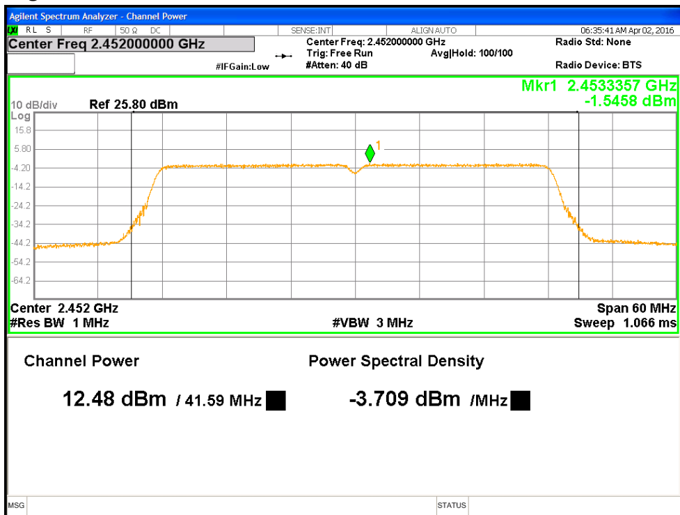
Figure 4: Maximum Transmitted Power, 2452 MHz at HT40 MCS0
