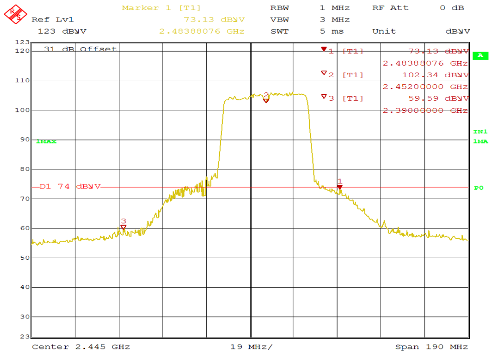
Figure 57: Radiated Emission at 2483.5 MHz Edge for 2452 MHz-HT40 – Vert. (Pk)
