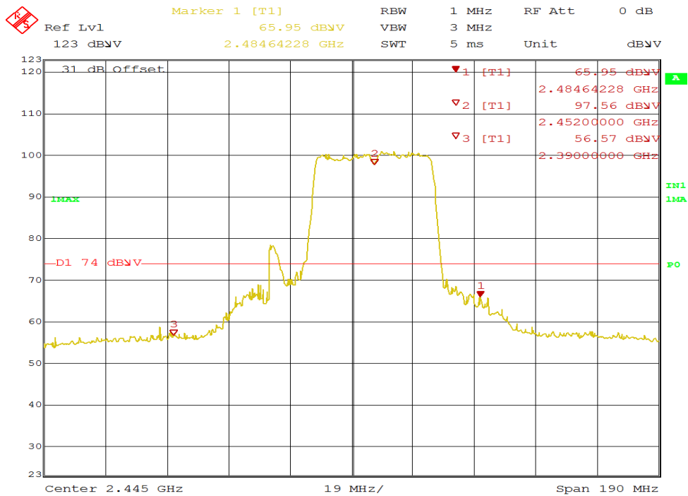
Figure 59: Radiated Emission at 2483.5 MHz Edge for 2452 MHz-HT40 – Horz. (Pk)
