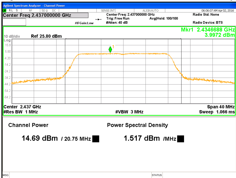
Figure 2: Maximum Transmitted Power, 2437 MHz at 11g 6Mbps
