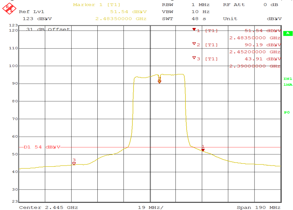
Figure 58: Radiated Emission at 2483.5 MHz Edge for 2452 MHz-HT40 – Vert. (Ave)
