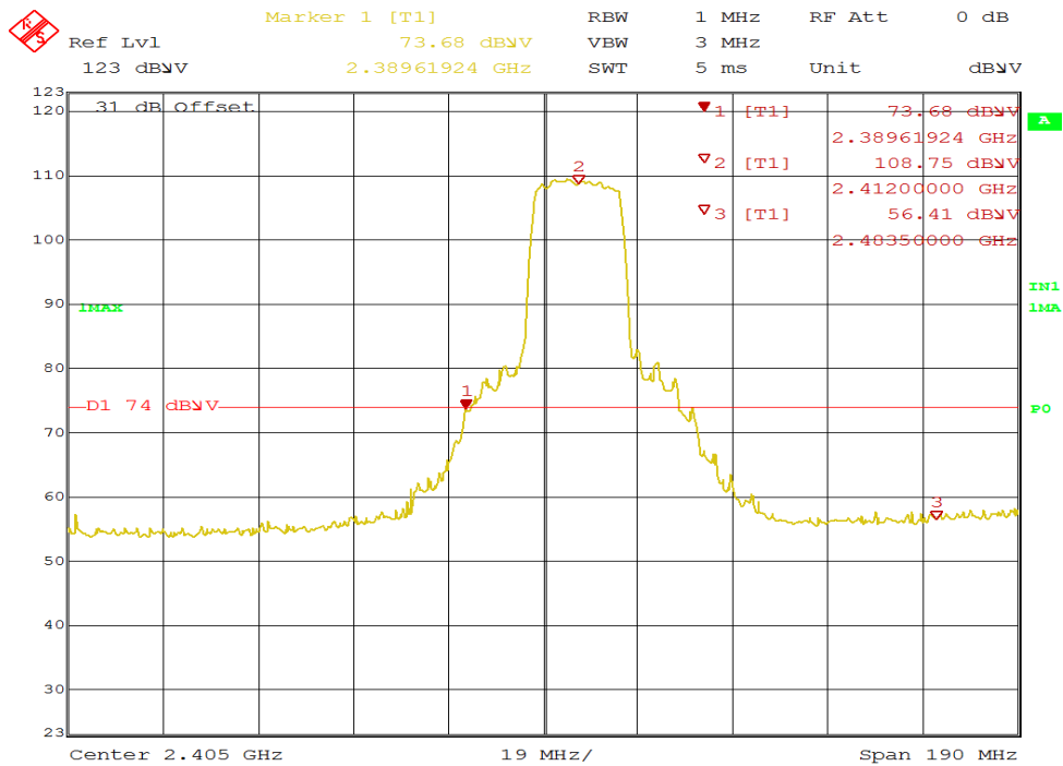
Figure 45: Radiated Emission at 2390 MHz Edge for 2412 MHz-HT20 – Vert. (Pk)
