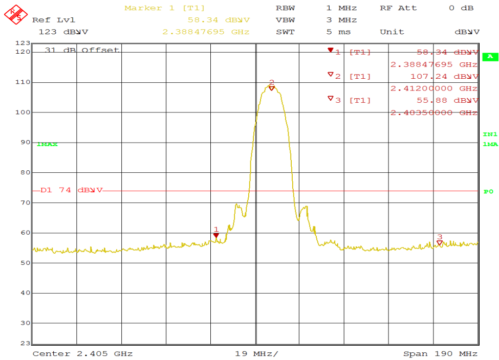
Figure 31: Radiated Emission at 2390 MHz Edge for 2412 MHz-802.11b – Horz. (Pk)
