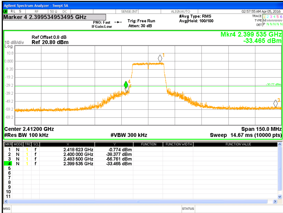
Figure 21: Measured Bandedge for HT20-MCS0 at 2412 MHz
