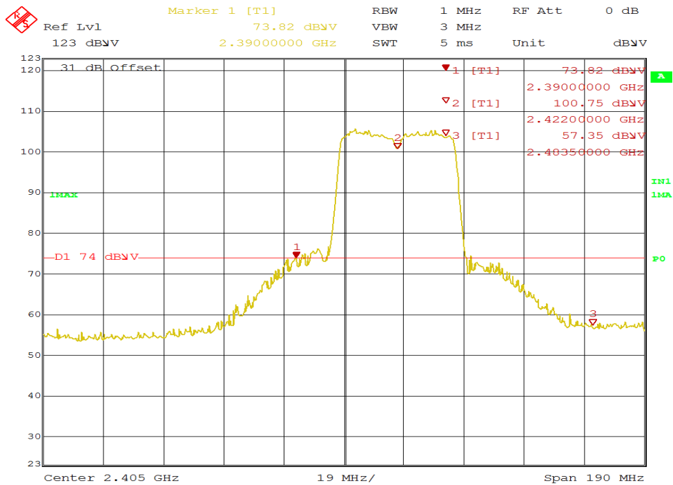
Figure 53: Radiated Emission at 2390 MHz Edge for 2422 MHz-HT40 – Vert. (Pk)
