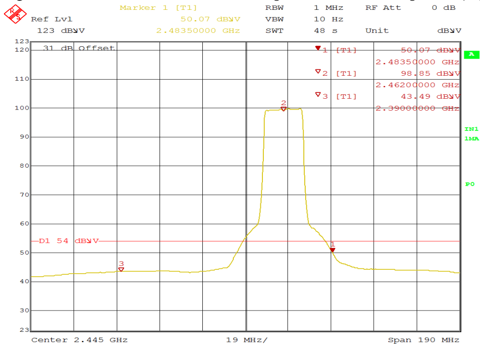
Figure 42: Radiated Emission at 2483.5 MHz Edge for 2462 MHz-802.11g – Vert. (Ave)
