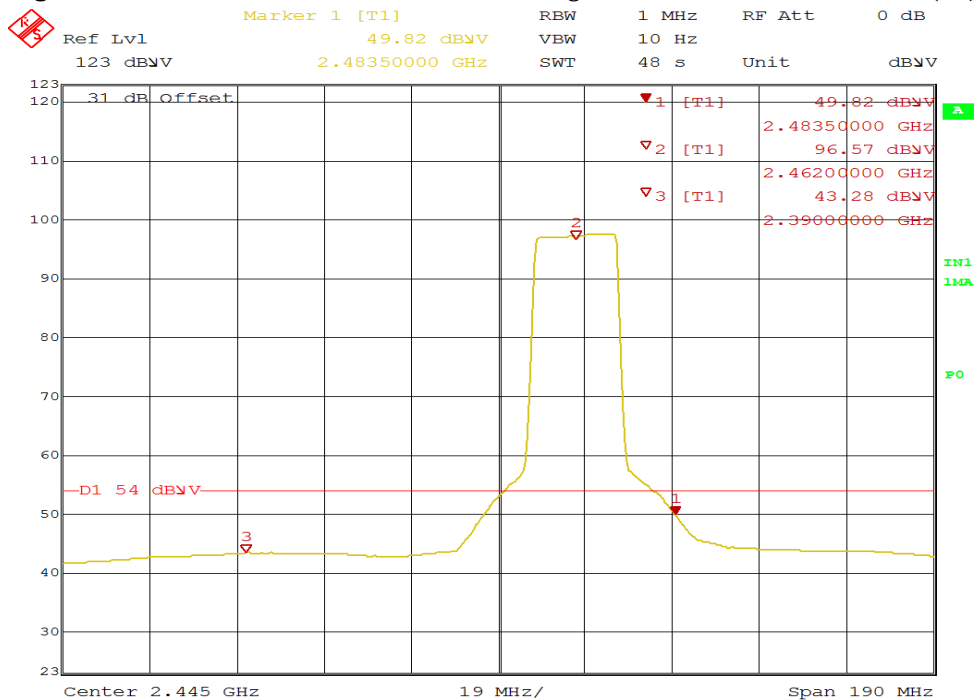
Figure 50: Radiated Emission at 2483.5 MHz Edge for 2462 MHz-HT20 – Vert. (Ave)
