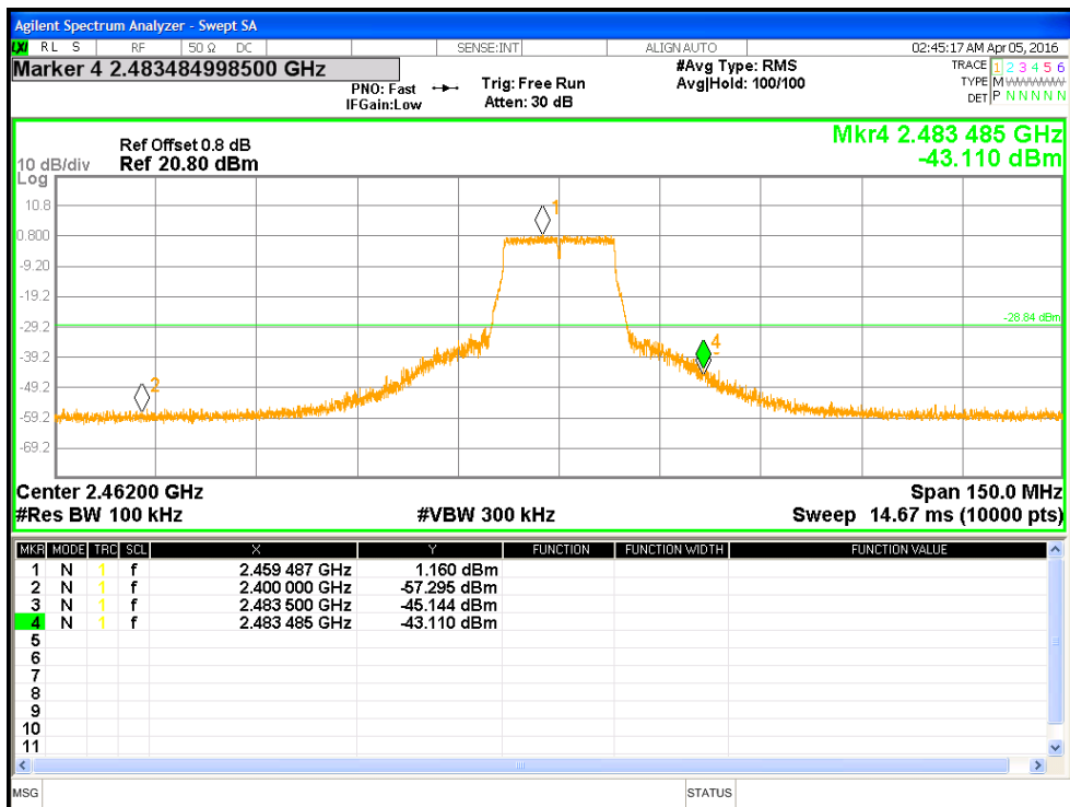
Figure 19: Measured Bandedge for 802.11g-6Mbps at 2462 MHz
