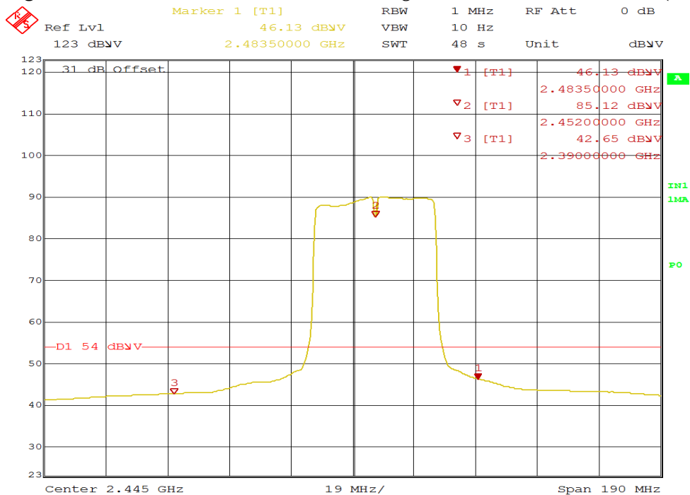
Figure 60: Radiated Emission at 2483.5 MHz Edge for 2452 MHz-HT40 – Horz. (Ave)
