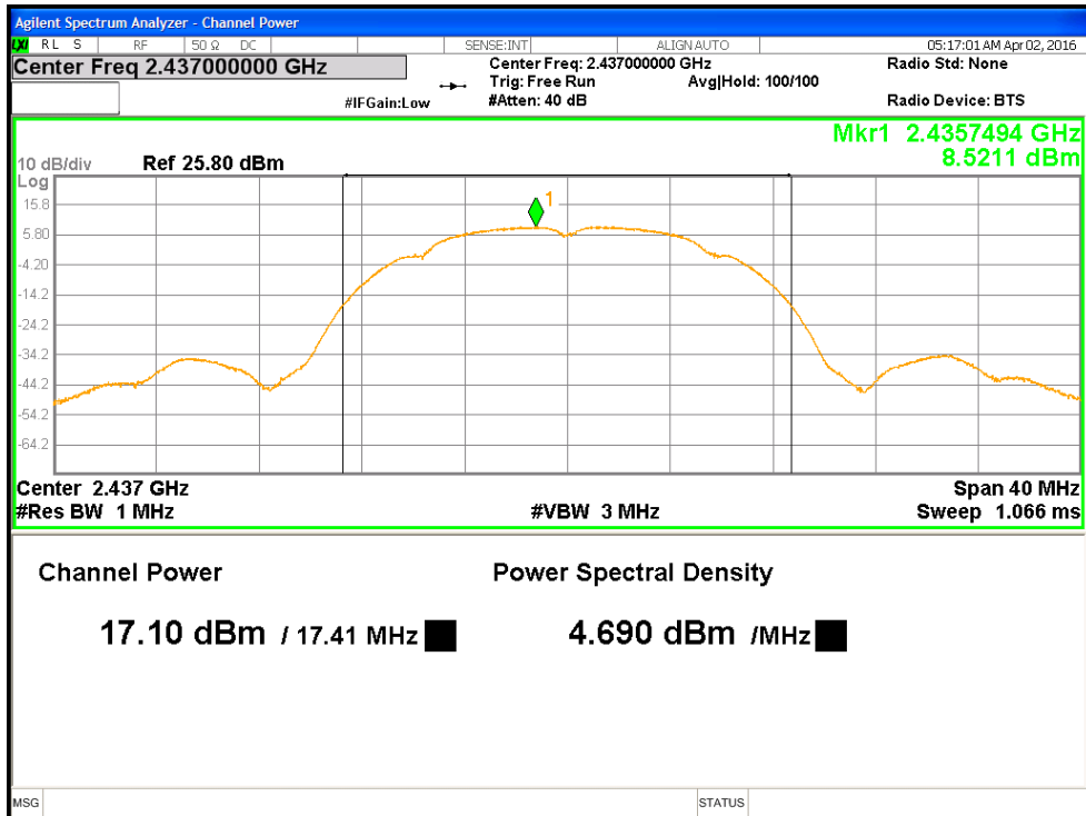
Figure 1: Maximum Transmitted Power, 2437 MHz at 11b 1Mbps
