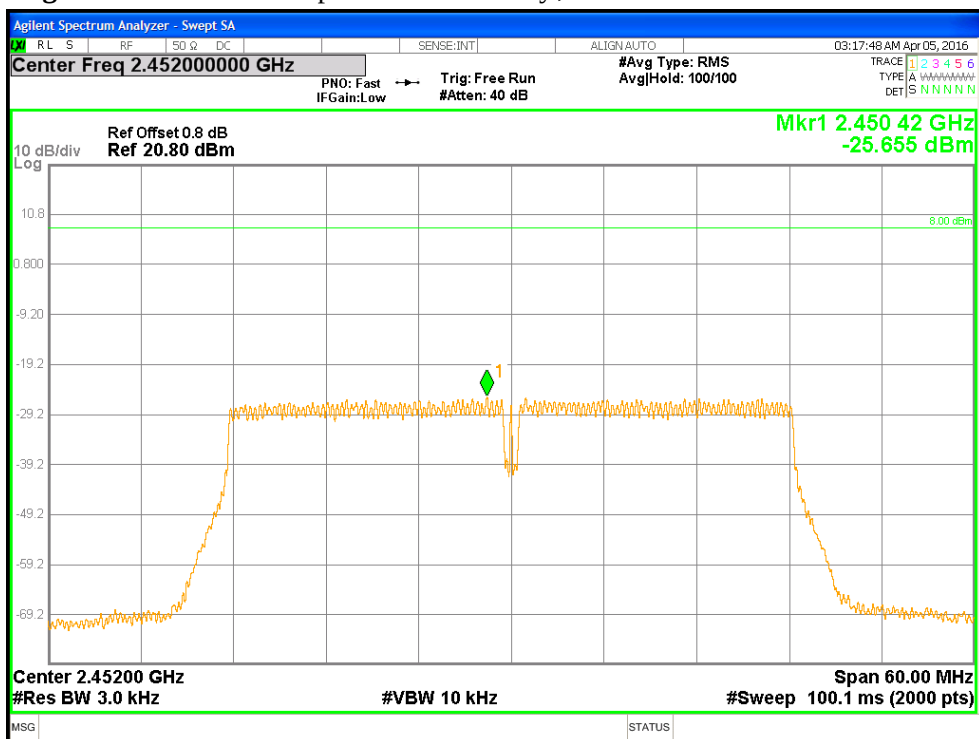
Figure 12: Power Spectral Density, 2452 MHz at HT40 MCS0
