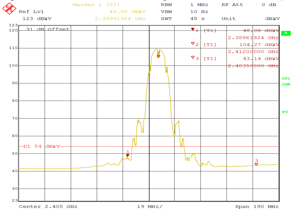
Figure 29: Radiated Emission at 2390 MHz Edge for 2412 MHz-802.11b – Vert. (Pk)
