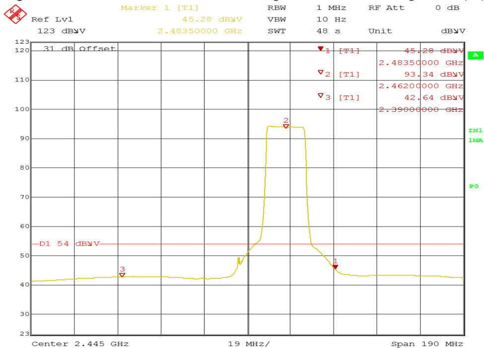
Figure 44: Radiated Emission at 2483.5 MHz Edge for 2462 MHz-802.11g – Horz. (Ave)
