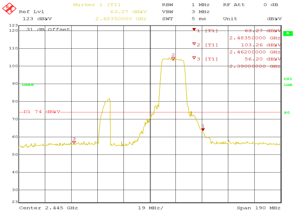
Figure 43: Radiated Emission at 2483.5 MHz Edge for 2462 MHz-802.11g – Horz. (Pk)
