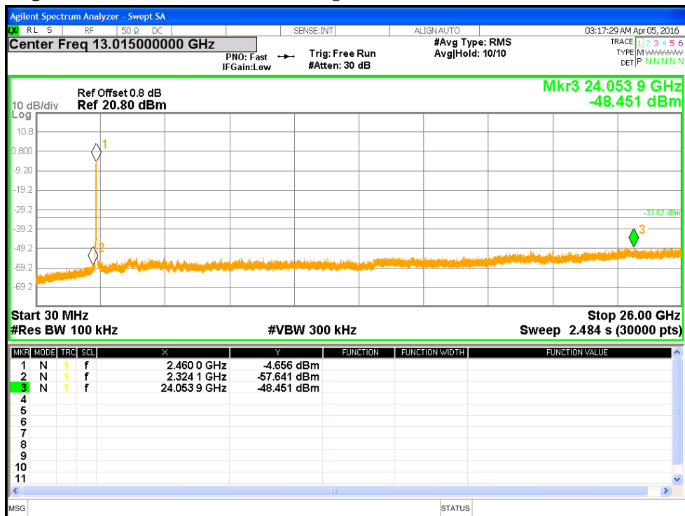
Figure 28: Out of Band Emissions for HT40-MCS0 at 2452 MHz
