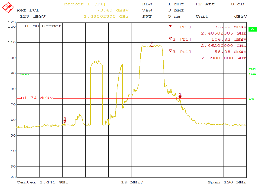
Figure 49: Radiated Emission at 2483.5 MHz Edge for 2462 MHz-HT20 – Vert. (Pk)
