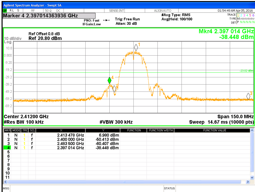
Figure 13: Measured Bandedge for 802.11b-1Mbps at 2412 MHz
