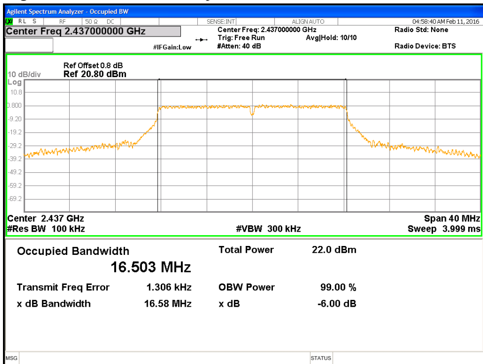
Figure 6: 6dB & 99% Occupied Bandwidth, 2437 MHz at 802.11g
