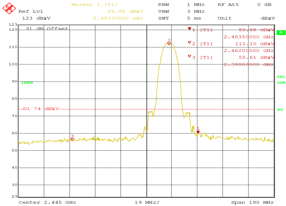
Figure 33: Radiated Emission at 2483.5 MHz Edge for 2462 MHz-802.11b – Vert. (Pk)
