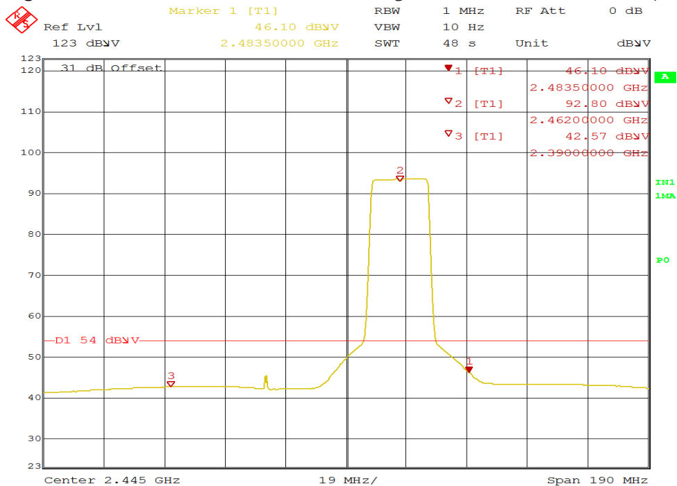
Figure 52: Radiated Emission at 2483.5 MHz Edge for 2462 MHz-HT20 – Horz. (Ave)
