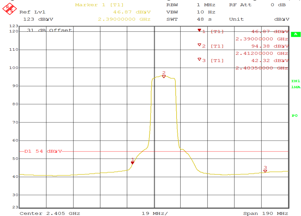
Figure 40: Radiated Emission at 2390 MHz Edge for 2412 MHz-802.11g – Horz. (Ave)
