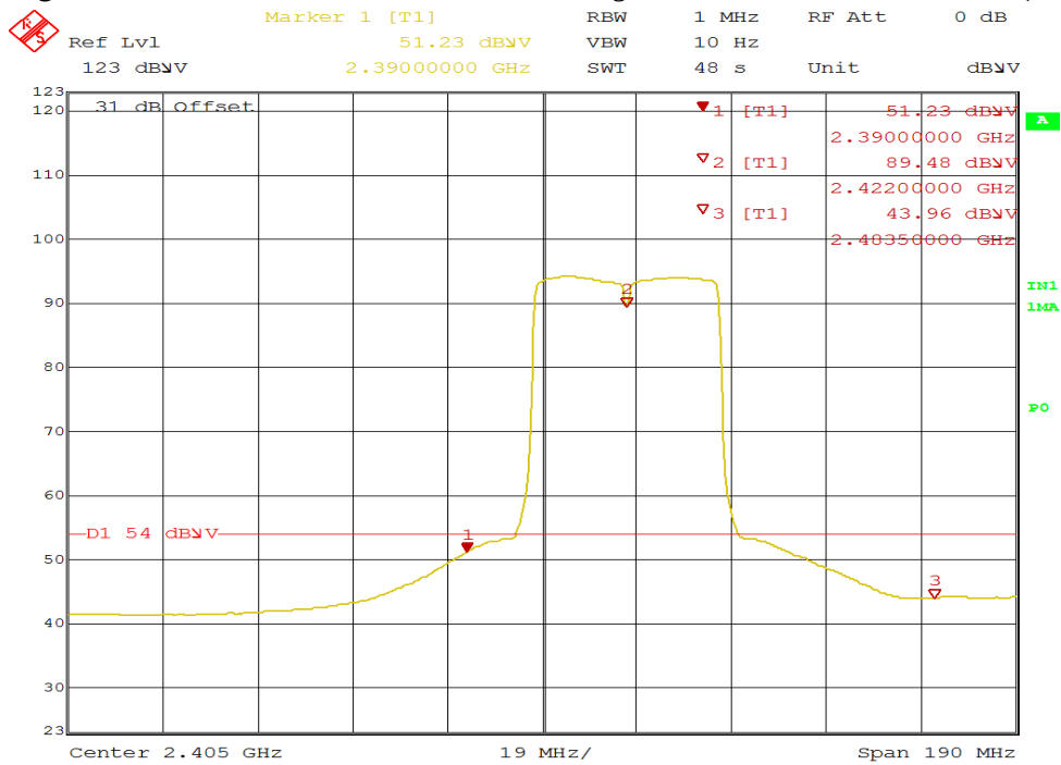
Figure 54: Radiated Emission at 2390 MHz Edge for 2422 MHz-HT40 – Vert. (Ave)
