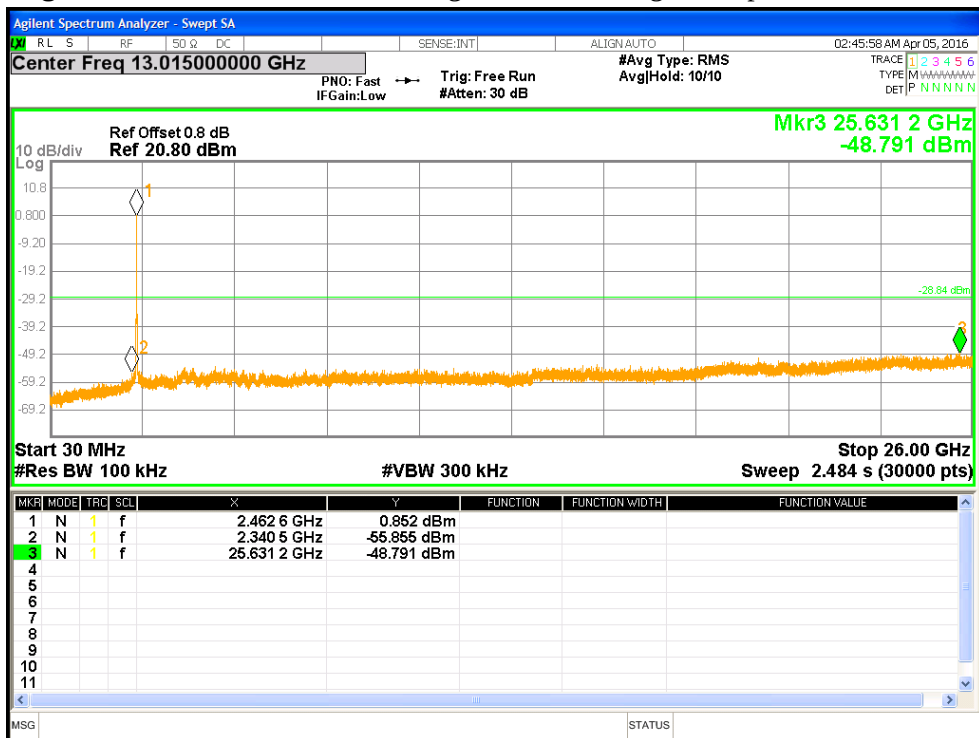
Figure 20: Out of Band Emissions for 802.11g-6Mbps at 2462 MHz
