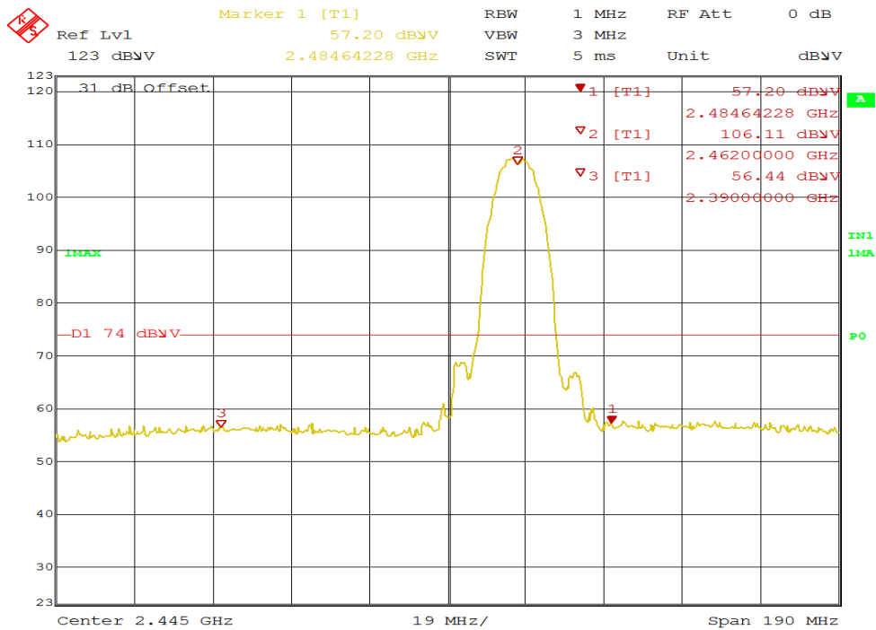
Figure 35: Radiated Emission at 2483.5 MHz Edge for 2462 MHz-802.11b – Horz. (Pk)
