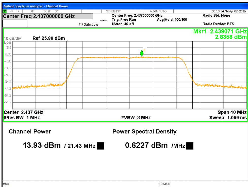
Figure 3: Maximum Transmitted Power, 2437 MHz at HT20 MCS0
