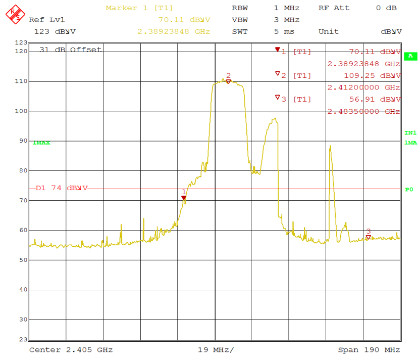
Figure 37: Radiated Emission at 2390 MHz Edge for 2412 MHz-802.11g – Vert. (Pk)
