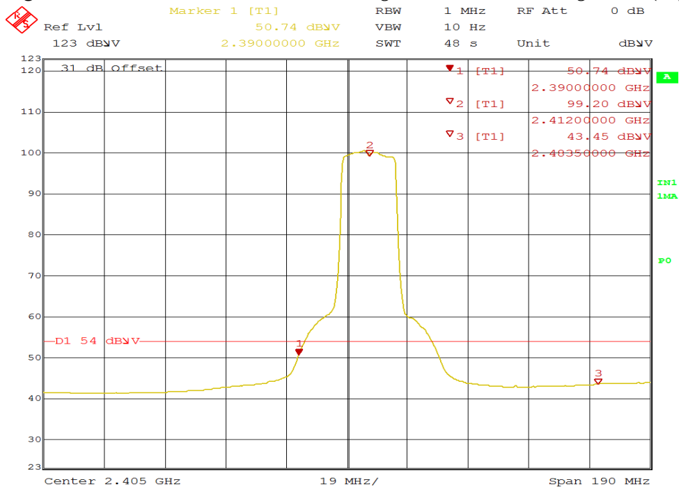
Figure 38: Radiated Emission at 2390 MHz Edge for 2412 MHz-802.11g – Vert. (Ave)
