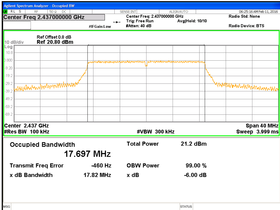
Figure 7: 6dB & 99% Occupied Bandwidth, 2437 MHz at HT20
