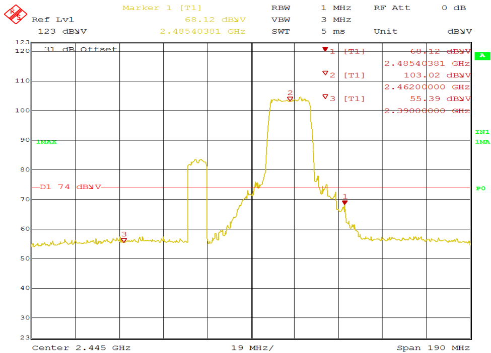
Figure 51: Radiated Emission at 2483.5 MHz Edge for 2462 MHz-HT20 – Horz. (Pk)
