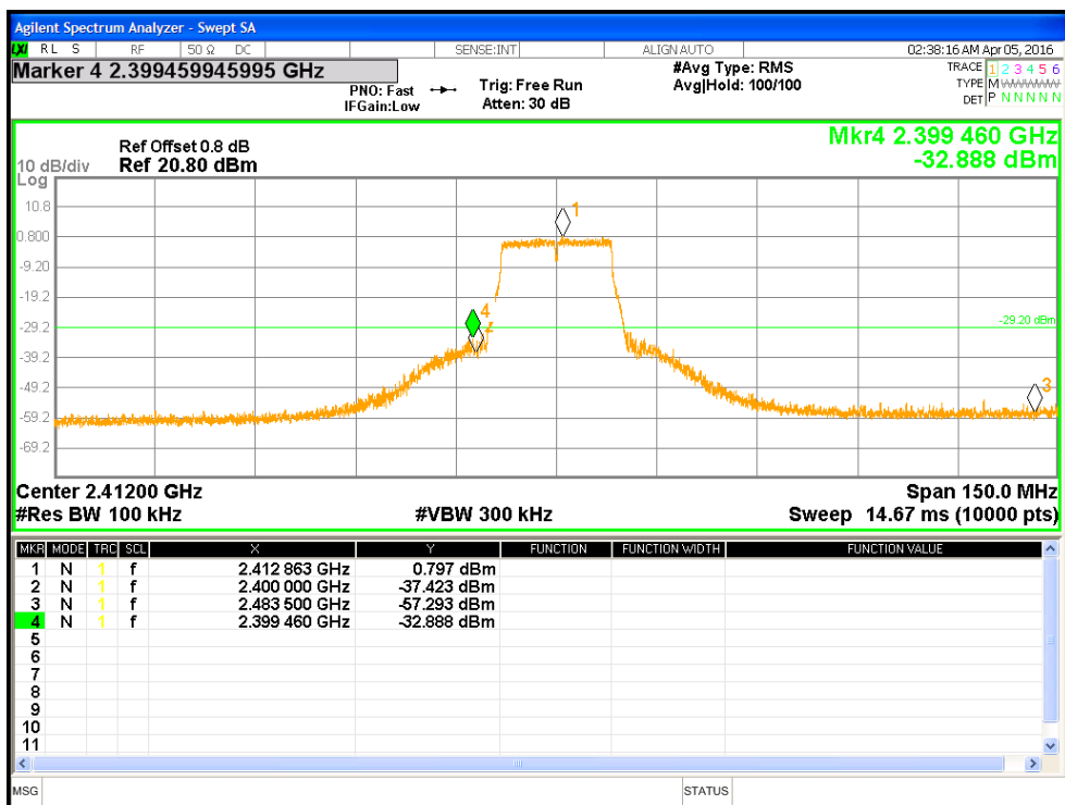
Figure 17: Measured Bandedge for 802.11g-6Mbps at 2412 MHz
