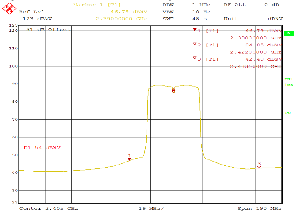
Figure 55: Radiated Emission at 2390 MHz Edge for 2422 MHz-HT40 – Horz. (Pk)
