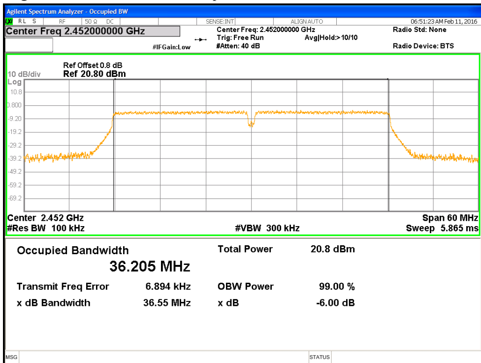
Figure 8: 6dB & 99% Occupied Bandwidth, 2452 MHz at HT40
