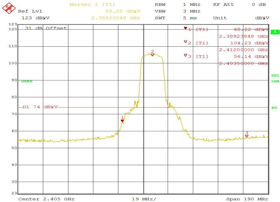
Figure 39: Radiated Emission at 2390 MHz Edge for 2412 MHz-802.11g – Horz. (Pk)
