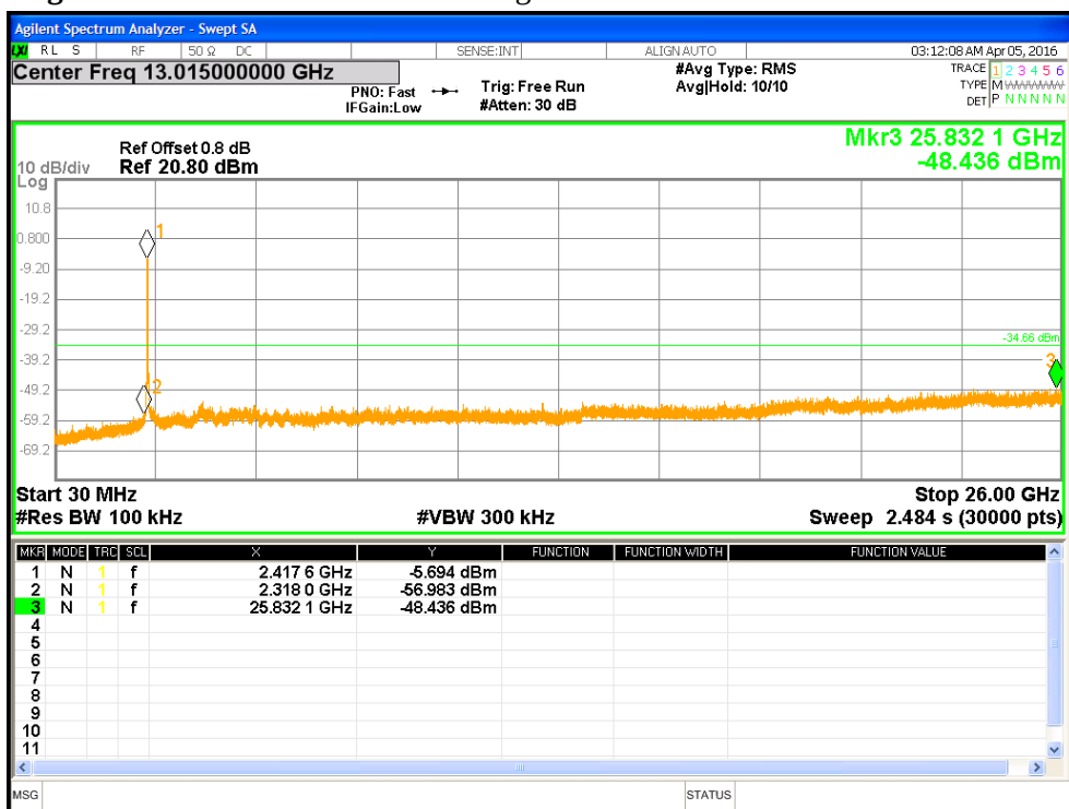
Figure 26: Out of Band Emissions for HT40-MCS0 at 2422 MHz
