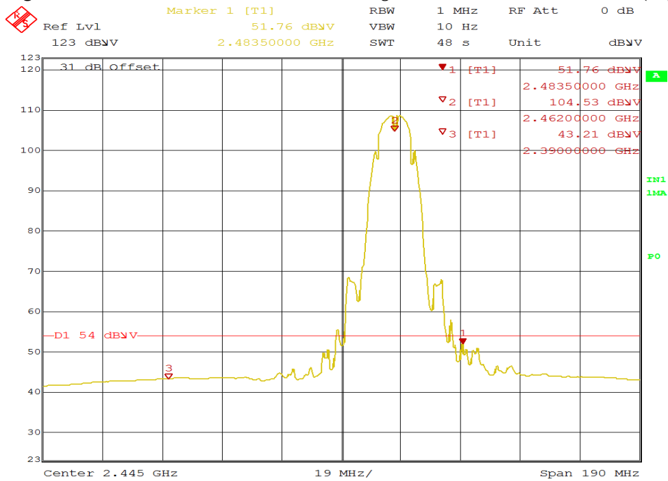
Figure 34: Radiated Emission at 2483.5 MHz Edge for 2462 MHz-802.11b – Vert. (Ave)
