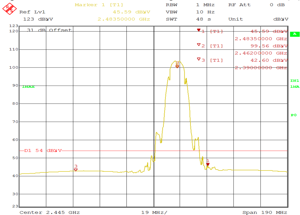
Figure 36: Radiated Emission at 2483.5 MHz Edge for 2462 MHz-802.11b – Horz. (Ave)
