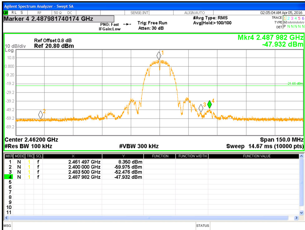
Figure 15: Measured Bandedge for 802.11b-1Mbps at 2462 MHz
