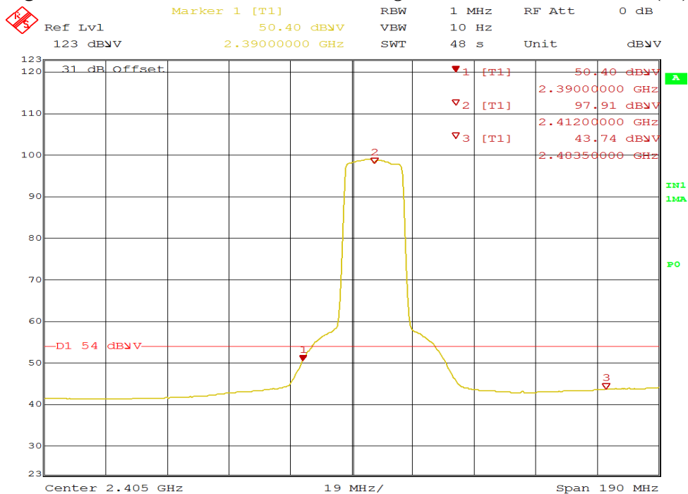
Figure 46: Radiated Emission at 2390 MHz Edge for 2412 MHz-HT20 – Vert. (Ave)
