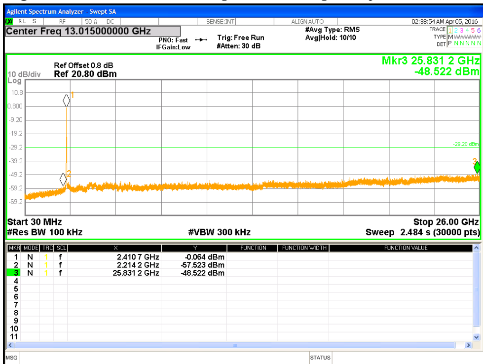
Figure 18: Out of Band Emissions for 802.11g-6Mbps at 2412 MHz
