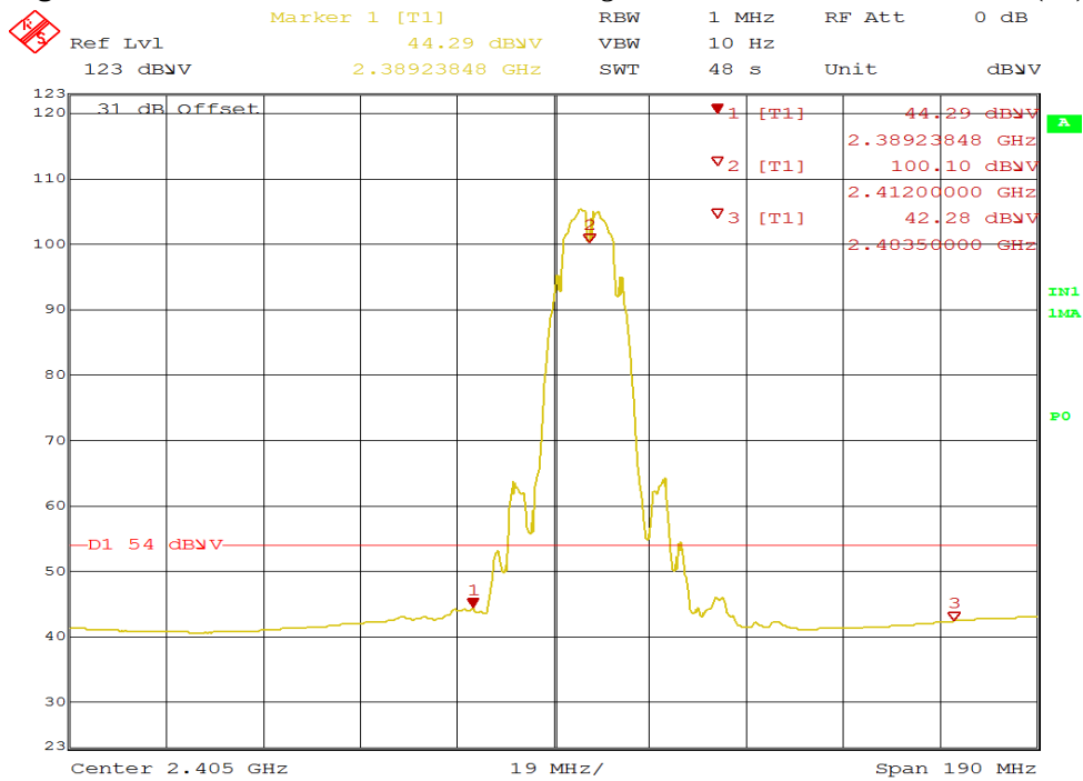
Figure 32: Radiated Emission at 2390 MHz Edge for 2412 MHz-802.11b – Horz. (Ave)
