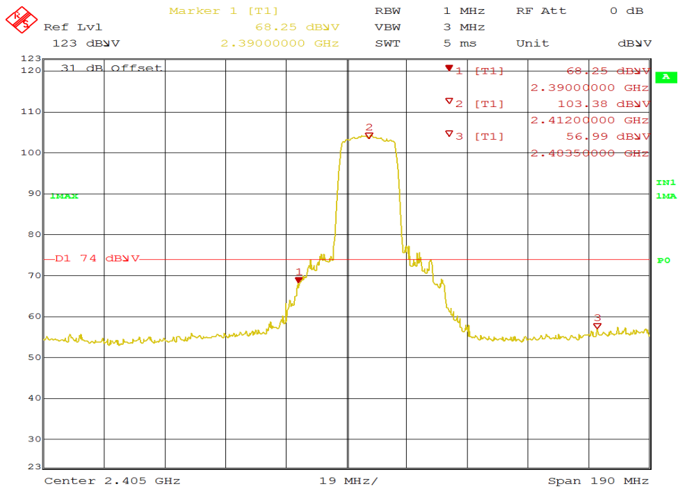
Figure 47: Radiated Emission at 2390 MHz Edge for 2412 MHz-HT20 – Horz. (Pk)
