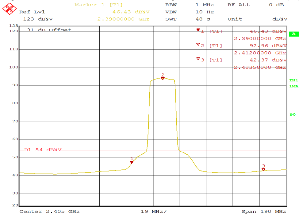
Figure 48: Radiated Emission at 2390 MHz Edge for 2412 MHz-HT20 – Horz. (Ave)
