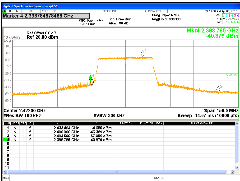
Figure 25: Measured Bandedge for HT40-MCS0 at 2422 MHz
