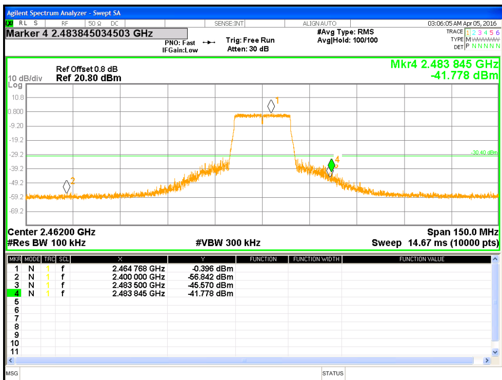
Figure 23: Measured Bandedge for HT20-MCS0 at 2462 MHz
