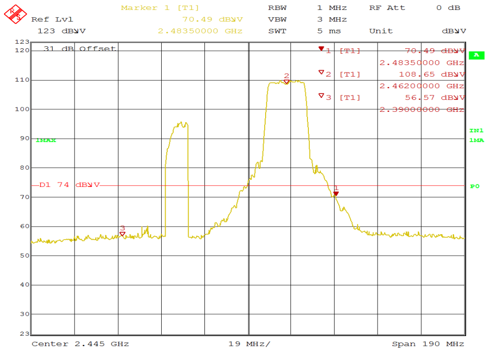
Figure 41: Radiated Emission at 2483.5 MHz Edge for 2462 MHz-802.11g – Vert. (Pk)
