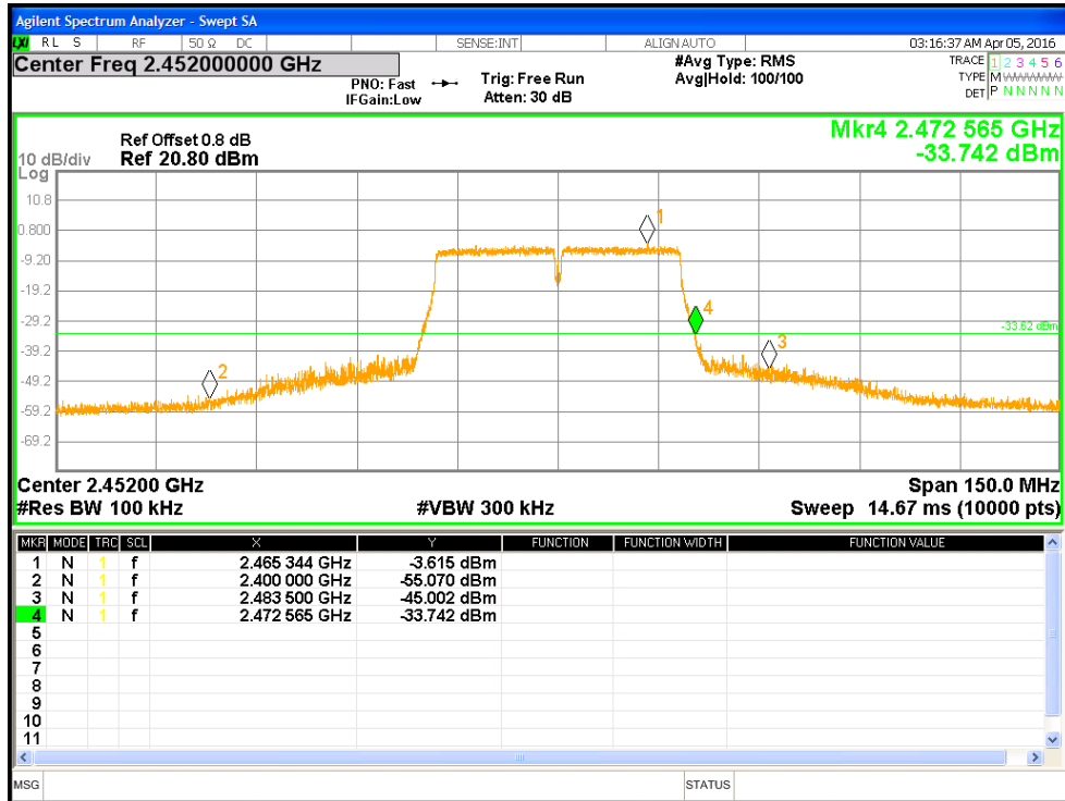
Figure 27: Measured Bandedge for HT40-MCS0 at 2452 MHz
