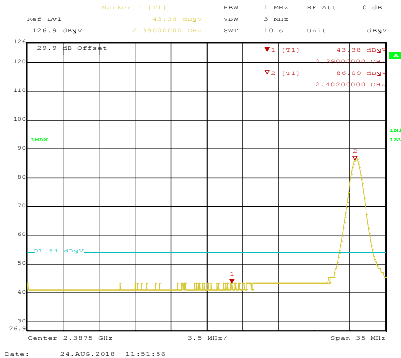
Figure 38: Radiated Emission at the 2390 MHz Edge for Channel 2402 MHz at DH1 – Horizontal (Avg)
