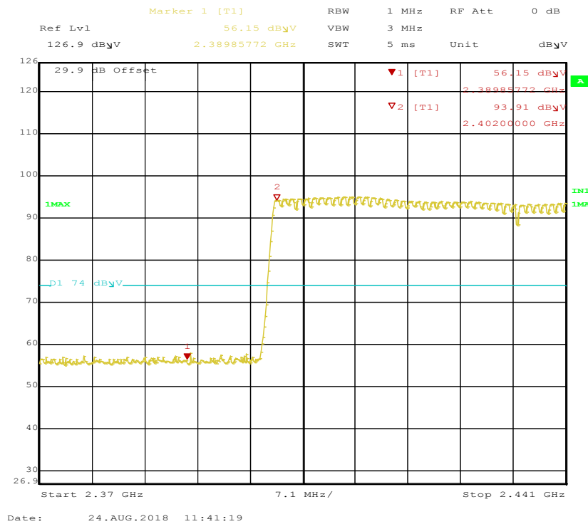
Figure 48: Radiated Emission at the 2390 MHz Edge for Hopping Channel at DH1 – Vertical (Pk)
