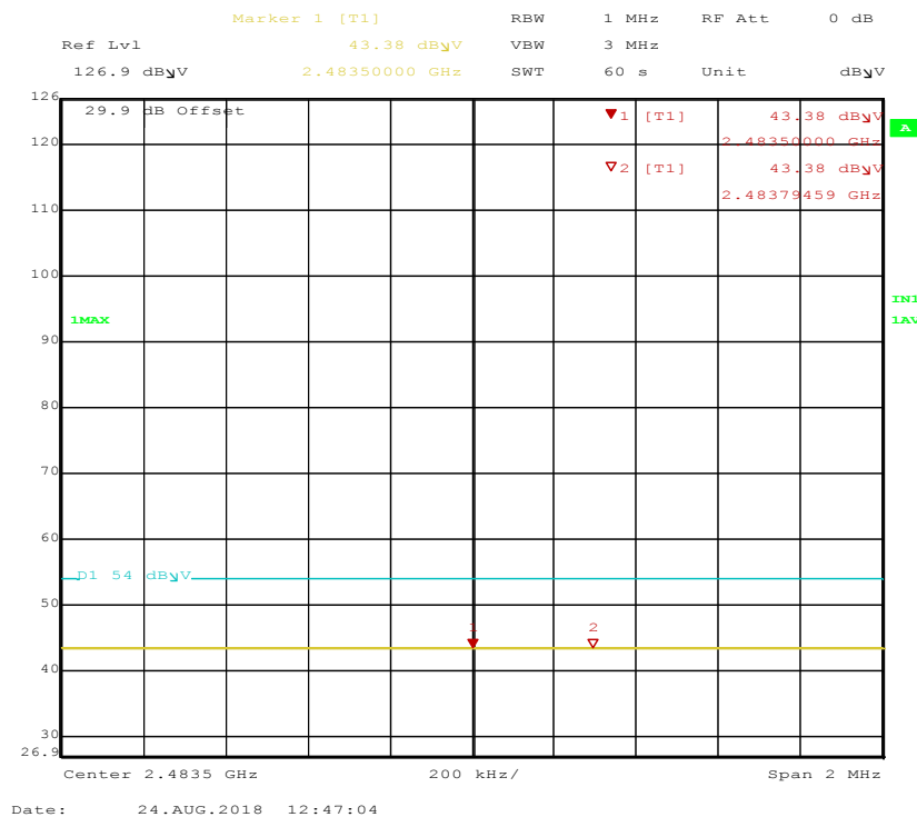
Figure 63: Radiated Emission at the 2483.5 MHz, 2 MHz Span, for Hopping Channel at DH1 – Horizontal (Avg)
