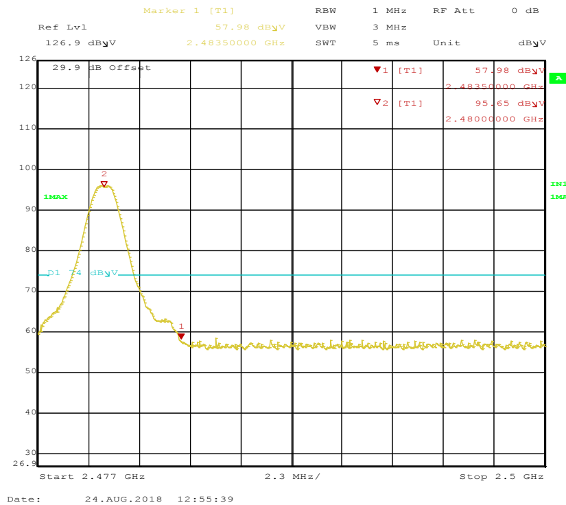
Figure 40: Radiated Emission at the 2483.5 MHz Edge for Channel 2480 MHz at DH1 – Vertical (Pk)
