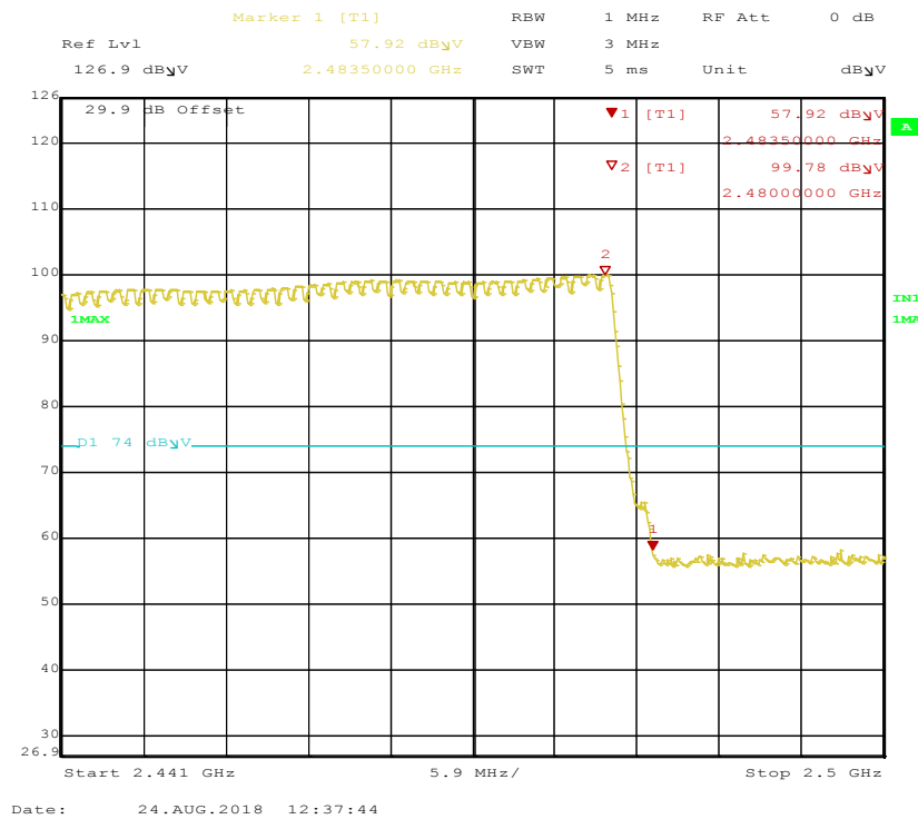
Figure 60: Radiated Emission at the 2483.5 MHz Edge for Hopping Channel at DH1 – Horizontal (Pk)
