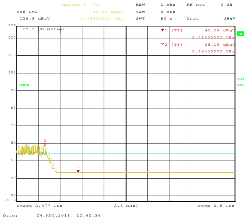
Figure 62: Radiated Emission at the 2483.5 MHz Edge for Hopping Channel at DH1 – Horizontal (Avg)
