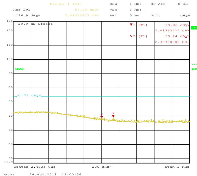
Figure 41: Radiated Emission at 2483.5 MHz, 2 MHz Span, for Channel 2480 MHz at DH1 – Vertical (Pk)
