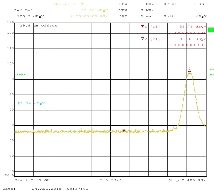
Figure 32: Radiated Emission at 2390 MHz Edge for Channel 2402 MHz at DH1 – Vertical (Pk)
