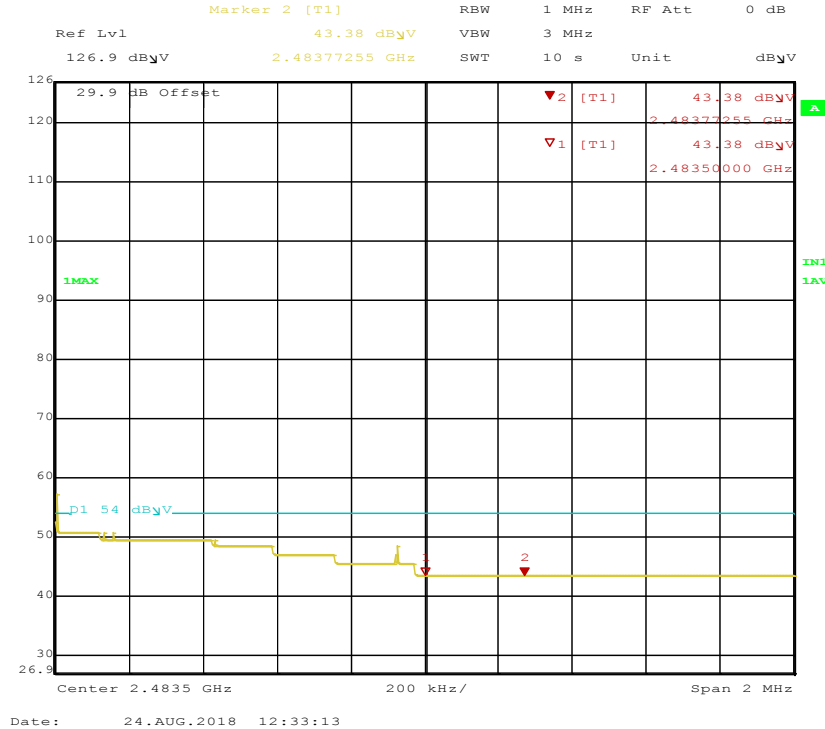
Figure 47: Radiated Emission at 2483.5 MHz, 2 MHz Span, for Channel 2480 MHz at DH1 – Horizontal (Avg)
