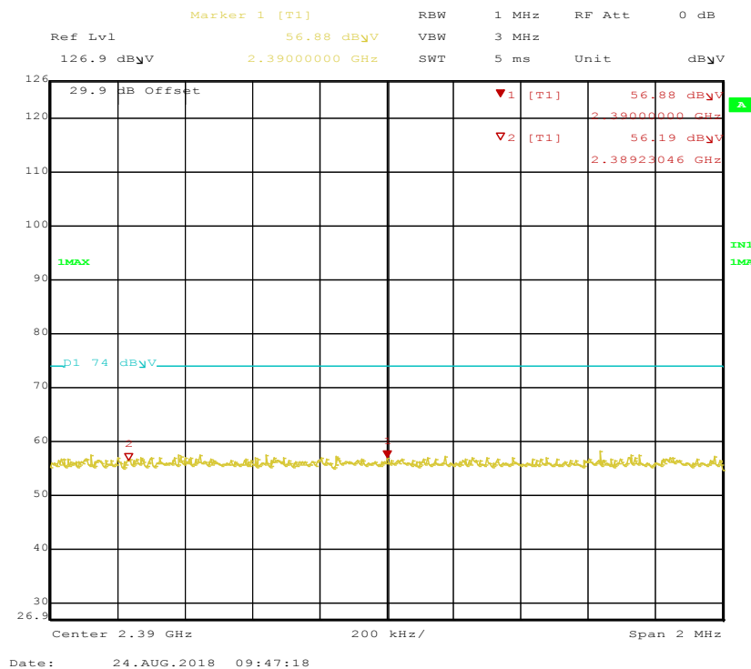
Figure 33: Radiated Emission at 2390 MHz, 2 MHz Span, for Channel 2402 MHz at DH1 – Vertical (Pk)
