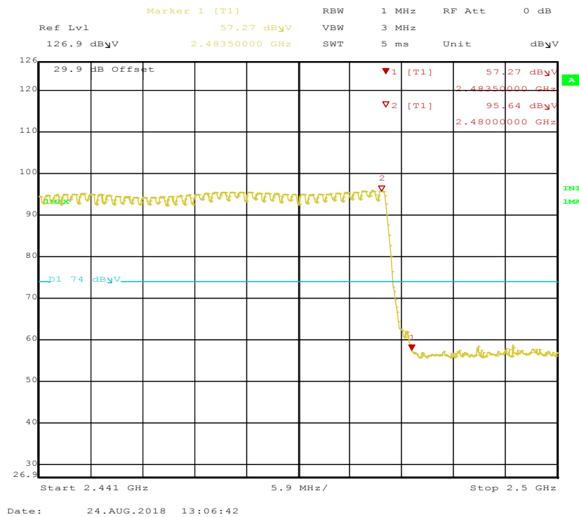
Figure 56: Radiated Emission at the 2483.5 MHz Edge for Hopping Channel at DH1 – Vertical (Pk)
