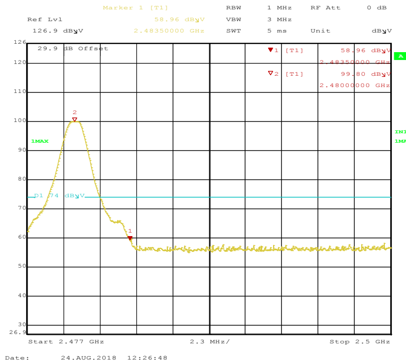
Figure 44: Radiated Emission at the 2483.5 MHz Edge for Channel 2480 MHz at DH1 – Horizontal (Pk)
