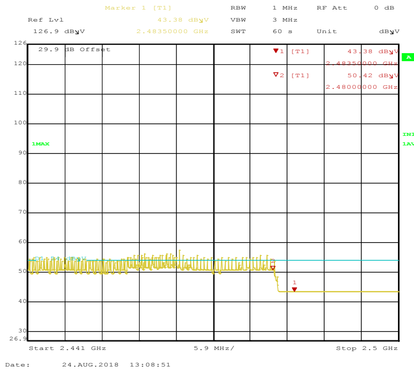
Figure 58: Radiated Emission at the 2483.5 MHz Edge for Hopping Channel at DH1 – Vertical (Avg)
