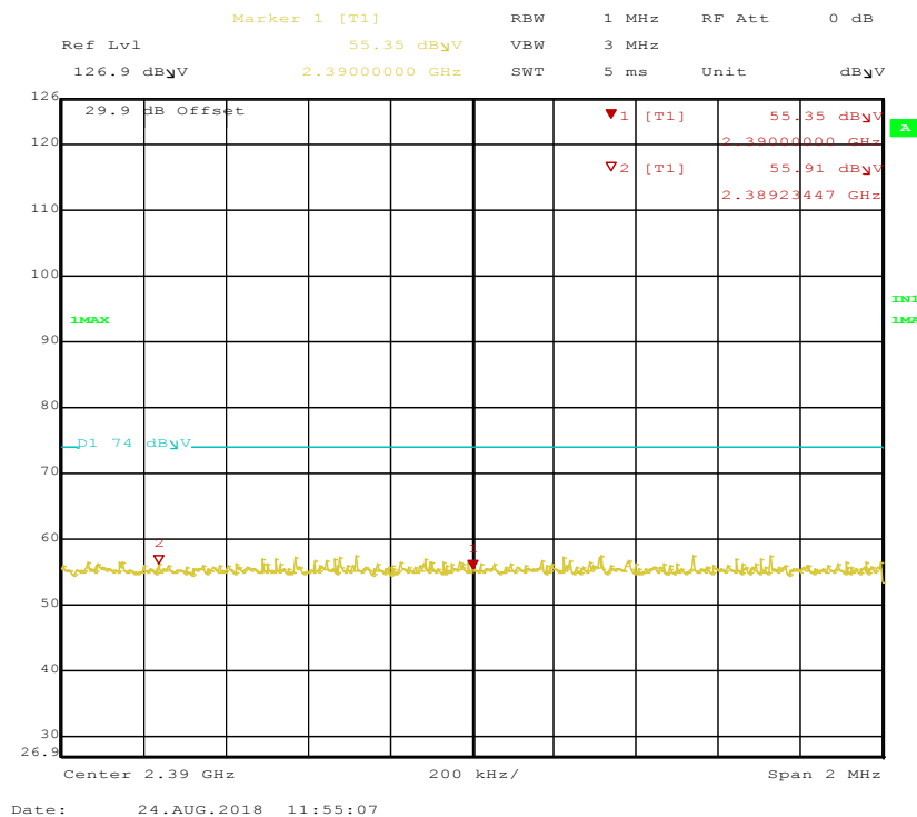
Figure 37: Radiated Emission at 2390 MHz, 2 MHz Span, for Channel 2402 MHz at DH1 – Horizontal (Pk)
