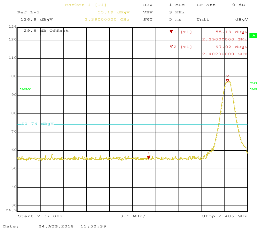
Figure 36: Radiated Emission at the 2390 MHz Edge for Channel 2402 MHz at DH1 – Horizontal (Pk)
