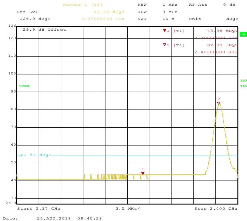
Figure 34: Radiated Emission at the 2390 MHz Edge for Channel 2402 MHz at DH1 – Vertical (Avg)
