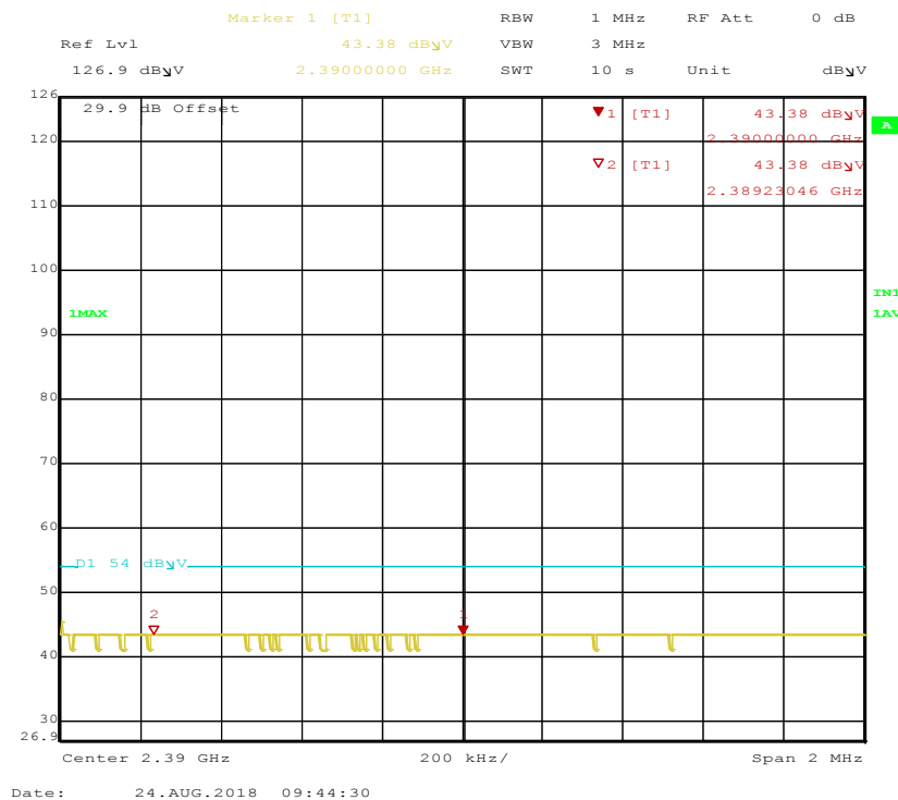
Figure 35: Radiated Emission at 2390 MHz, 2 MHz Span, for Channel 2402 MHz at DH1 – Vertical (Avg)
