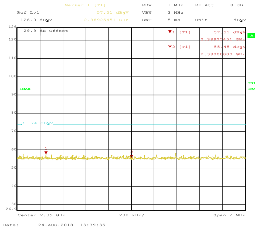
Figure 49: Radiated Emission at the 2390 MHz, 2 MHz Span, for Hopping Channel at DH1 – Vertical (Pk)
