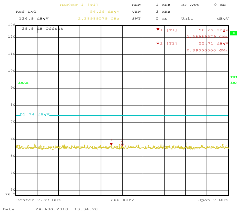
Figure 53: Radiated Emission at the 2390 MHz, 2 MHz Span, for Hopping Channel at DH1 – Horizontal (Pk)
