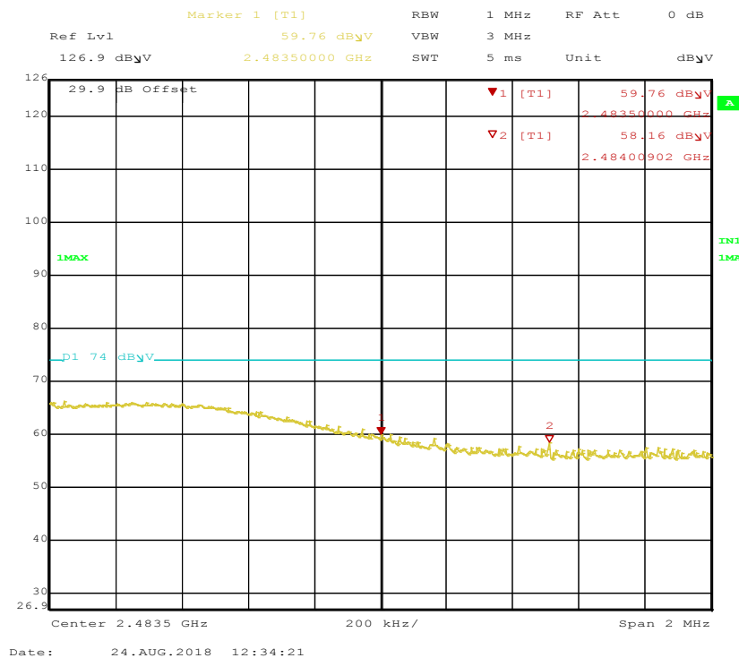
Figure 45: Radiated Emission at 2483.5 MHz, 2 MHz Span, for Channel 2480 MHz at DH1 – Horizontal (Pk)
