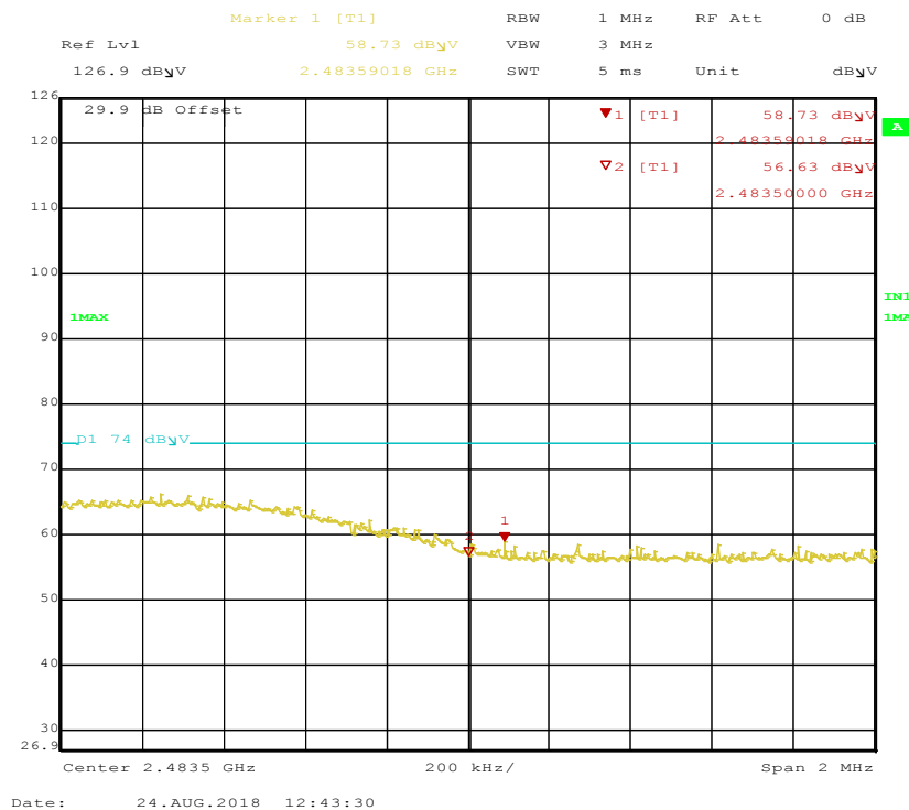
Figure 61: Radiated Emission at the 2483.5 MHz, 2 MHz Span, for Hopping Channel at DH1 – Horizontal (Pk)
