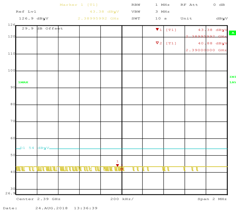
Figure 55: Radiated Emission at the 2390 MHz, 2 MHz Span, for Hopping Channel at DH1 – Horizontal (Avg)
