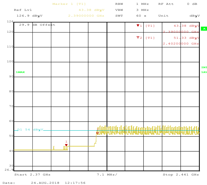
Figure 54: Radiated Emission at the 2390 MHz Edge for Hopping Channel at DH1 – Horizontal (Avg)
