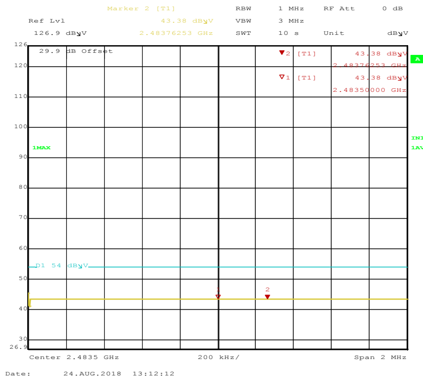
Figure 59: Radiated Emission at the 2483.5 MHz, 2 MHz Span, for Hopping Channel at DH1 – Vertical (Avg)
