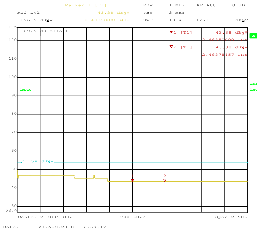
Figure 43: Radiated Emission at 2483.5 MHz, 2 MHz Span, for Channel 2480 MHz at DH1 – Vertical (Avg)
