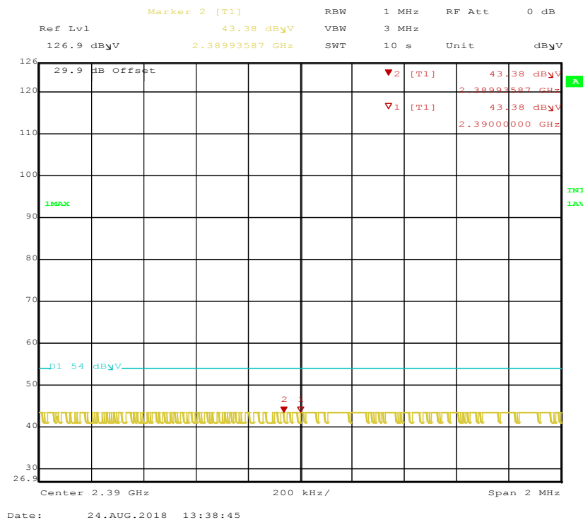
Figure 51: Radiated Emission at the 2390 MHz, 2 MHz Span, for Hopping Channel at DH1 – Vertical (Avg)
