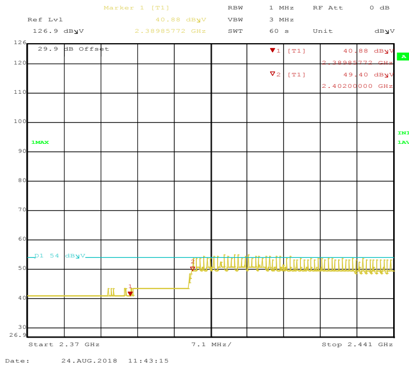
Figure 50: Radiated Emission at the 2390 MHz Edge for Hopping Channel at DH1 – Vertical (Avg)
