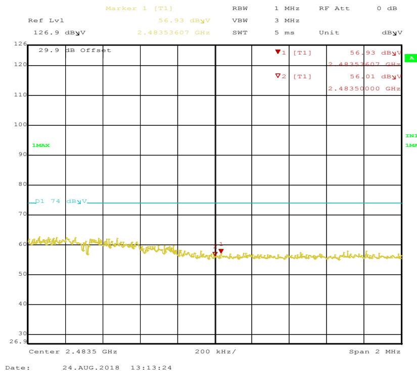
Figure 57: Radiated Emission at the 2483.5 MHz, 2 MHz Span, for Hopping Channel at DH1 – Vertical (Pk)
