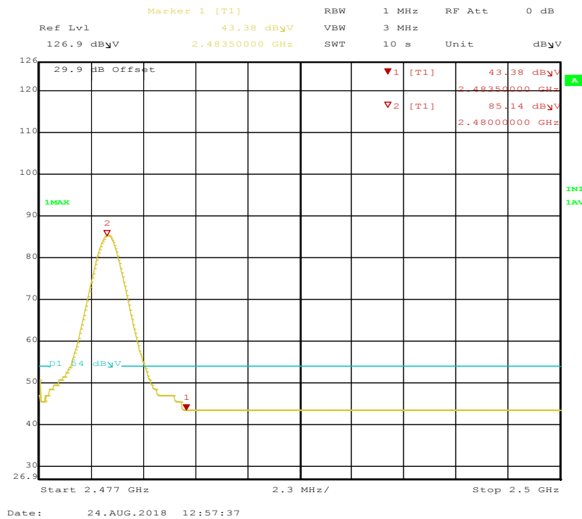
Figure 42: Radiated Emission at the 2483.5 MHz Edge for Channel 2480 MHz at DH1 – Vertical (Avg)
