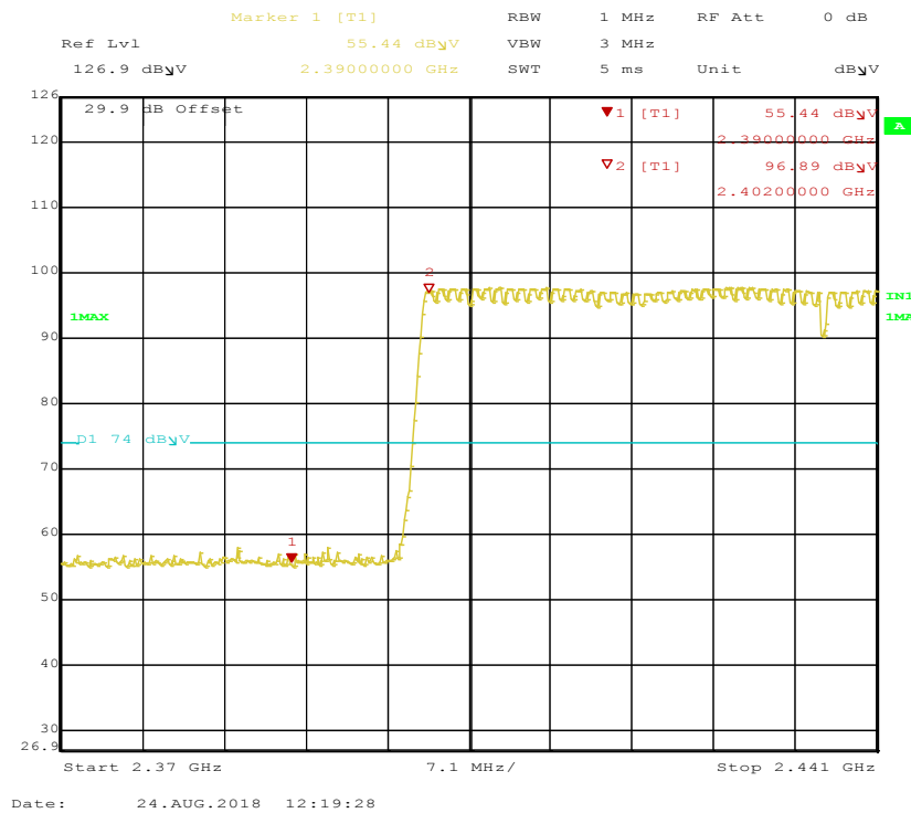
Figure 52: Radiated Emission at the 2390 MHz Edge for Hopping Channel at DH1 – Horizontal (Pk)
