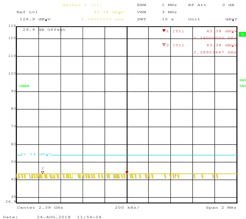
Figure 39: Radiated Emission at 2390 MHz, 2 MHz Span, for Channel 2402 MHz at DH1 – Horizontal (Avg)
