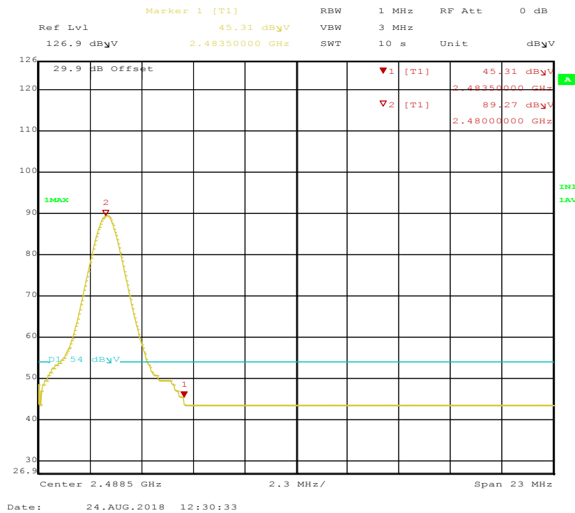
Figure 46: Radiated Emission at the 2483.5 MHz Edge for Channel 2480 MHz at DH1 – Horizontal (Avg)
