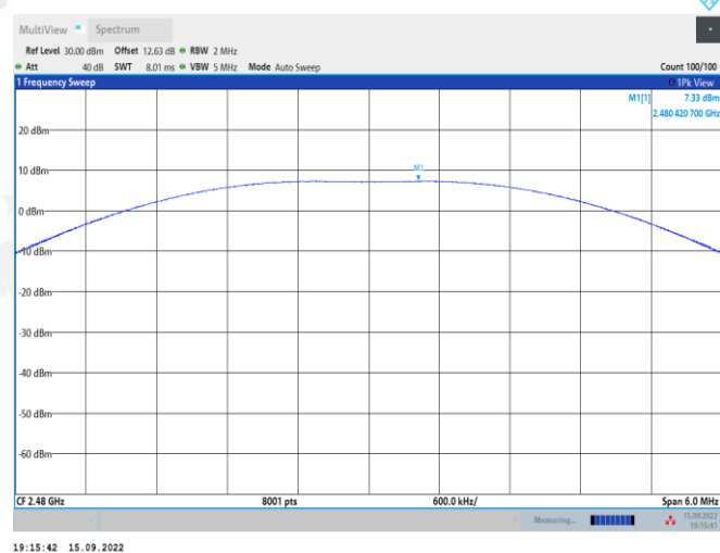
GFSK 2M_Ant1_2480
