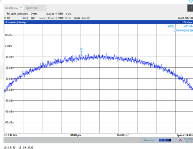
GFSK 2M_Ant1_2480
