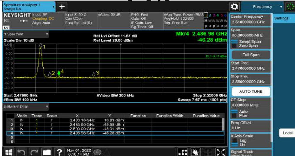
DH5_Ant1_High_2480
