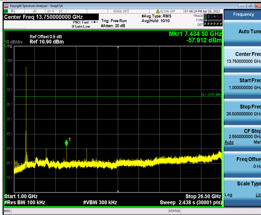
2DH5_Ant1_2402_0~Reference
