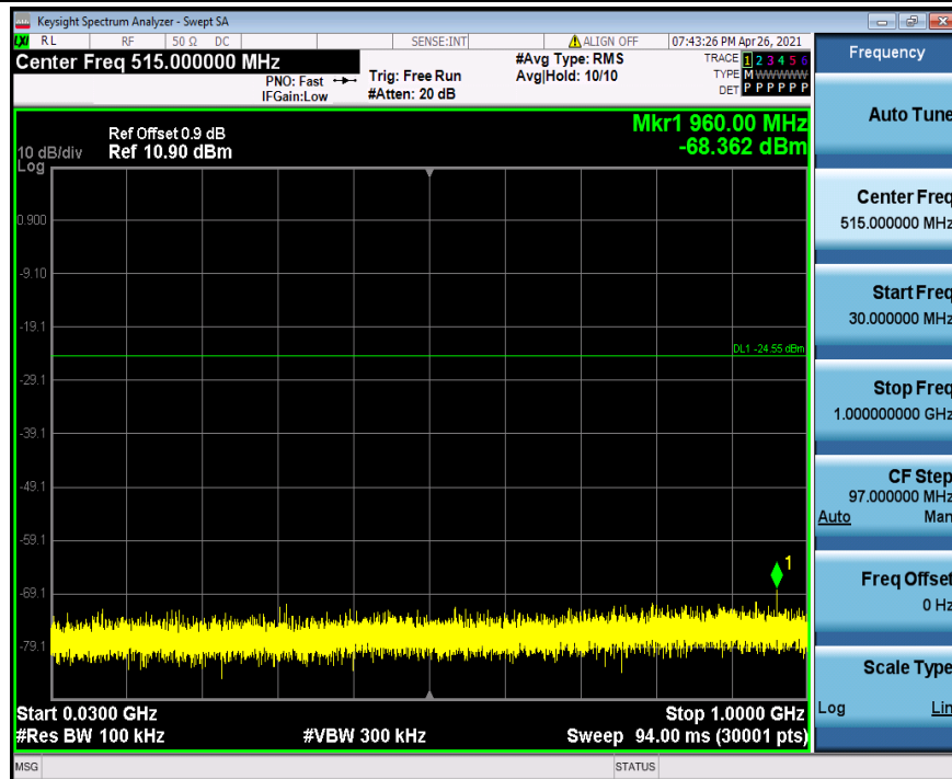
DH5_Ant1_2402_30-1000
