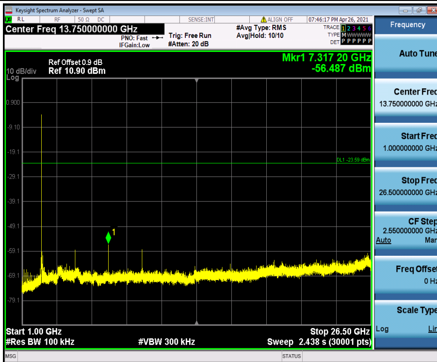
DH5_Ant1_2441_1000~26500
