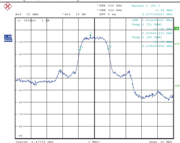
HCH (99% bandwidth)
