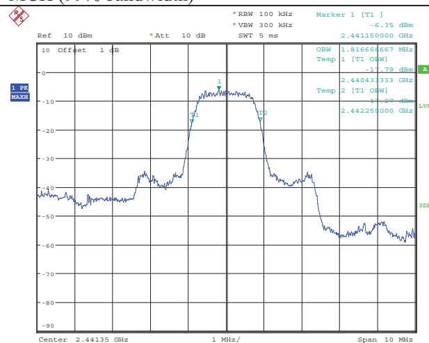
MCH (99% bandwidth)
