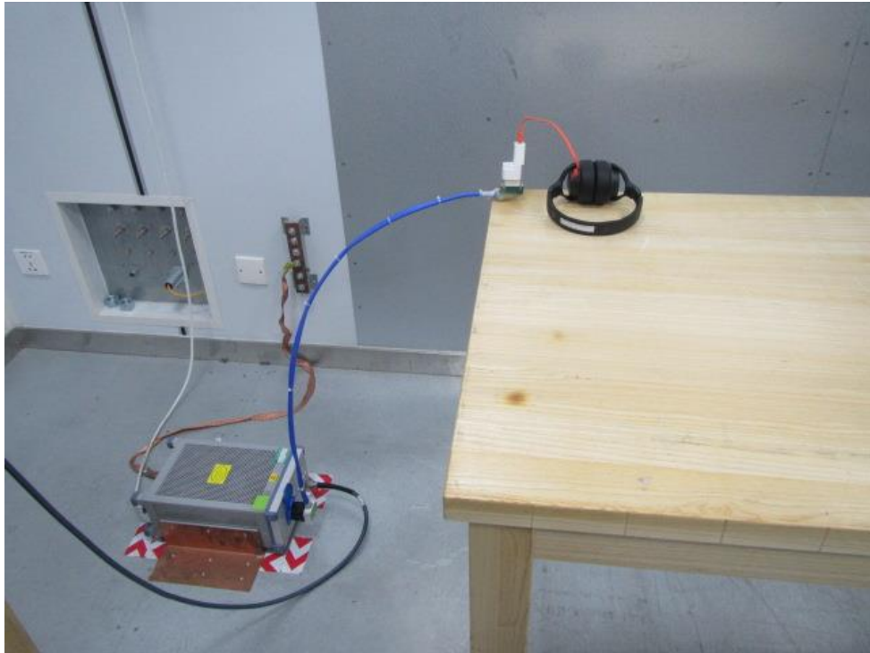
Conducted Disturbance
