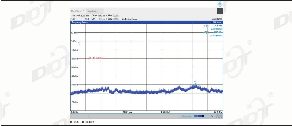
3DH5 Ant1_2402_0~Reference
