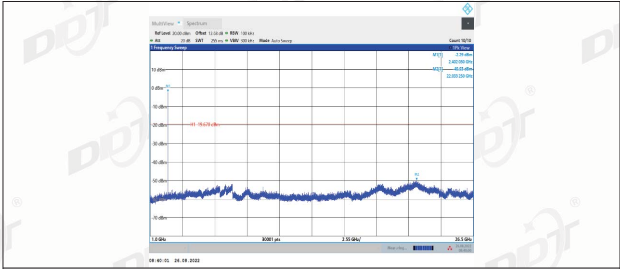
3DH5_Ant1_2441_0~Reference
