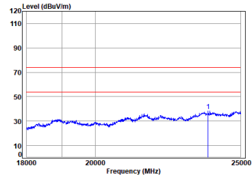
Right earbuds 2.4G SRD_1M_TX_CH_19_Vertical
