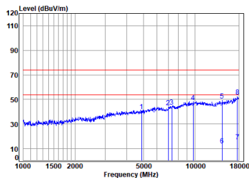
Right earbuds 2.4G SRD_1M_TX_CH_19_Vertical
