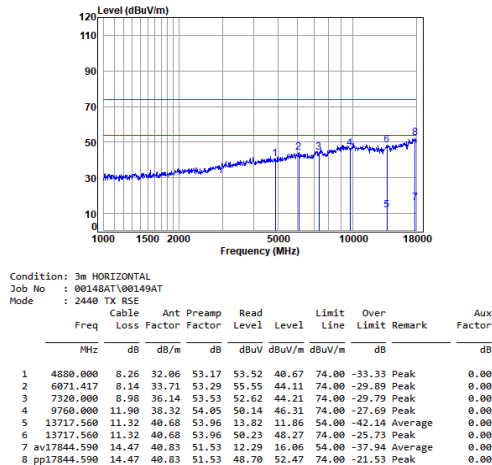
Left earbuds 2.4G SRD_1M_TX_CH_19_Horizontal
