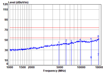
Left earbuds 2.4G SRD_2M_TX_CH_19_Horizontal
