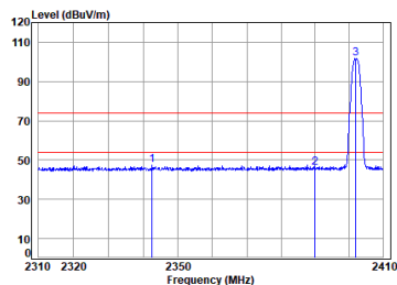
Left earbuds 2.4G SRD_1M_TX_CH_00_Horizontal
