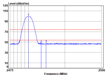
Left earbuds 2.4G SRD_1M_TX_CH_39_Horizontal
