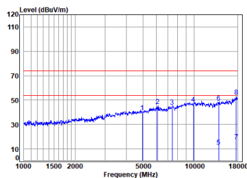
Right earbuds 2.4G SRD_2M_TX_CH_38_Horizontal
