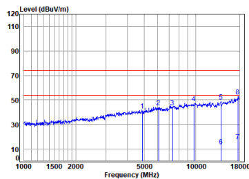
Right earbuds 2.4G SRD_2M_TX_CH_19_Horizontal
