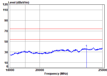
Left earbuds 2.4G SRD_1M_TX_CH_19_Horizontal
