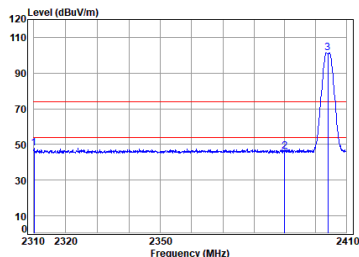
Left earbuds 2.4G SRD_2M_TX_CH_01_Horizontal
