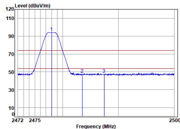
Left earbuds 2.4G SRD_2M_TX_CH_38_Vertical
