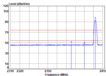
Left earbuds 2.4G SRD_1M_TX_CH_00_Vertical
