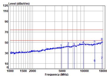
Right earbuds 2.4G SRD_1M_TX_CH_19_Horizontal
