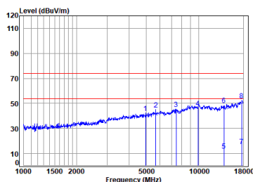
Right earbuds 2.4G SRD_1M_TX_CH_39_Horizontal
