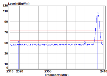
Right earbuds 2.4G SRD_2M_TX_CH_01_Horizontal
