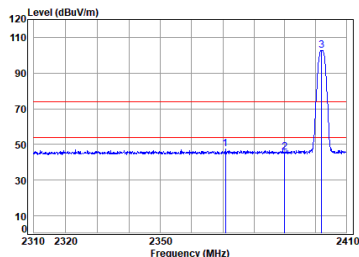
Right earbuds 2.4G SRD_1M_TX_CH_00_Horizontal
