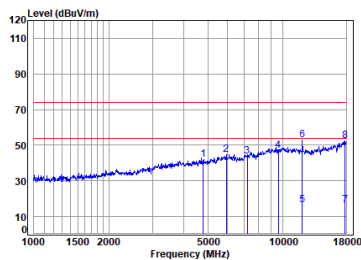
Right earbuds 2.4G SRD_1M_TX_CH_00_Vertical
