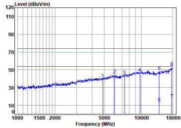
Left earbuds 2.4G SRD_2M_TX_CH_19_Vertical
