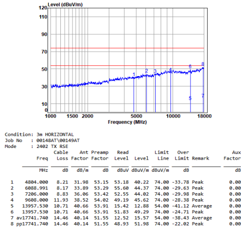
Left earbuds 2.4G SRD_1M_TX_CH_00_Horizontal
