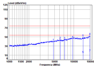
Left earbuds 2.4G SRD_2M_TX_CH_01_Vertical
