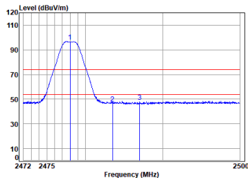
Right earbuds 2.4G SRD_2M_TX_CH_38_Vertical
