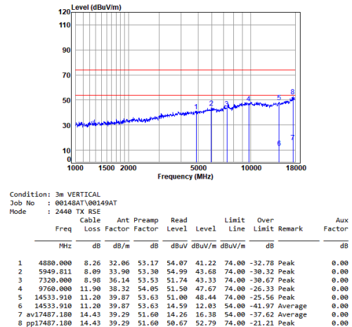
Left earbuds 2.4G SRD_1M_TX_CH_19_Vertical
