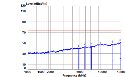
Left earbuds 2.4G SRD_2M_TX_CH_01_Horizontal
