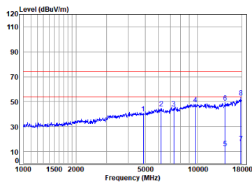
Right earbuds 2.4G SRD_2M_TX_CH_19_Vertical
