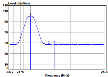
Left earbuds 2.4G SRD_2M_TX_CH_38_Horizontal
