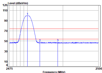
Right earbuds 2.4G SRD_1M_TX_CH_39_Horizontal
