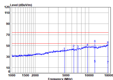
Right earbuds 2.4G SRD_2M_TX_CH_01_Vertical
