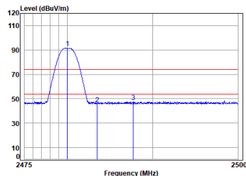
Left earbuds 2.4G SRD_1M_TX_CH_39_Vertical
