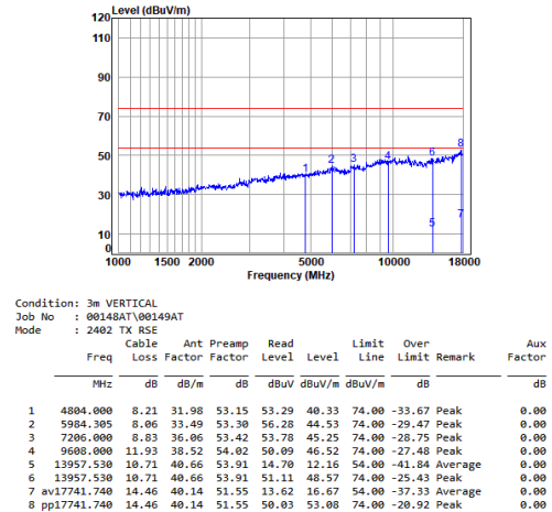
Left earbuds 2.4G SRD_1M_TX_CH_00_Vertical
