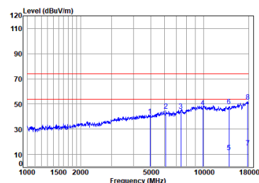
Right earbuds 2.4G SRD_1M_TX_CH_39_Vertical
