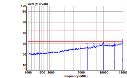
Left earbuds 2.4G SRD_1M_TX_CH_39_Horizontal
