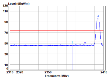
Right earbuds 2.4G SRD_2M_TX_CH_01_Vertical
