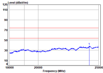
Right earbuds 2.4G SRD_1M_TX_CH_19_Horizontal
