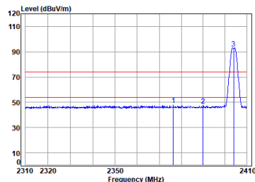
Left earbuds 2.4G SRD_2M_TX_CH_01_Vertical
