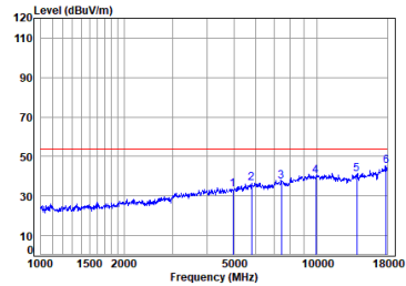
Left earbuds BLE_1M_TX_CH_39_Vertical-Avg
