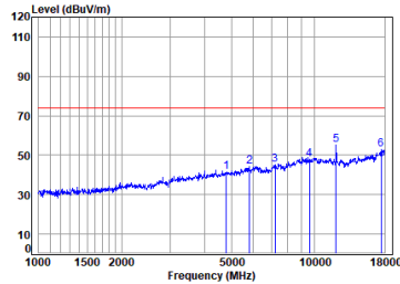
Right earbuds BLE_1M_TX_CH_00_Horizontal-Peak
