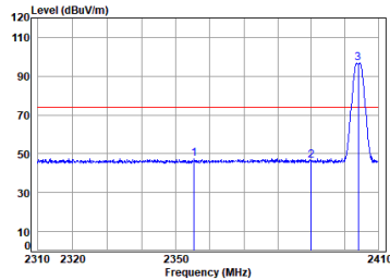
Left earbuds BLE_2M_TX_CH_01_Vertical-Peak
