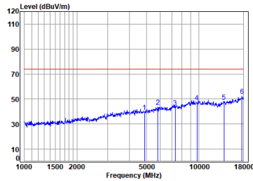
Left earbuds BLE_2M_TX_CH_19_Vertical-Peak
