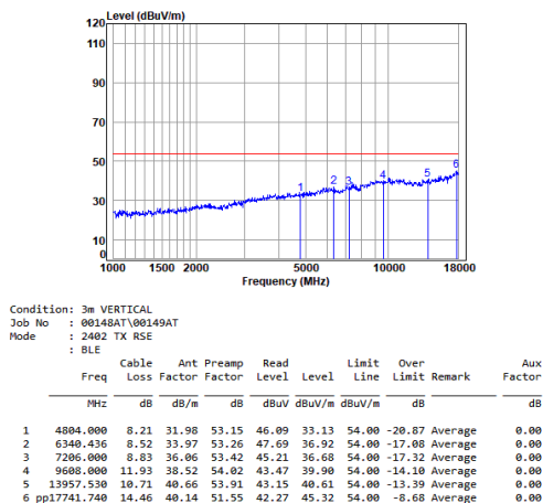
Left earbuds BLE_1M_TX_CH_00_Vertical-Avg
