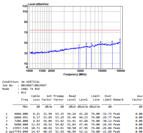
Left earbuds BLE_1M_TX_CH_00_Vertical-Peak
