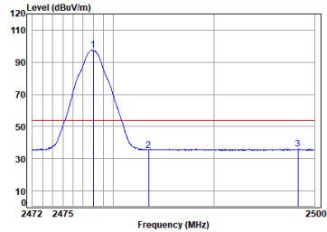
Right earbuds BLE_2M_TX_CH_38_Horizontal-Avg
