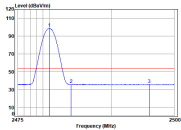
Left earbuds BLE_1M_TX_CH_39_Horizontal-Avg
