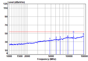
Right earbuds BLE_1M_TX_CH_00_Vertical-Avg
