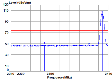
Right earbuds BLE_2M_TX_CH_01_Horizontal-Peak
