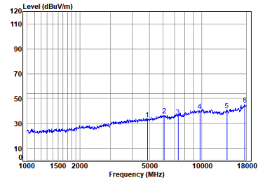
Left earbuds BLE_1M_TX_CH_19_Vertical-Avg
