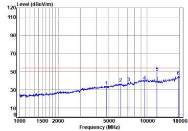
Right earbuds BLE_1M_TX_CH_00_Horizontal-Avg
