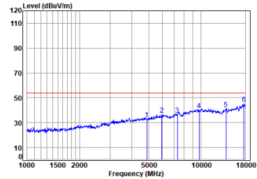
Left earbuds BLE_1M_TX_CH_19_Horizontal-Avg
