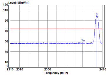
Right earbuds BLE_2M_TX_CH_01_Vertical-Peak
