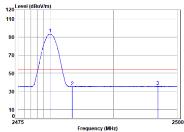
Left earbuds BLE_1M_TX_CH_39_Vertical-Avg
