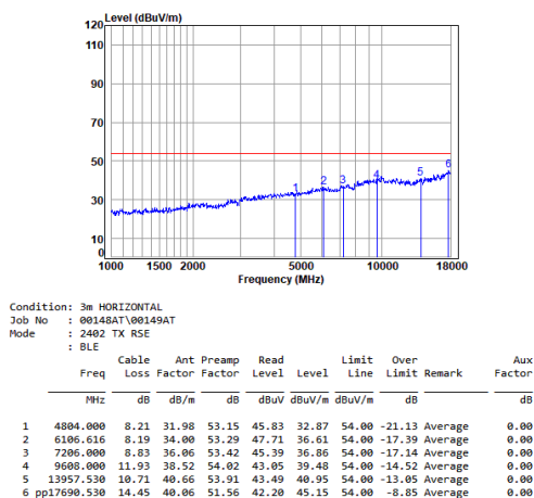
Left earbuds BLE_1M_TX_CH_00_Horizontal-Avg
