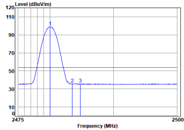
Right earbuds BLE_1M_TX_CH_39_Horizontal-Avg
