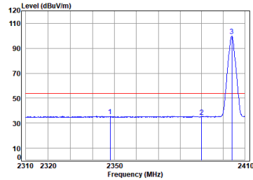
Left earbuds BLE_2M_TX_CH_01_Horizontal-Avg
