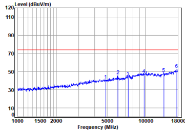
Left earbuds BLE_1M_TX_CH_19_Horizontal-Peak
