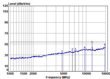
Right earbuds BLE_2M_TX_CH_01_Horizontal-Avg
