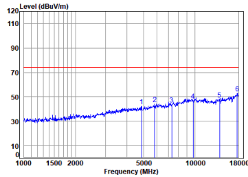
Right earbuds BLE_2M_TX_CH_19_Vertical-Peak
