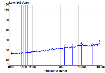
Left earbuds BLE_2M_TX_CH_19_Vertical-Avg
