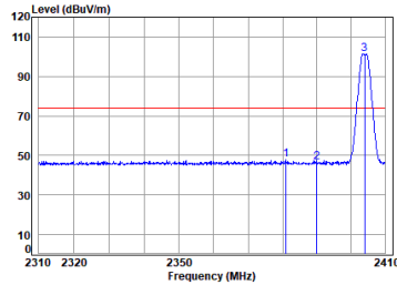
Left earbuds BLE_2M_TX_CH_01_Horizontal-Peak
