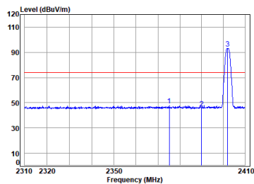
Left earbuds BLE_1M_TX_CH_00_Vertical-Peak
