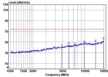
Left earbuds BLE_2M_TX_CH_19_Horizontal-Peak
