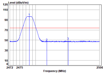
Right earbuds BLE_2M_TX_CH_38_Vertical-Peak
