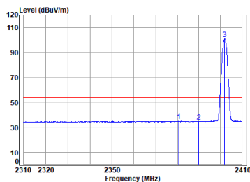
Left earbuds BLE_1M_TX_CH_00_Horizontal-Avg
