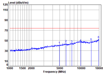
Right earbuds BLE_1M_TX_CH_39_Vertical-Peak
