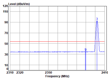
Left earbuds BLE_1M_TX_CH_00_Vertical-Avg
