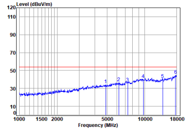
Left earbuds BLE_2M_TX_CH_19_Horizontal-Avg
