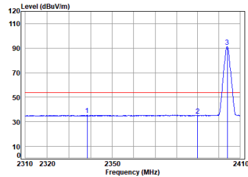
Left earbuds BLE_2M_TX_CH_01_Vertical-Avg
