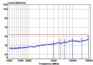
Left earbuds BLE_2M_TX_CH_38_Vertical-Avg
