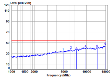
Right earbuds BLE_1M_TX_CH_19_Horizontal-Avg
