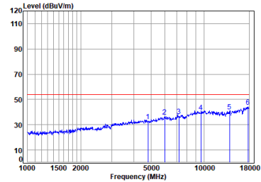
Left earbuds BLE_2M_TX_CH_01_Horizontal-Avg
