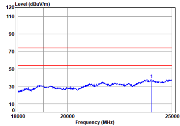
Left earbuds BLE_1M_TX_CH_19_Vertical-Peak
