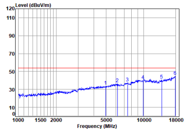
Left earbuds BLE_2M_TX_CH_38_Horizontal-Avg
