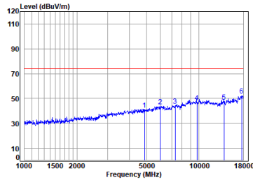
Left earbuds BLE_1M_TX_CH_19_Vertical-Peak
