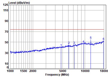
Right earbuds BLE_1M_TX_CH_00_Vertical-Peak
