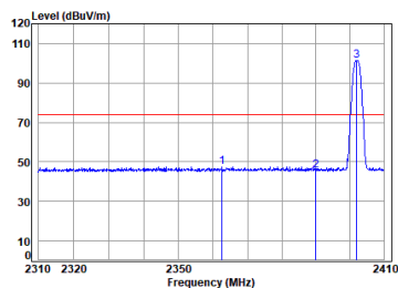
Left earbuds BLE_1M_TX_CH_00_Horizontal-Peak
