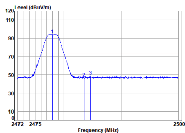
Left earbuds BLE_2M_TX_CH_38_Vertical-Peak
