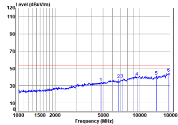
Left earbuds BLE_2M_TX_CH_01_Vertical-Avg
