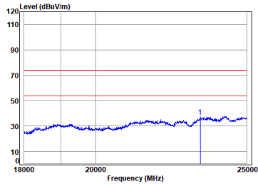
Right earbuds BLE_1M_TX_CH_19_Horizontal-Peak
