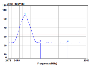
Left earbuds BLE_2M_TX_CH_38_Horizontal-Avg
