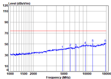
Right earbuds BLE_2M_TX_CH_01_Vertical-Peak
