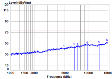
Right earbuds BLE_2M_TX_CH_19_Horizontal-Peak
