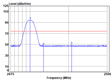
Left earbuds BLE_1M_TX_CH_39_Vertical-Peak
