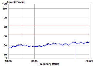
Left earbuds BLE_1M_TX_CH_19_Horizontal-Peak
