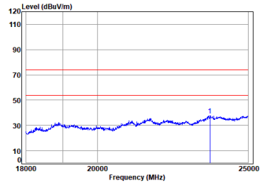
Right earbuds BLE_1M_TX_CH_19_Vertical-Peak
