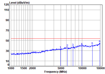
Right earbuds BLE_1M_TX_CH_39_Vertical-Avg
