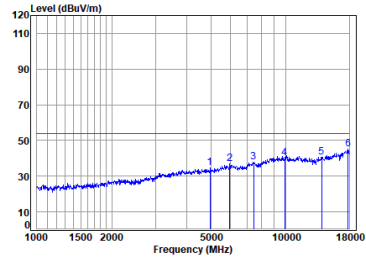
Left earbuds BLE_1M_TX_CH_39_Horizontal-Avg
