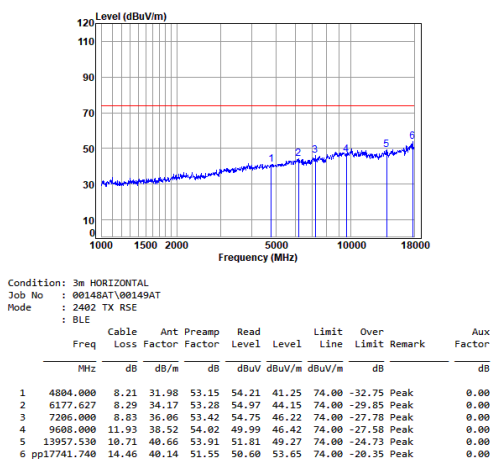
Left earbuds BLE_1M_TX_CH_00_Horizontal-Peak
