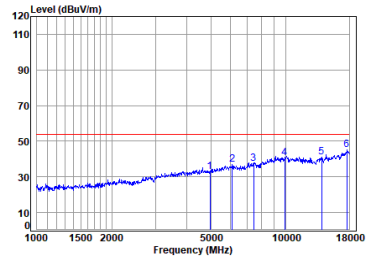
Right earbuds BLE_2M_TX_CH_38_Vertical-Avg
