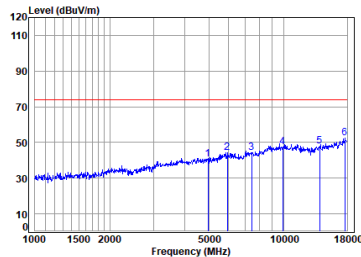
Left earbuds BLE_2M_TX_CH_38_Horizontal-Peak
