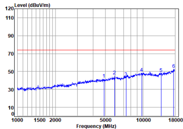
Right earbuds BLE_1M_TX_CH_19_Horizontal-Peak
