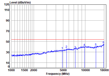
Right earbuds BLE_2M_TX_CH_19_Horizontal-Avg
