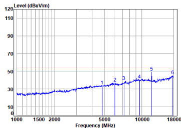
Right earbuds BLE_2M_TX_CH_01_Vertical-Avg
