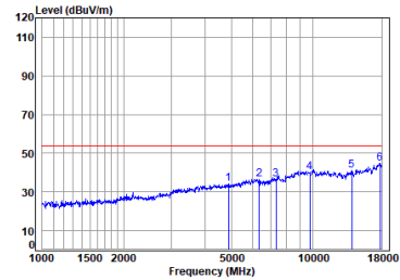
Right earbuds BLE_2M_TX_CH_19_Vertical-Avg
