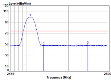
Left earbuds BLE_1M_TX_CH_39_Horizontal-Peak
