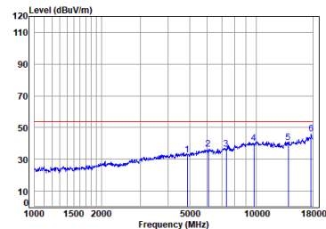
Right earbuds BLE_1M_TX_CH_19_Vertical-Avg
