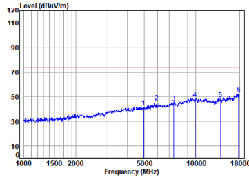
Right earbuds BLE_1M_TX_CH_39_Horizontal-Peak
