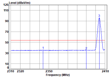
Right earbuds BLE_2M_TX_CH_01_Vertical-Avg
