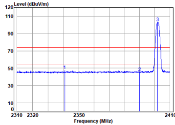
Right earbuds BT_DH5_TX_CH_00_Horizontal
