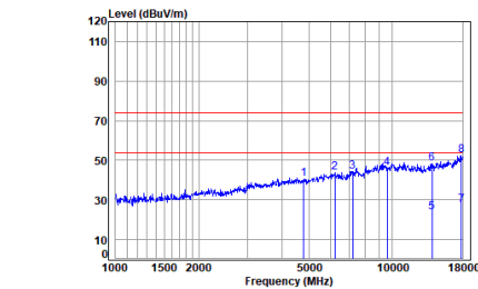
Left earbuds BT_DH5_TX_CH_00_Horizontal
