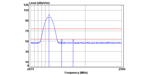
Left earbuds BT_DH5_TX_CH_78_Vertical
