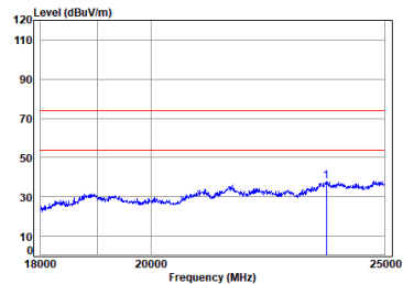
Left earbuds BT_DH5_TX_CH_39_Vertical
