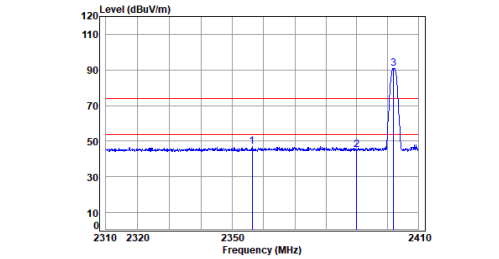
Left earbuds BT_DH5_TX_CH_00_Vertical
