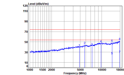
Left earbuds BT_DH5_TX_CH_39_Horizontal
