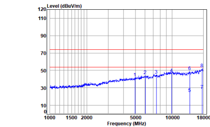
Right earbuds BT_DH5_TX_CH_78_Horizontal
