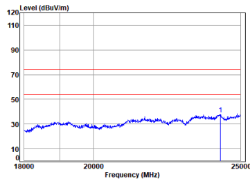
Left earbuds BT_DH5_TX_CH_39_Horizontal
