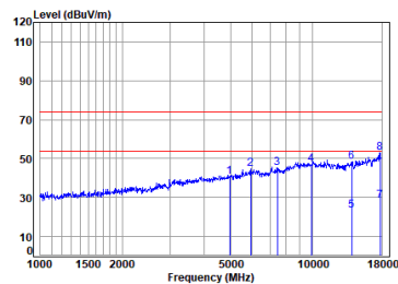
Left earbuds BT_DH5_TX_CH_78_Vertical
