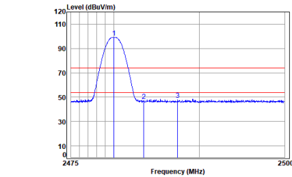
Left earbuds BT_DH5_TX_CH_78_Horizontal
