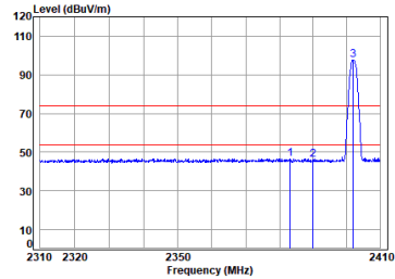
Right earbuds BT_DH5_TX_CH_00_Vertical
