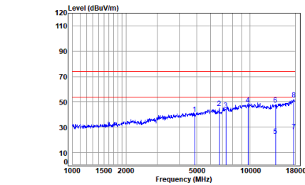
Right earbuds BT_DH5_TX_CH_39_Horizontal
