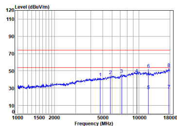
Right earbuds BT_DH5_TX_CH_00_Vertical
