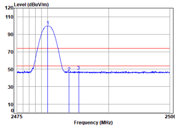
Right earbuds BT_DH5_TX_CH_78_Horizontal
