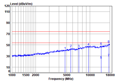
Left earbuds BT_DH5_TX_CH_00_Vertical
