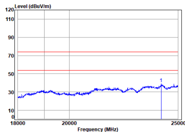
Right earbuds BT_DH5_TX_CH_39_Horizontal
