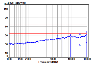
Right earbuds BT_DH5_TX_CH_39_Vertical
