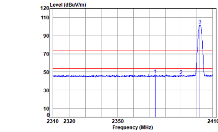
Left earbuds BT_DH5_TX_CH_00_Horizontal
