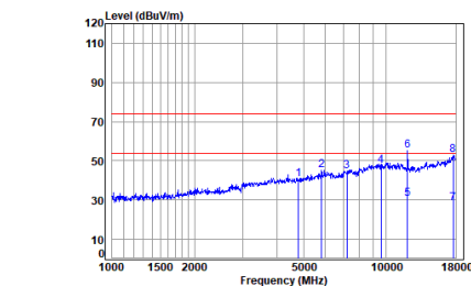
Right earbuds BT_DH5_TX_CH_00_Horizontal
