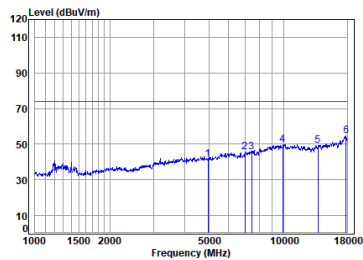
BLE_1M_TX_CH_39_Vertical-Peak
