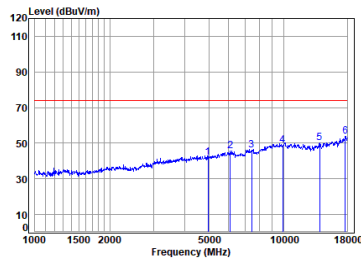
BLE_2M_TX_CH_38_Horizontal-Peak
