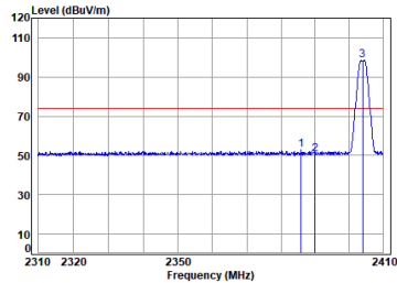
BLE_2M_TX_CH_01_Vertical-Peak
