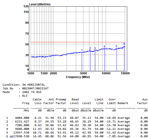
BLE_1M_TX_CH_00_Horizontal-Avg
