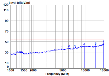
BLE_1M_TX_CH_19_Vertical-Avg
