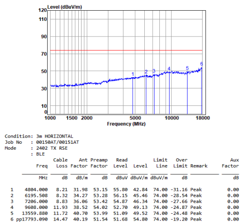
BLE_1M_TX_CH_00_Horizontal-Peak
