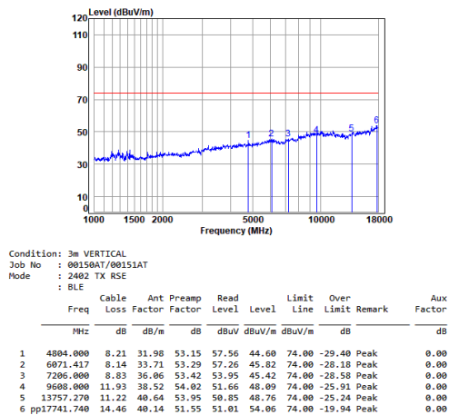
BLE_1M_TX_CH_00_Vertical-Peak
