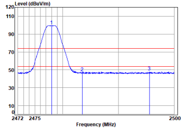
2.4G SRD_2M_TX_CH_38_Vertical
