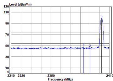
2.4G SRD_1M_TX_CH_00_Vertical
