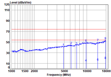
2.4G SRD_2M_TX_CH_19_Vertical
