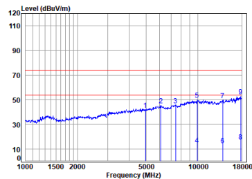
2.4G SRD_1M_TX_CH_39_Vertical
