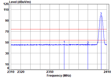
2.4G SRD_2M_TX_CH_01_Vertical
