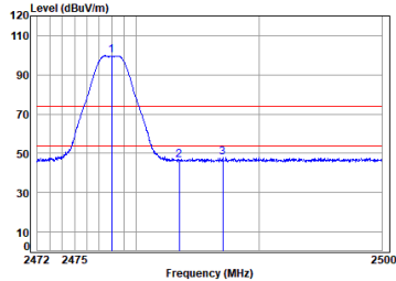
2.4G SRD_2M_TX_CH_38_Horizontal
