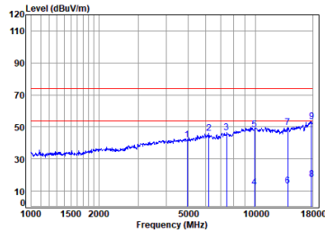
2.4G SRD_2M_TX_CH_38_Horizontal
