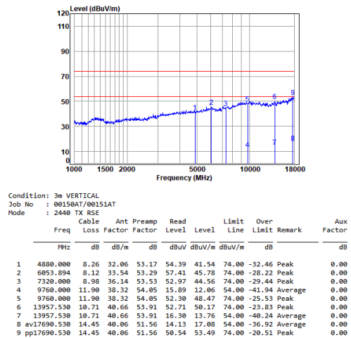
2.4G SRD_1M_TX_CH_19_Vertical
