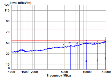
2.4G SRD_2M_TX_CH_38_Vertical
