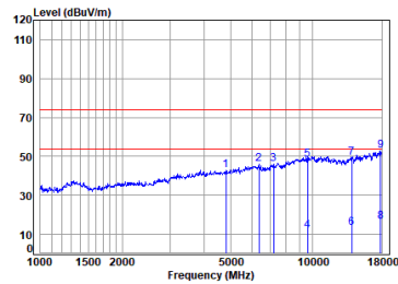
2.4G SRD_2M_TX_CH_01_Vertical
