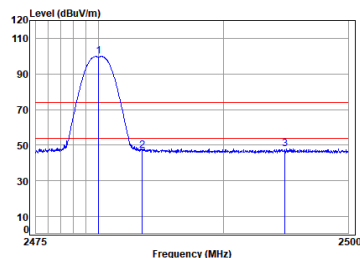
2.4G SRD_1M_TX_CH_39_Vertical
