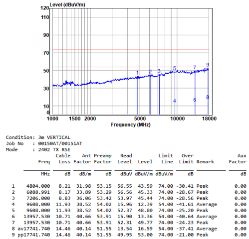
2.4G SRD_1M_TX_CH_00_Vertical
