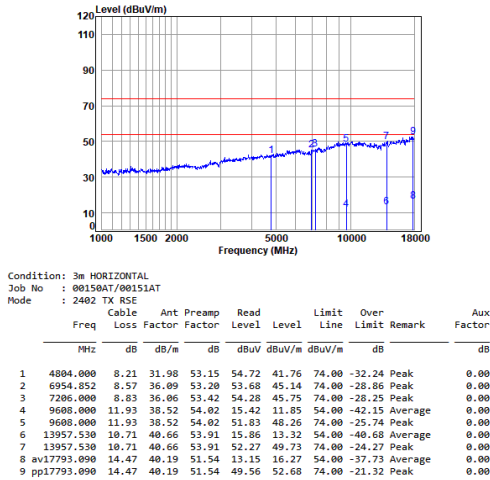
2.4G SRD_1M_TX_CH_00_Horizontal
