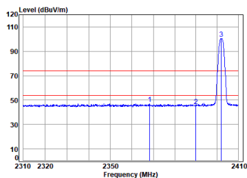
2.4G SRD_1M_TX_CH_00_Horizontal
