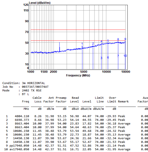
BT_DH5_TX_CH_00_Horizontal
