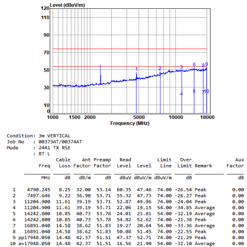
BT_DH5_TX_CH_39_Vertical
