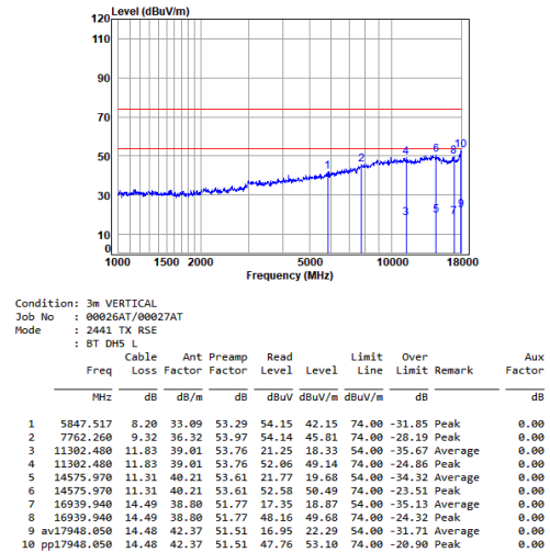
BT_DH5_TX_CH_39_Vertical
