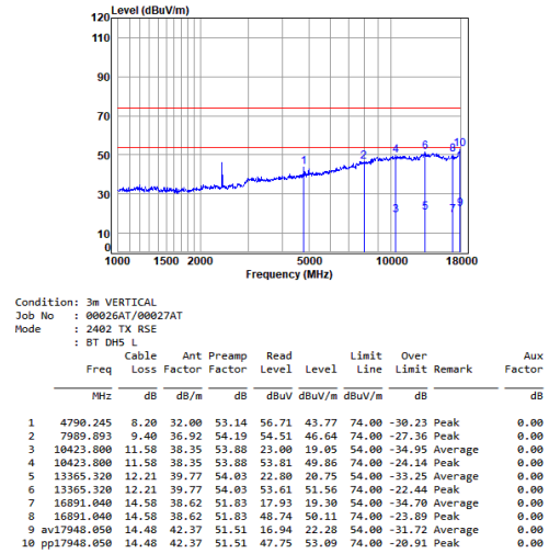
BT_DH5_TX_CH_00_Vertical
