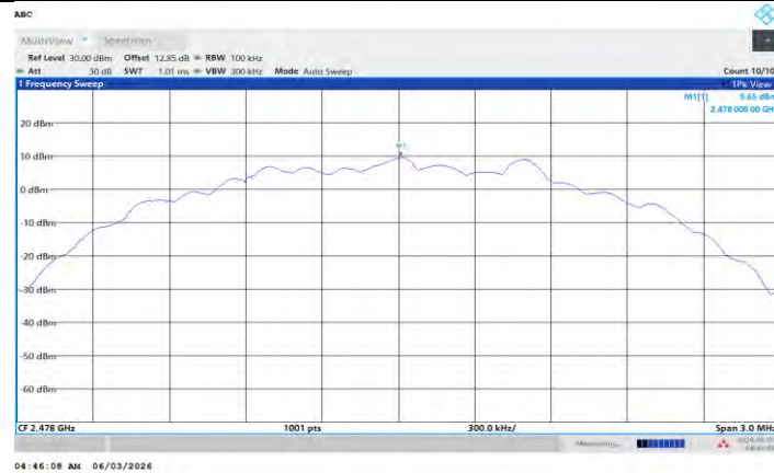
BLE_2M_Ant L_2478_0-Reference
