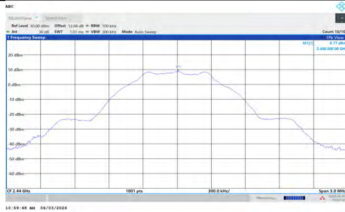
BLE_1M_Ant R_2440_0-Reference
