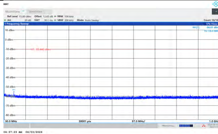
BLE_2M_Ant L_2404_30-1000
