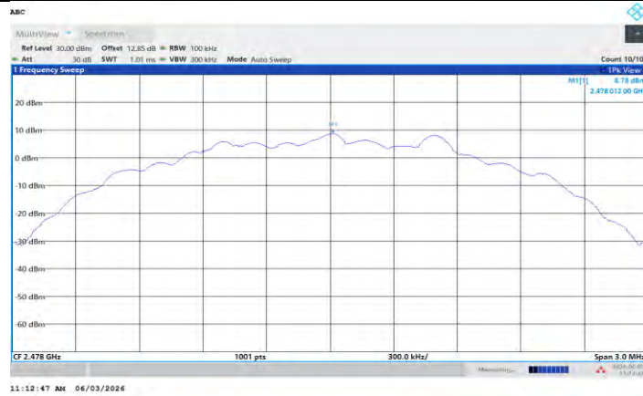
BLE_2M_Ant R_2478_0-Reference
