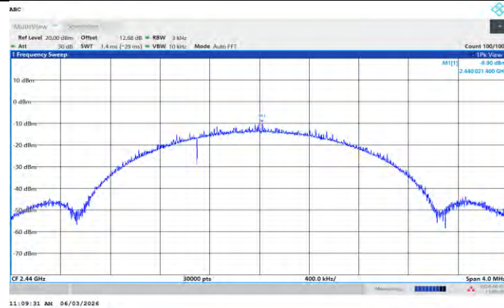
BLE_2M_Ant R_2440
