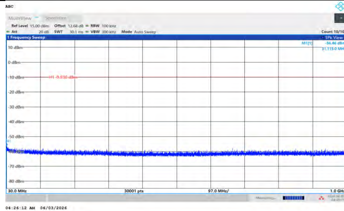
BLE_1M_Ant L_2440_30-1000
