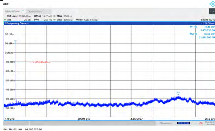
BLE_2M_Ant L_2404_1000-26500
