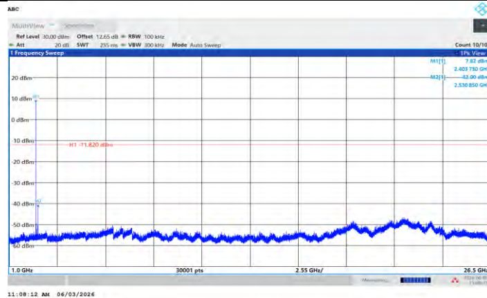
BLE_2M_Ant R_2404_1000-26500
