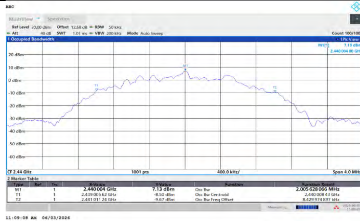
BLE_2M_Ant R_2440
