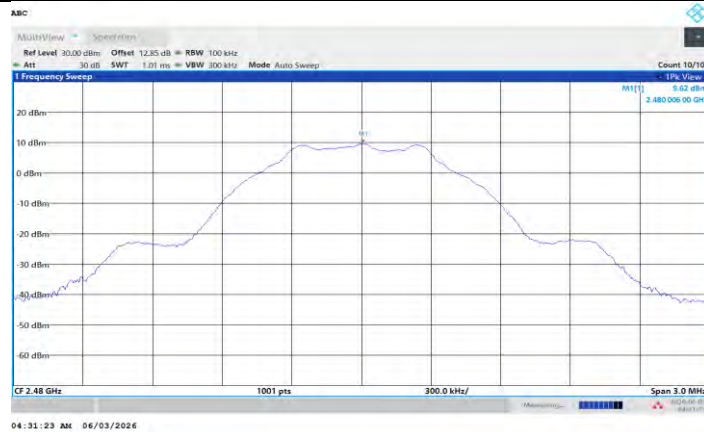
BLE_1M_Ant L_2480_0-Reference
