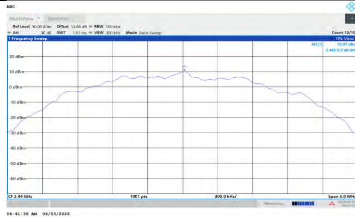
BLE_2M_Ant L_2440_0-Reference
