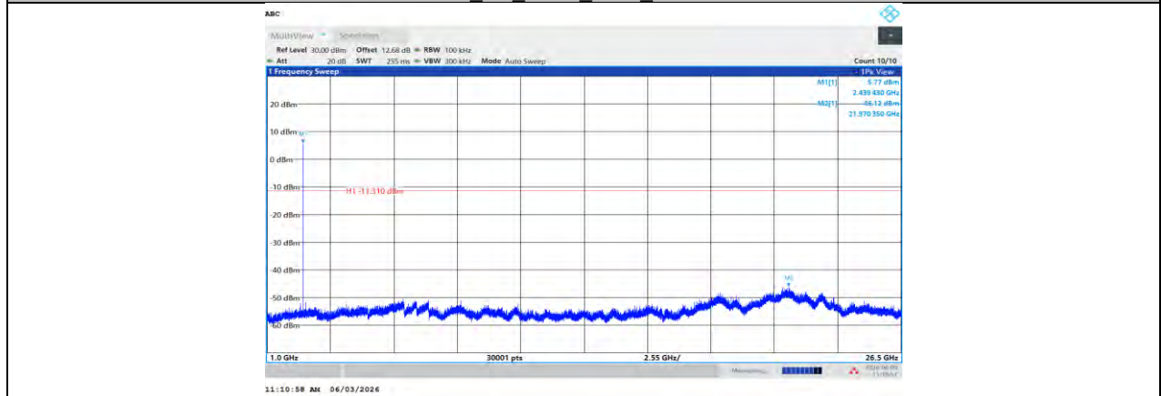
BLE_2M_Ant R_2440_1000-26500
