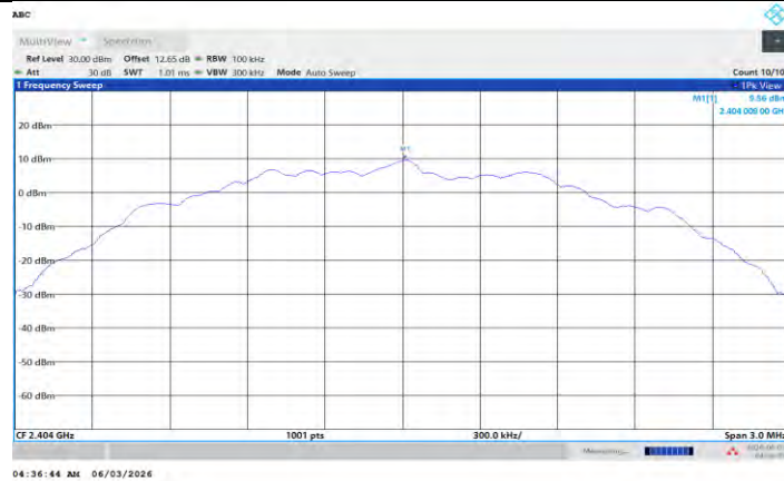
BLE_2M_Ant L_2404_0-Reference
