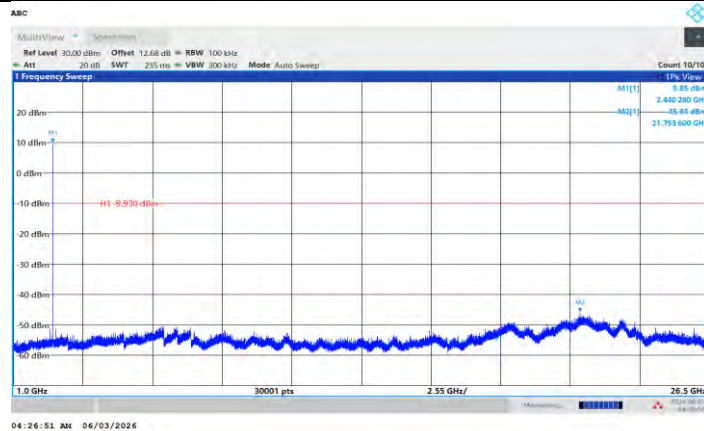
BLE_1M_Ant L_2440_1000-26500
