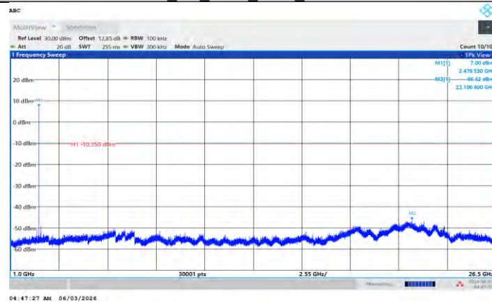
BLE_2M_Ant L_2478_1000-26500
