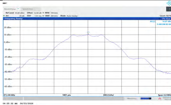
BLE_1M_Ant L_2440_0-Reference
