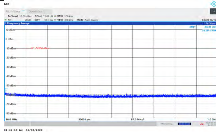
BLE_2M_Ant L_2440_30-1000
