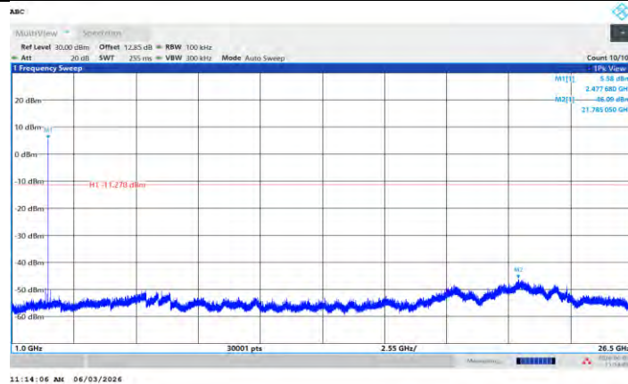
BLE_2M_Ant R_2478_1000-26500
