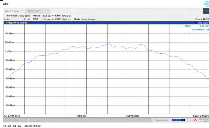
BLE_2M_Ant R_2404_0-Reference
