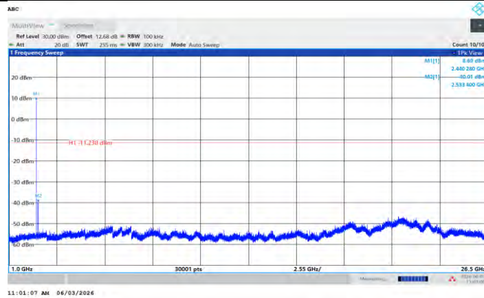
BLE_1M_Ant R_2440_1000-26500
