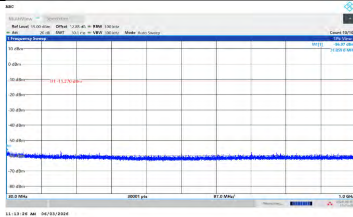
BLE_2M_Ant R_2478_30-1000
