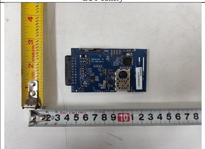
EUT main PCBA Bottom View
