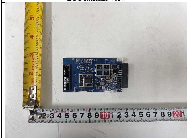
EUT main PCBA Top View
