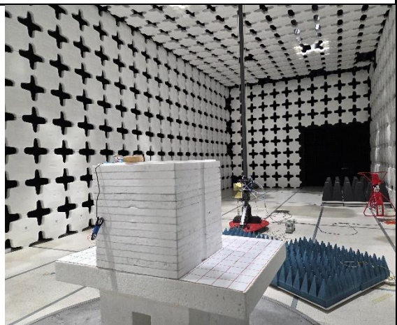
Radiated Emission Test above 1GHz Rear View
