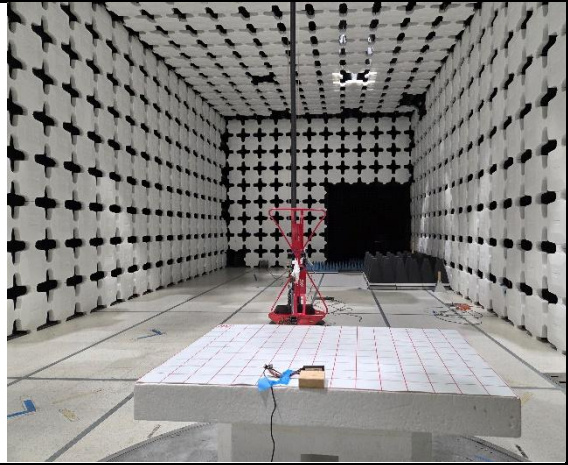
Radiated Emission Test below 1GHz Rear View
