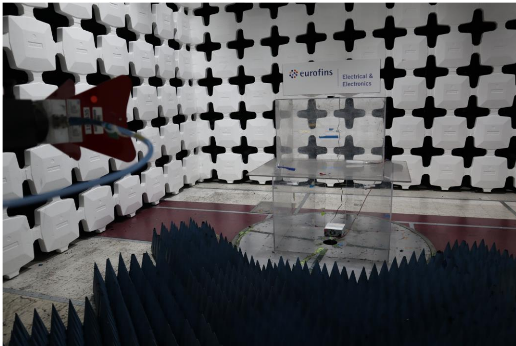
Figure 10. Radiated Spurious Emissions, (1 – 12.75 GHz) Test Setup
