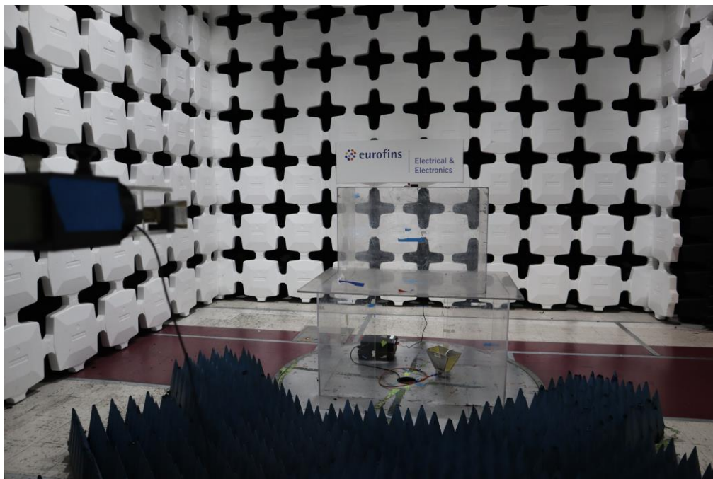
Figure 6. Radiated Spurious Emissions, (18 – 20 GHz) Test Setup
