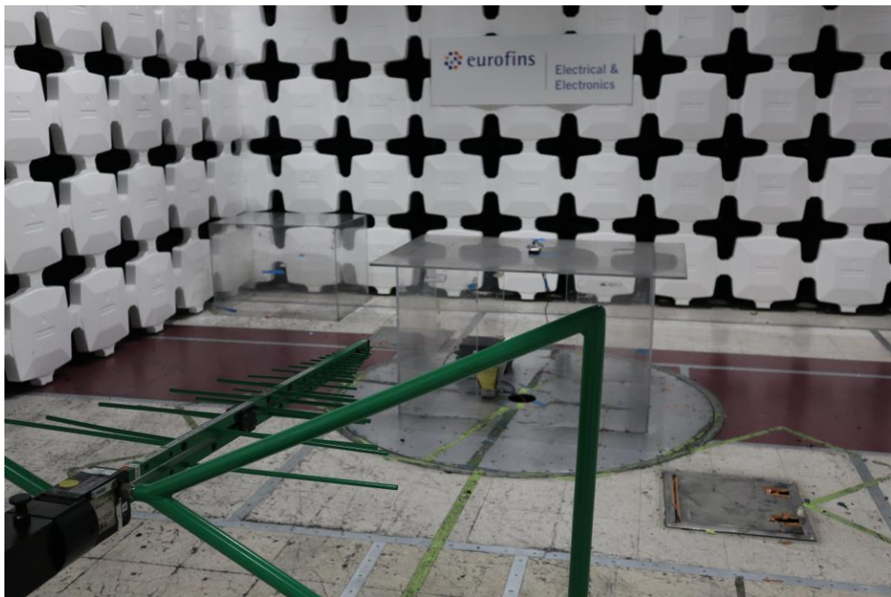
Figure 2. Radiated Spurious Emissions, (30 MHz – 1 GHz) Test Setup
