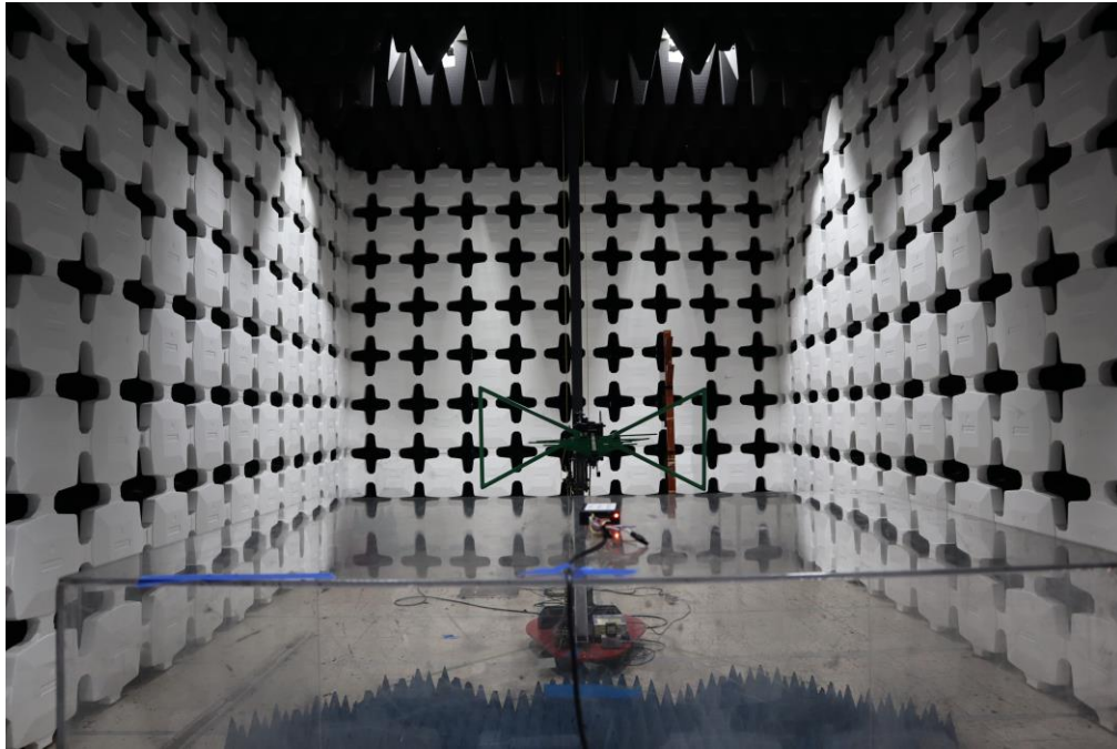
Figure 7. Radiated Spurious Emissions, (30 MHz – 1 GHz) Test Setup
