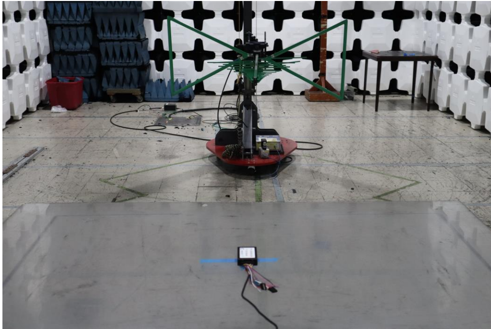
Figure 1. Radiated Spurious Emissions, (30 MHz – 1 GHz) Test Setup
