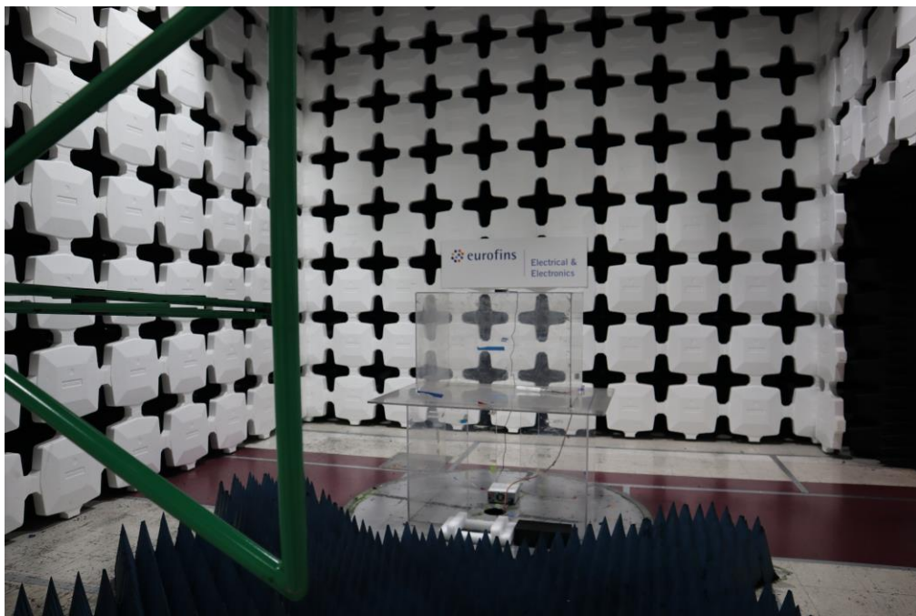
Figure 8. Radiated Spurious Emissions, (30 MHz – 1 GHz) Test Setup
