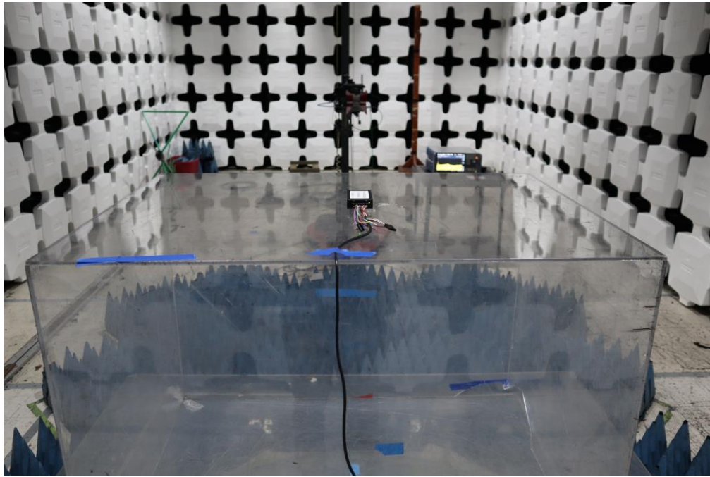
Figure 9. Radiated Spurious Emissions, (1 – 12.75 GHz) Test Setup
