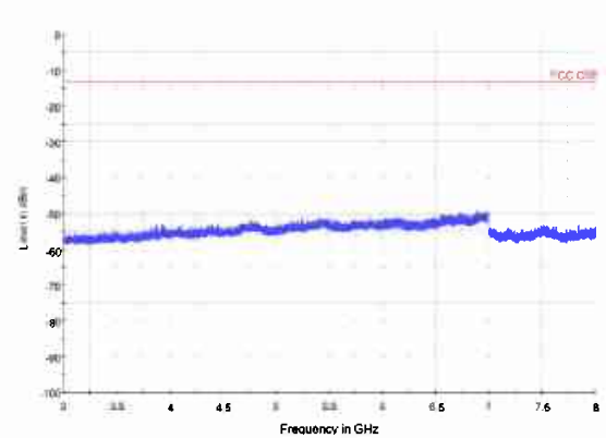
LTE Band 12 1.4MHz CH-Middle 3GHz~8GHz
