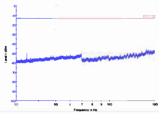
LTE Band 4 20MHz CH-High 3GHz~18GHz
