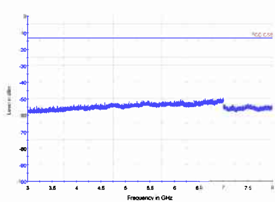
LTE Band 12 1.4MHz CH-Low 3GHz~8GHz
