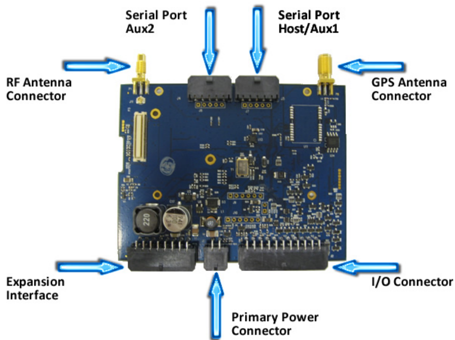
LMU-3640™ Connectors
