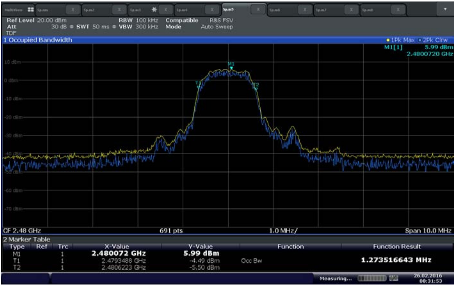
8DPSK High Channel
