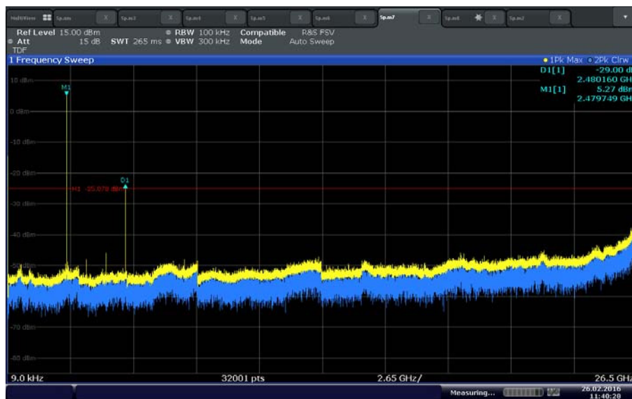
High Channel ( \pi/4 -DQPSK) – 2 nd harmonic complies with 20dBc
