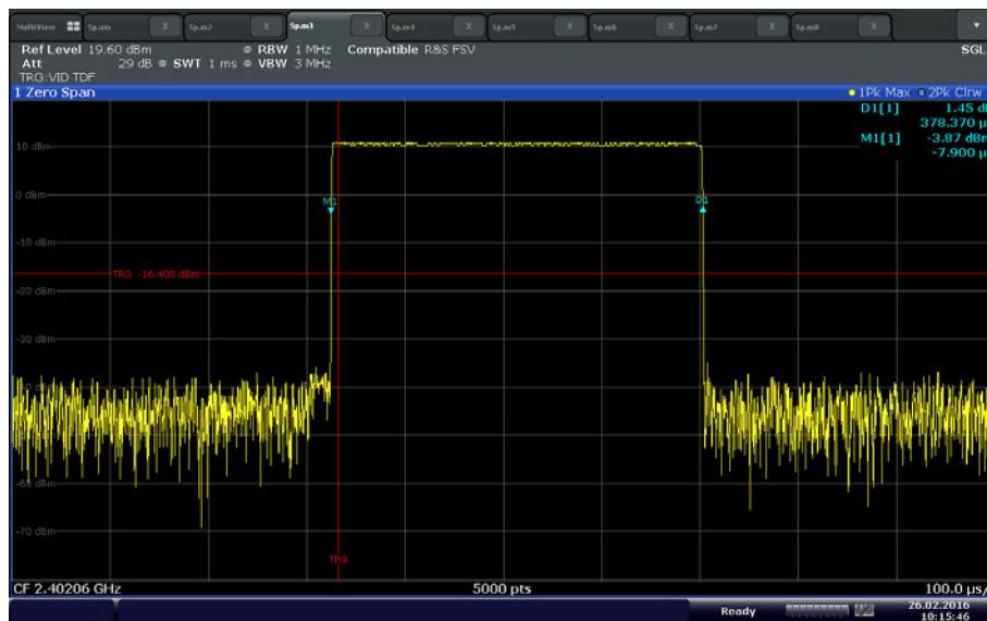
GFSK width of single pulse (0.37837ms)
