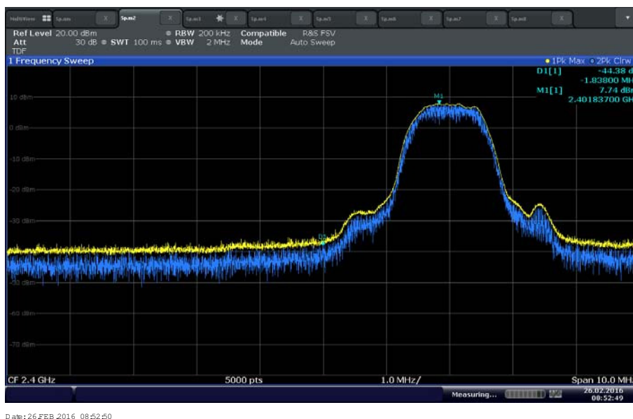
Non-hopping lower bandedge (8DPSK)
