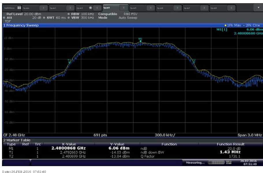
8DPSK High Channel
