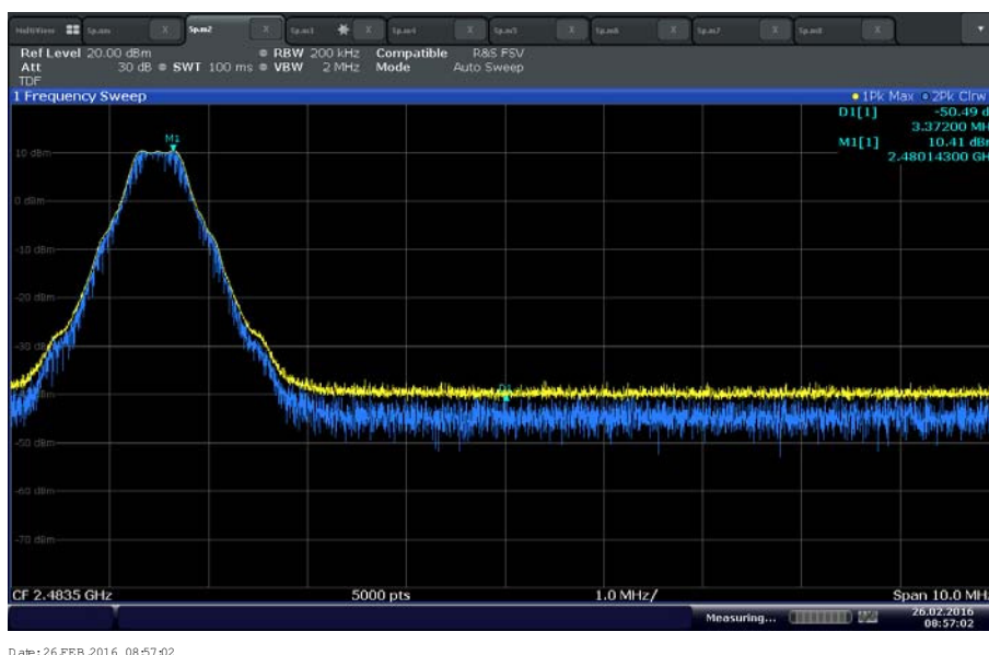
Non-hopping upper bandedge (GFSK)
