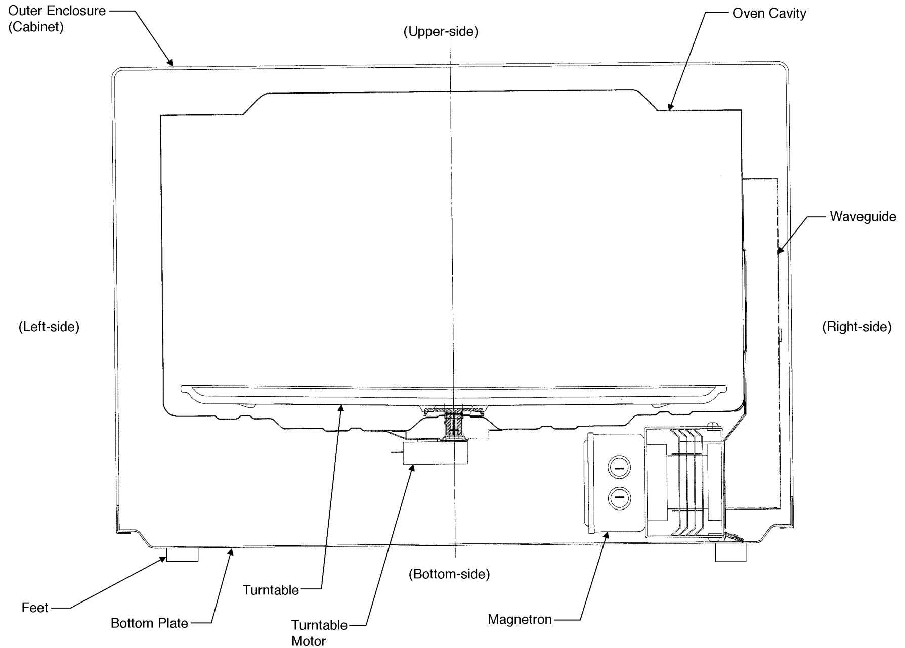
Fig. - 5 FCC ID: APYDMR0130 Shows a section drawing from front side view of Model R-630D, and shows a magnetron mounting location.
