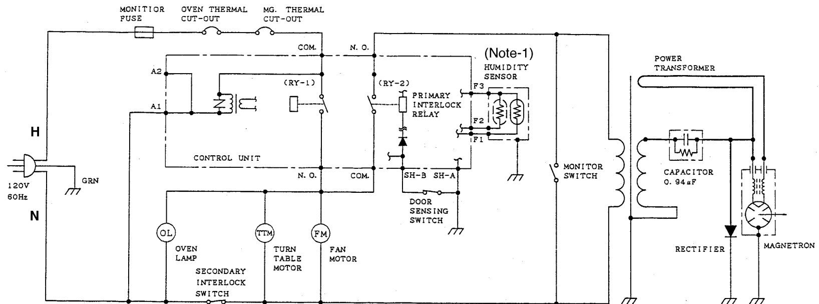
SCHEMATIC DIAGRAM (DOOR CLOSED, COOK OFF CONDITION)
