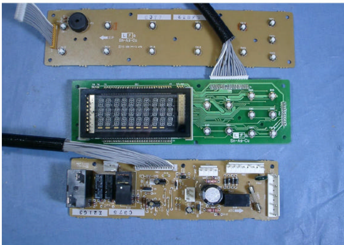
PHOTO.-05 APYDMR0143 Shows a printed wiring board assembly of Model R-8000G.
