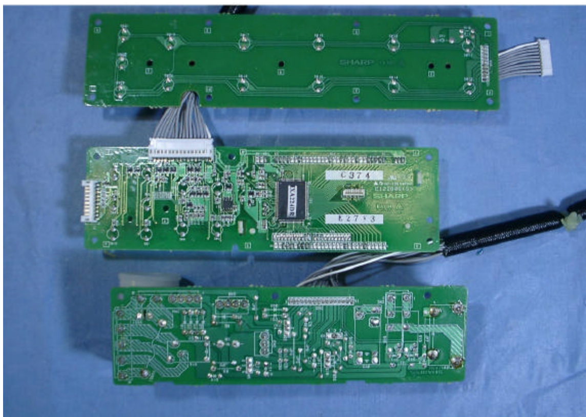
PHOTO.-06 APYDMR0143 Shows a back-side view of printed wiring board assembly for Model R-8000G.
