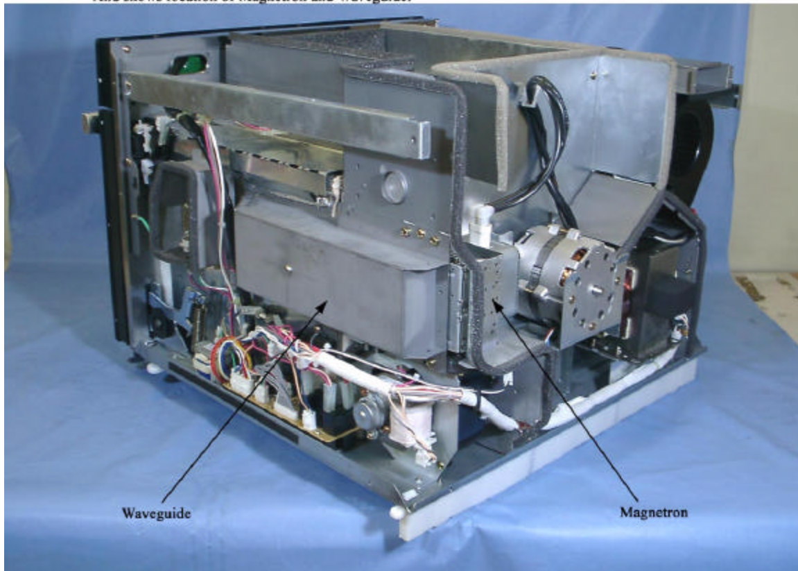
PHOTO.-04 APYDMR0143 Shows an inside view of Model R-8000G with outer case removed. And shows location of Magnetron and Waveguide.
