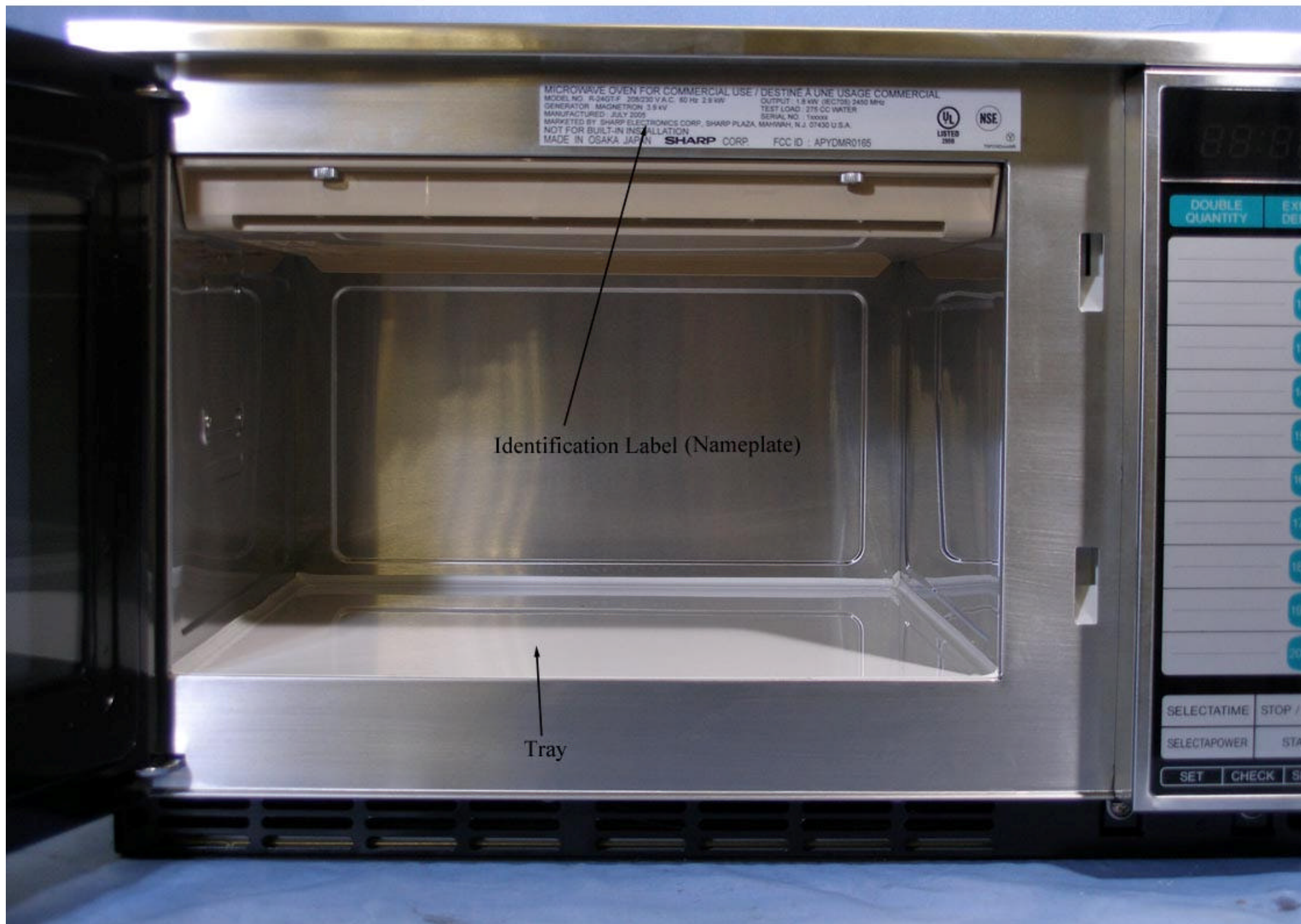
Photo.-03 FCC ID: APYDMR0165 Shows an oven cavity of model R-24GT# with door open, and shows Identification Label.
