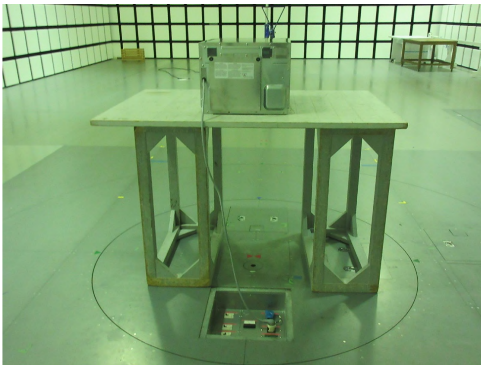
– Rear View –
