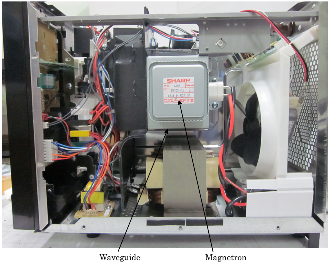
Fig. 5: Internal right side view with outer enclosure removed.
