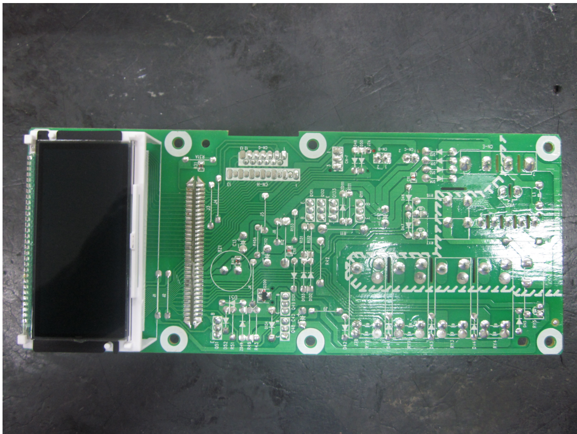
Fig. 7: Back-side of control unit PWB assembly.
