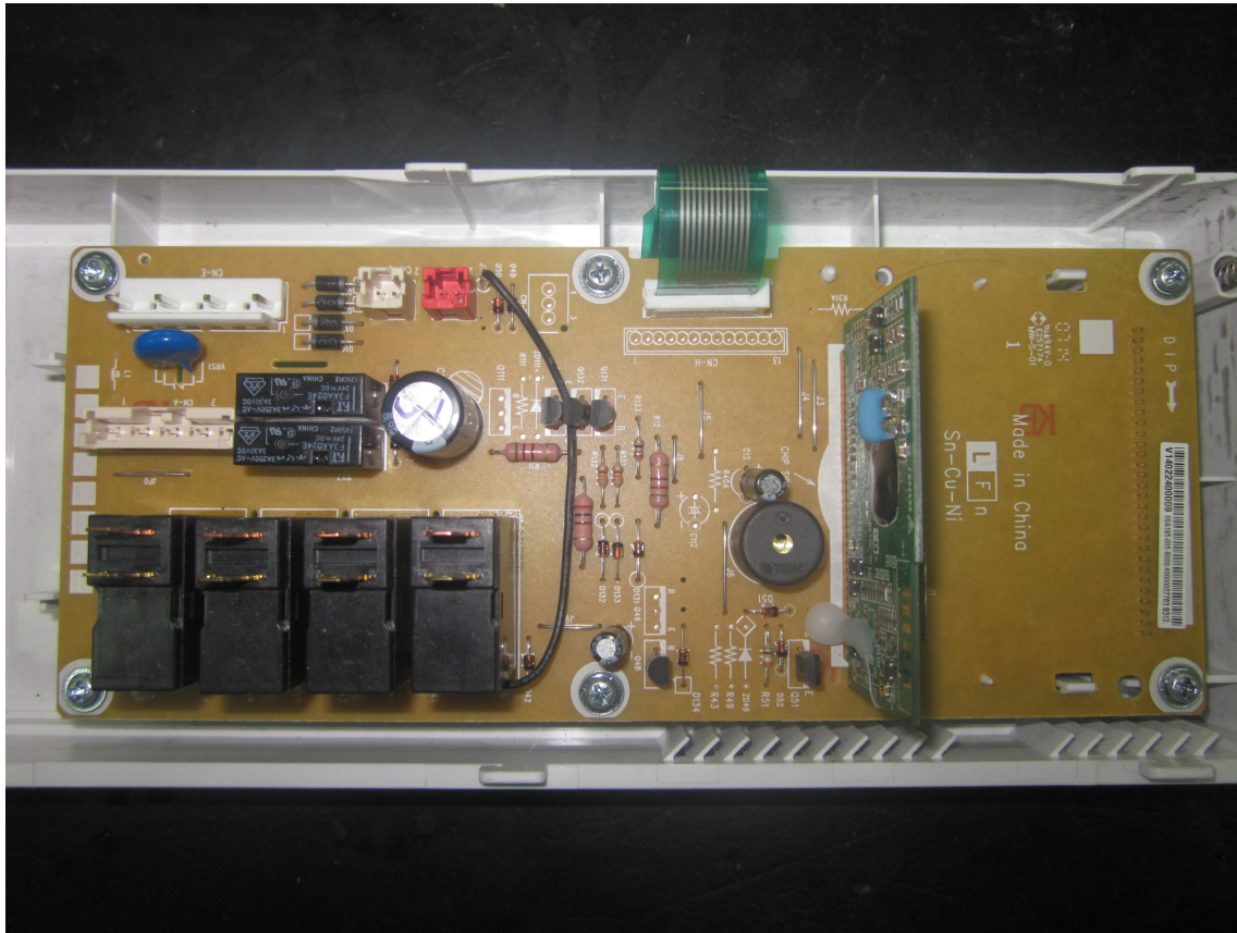
Fig. 6: Control unit PWB assembly.
