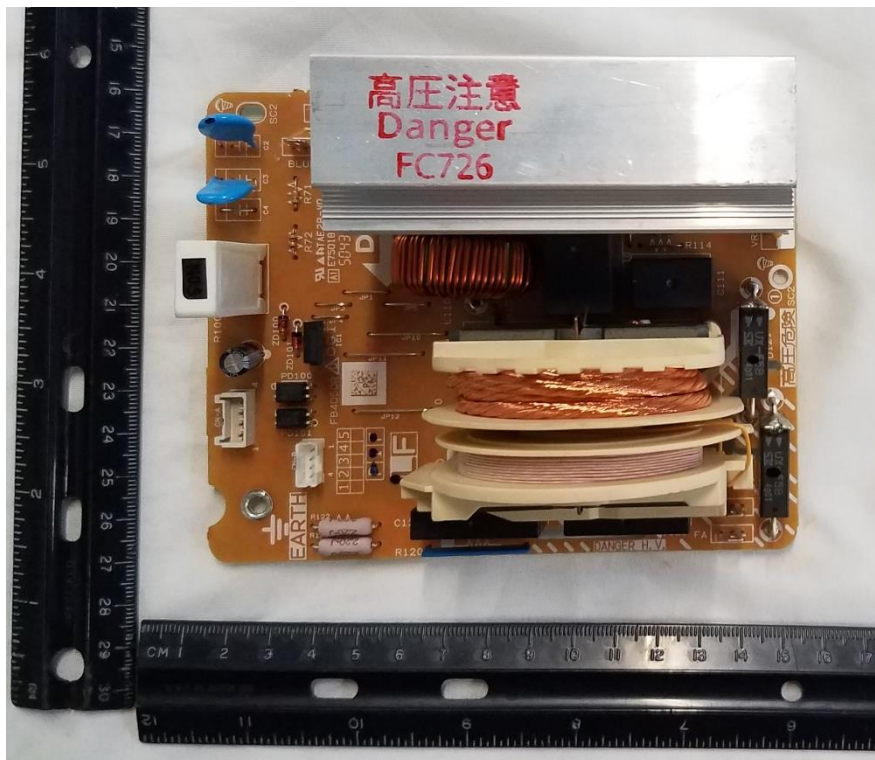
Figure 7. Inverter Top Side
