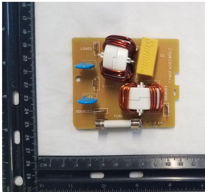
Figure 13. 120V Power Input Filter Top Side
