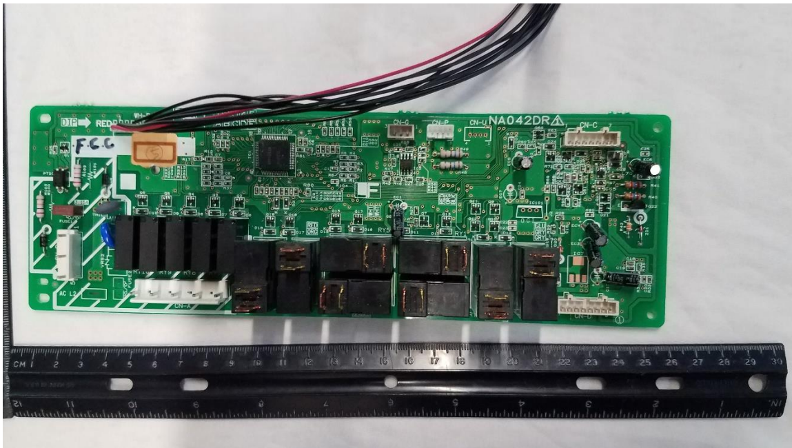
Figure 17. Power Control Board Top Side
