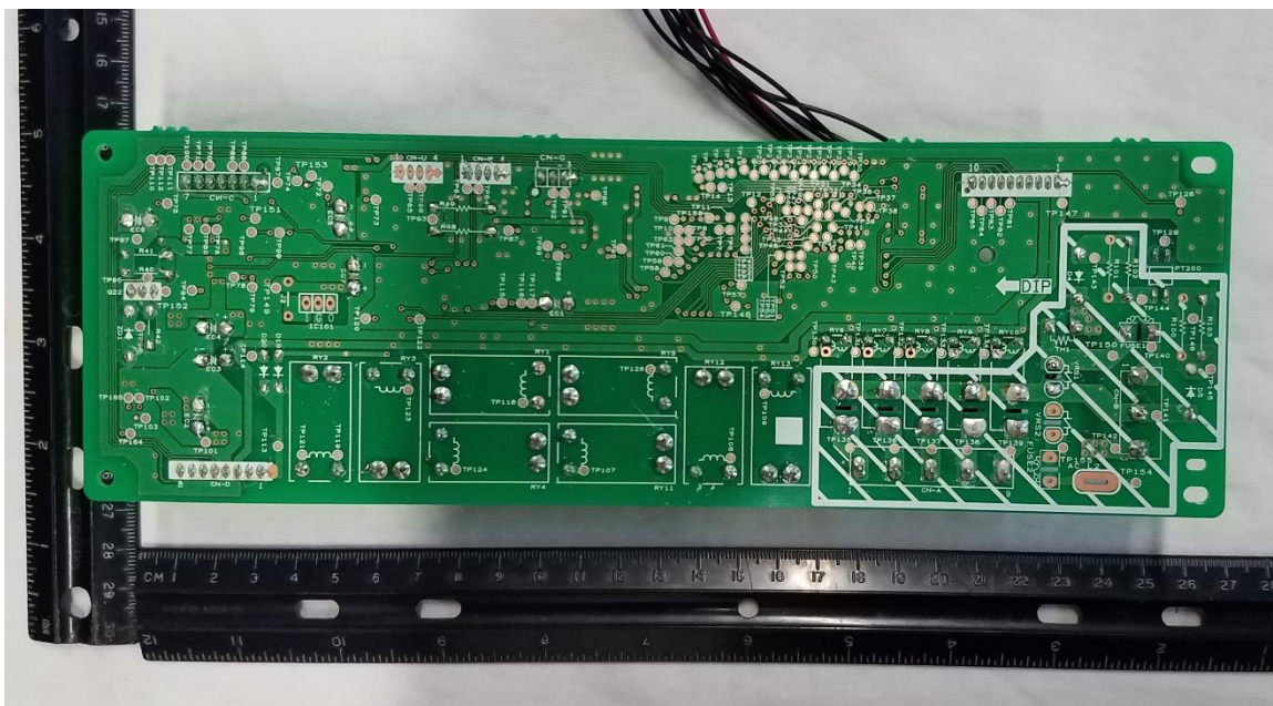
Figure 18. Power Control Board Bottom Side
