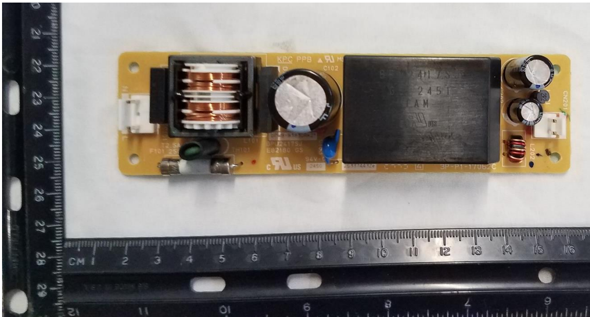
Figure 9. Auxiliary Power Supply Top Side
