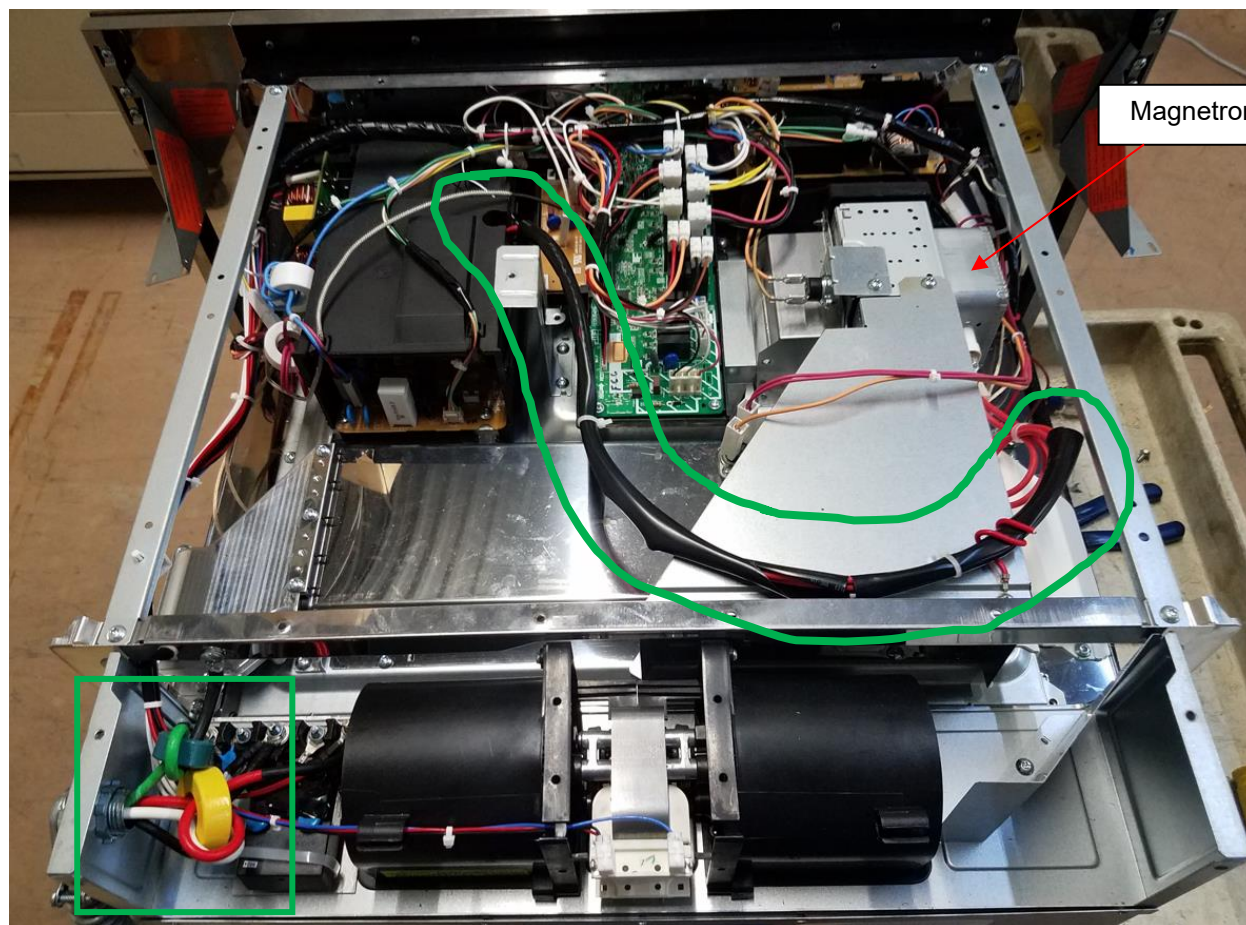
Figure 2. Top and Rear View
