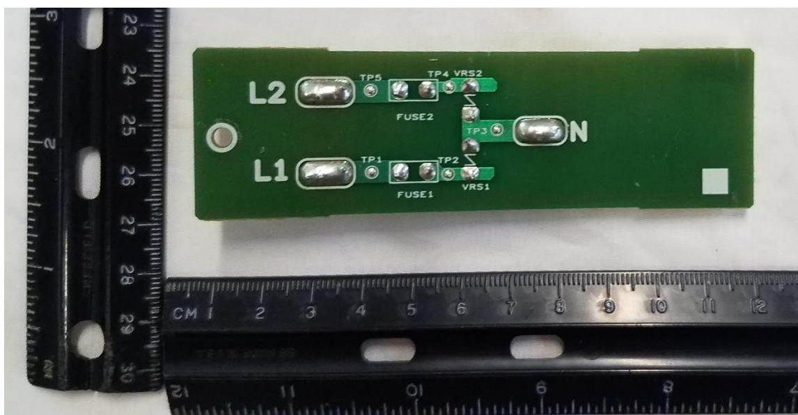
Figure 15. 240V Power Input Filter Bottom Top Side
