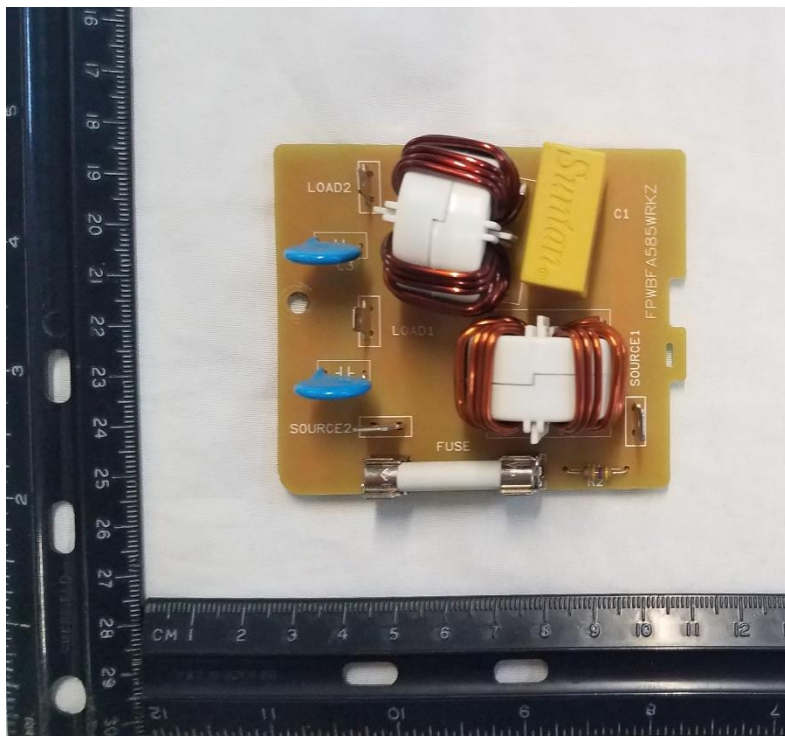
Figure 12. 120V Power Input Filter Top Side
