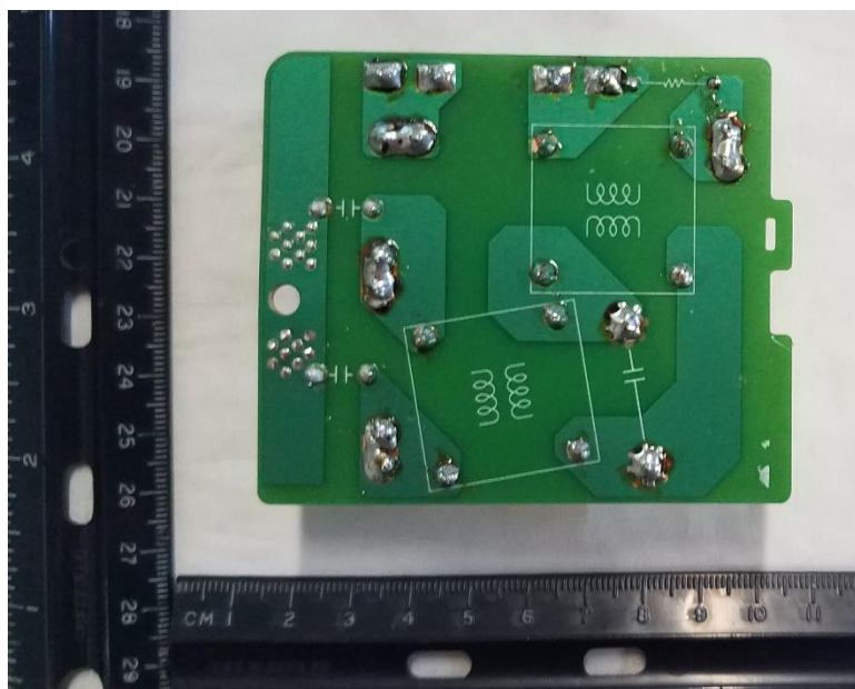
Figure 13. 120V Power Input Filter Bottom Side
