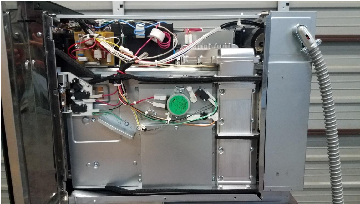
Figure 4. Right Side
