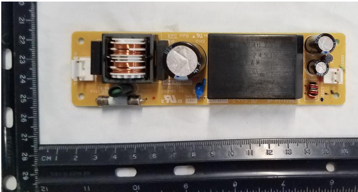
Figure 8. Auxiliary Power Supply Top Side
