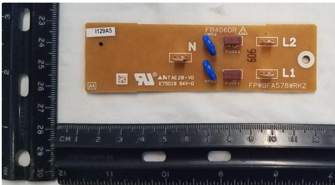
Figure 14. 240V Power Line Filter Top Side
