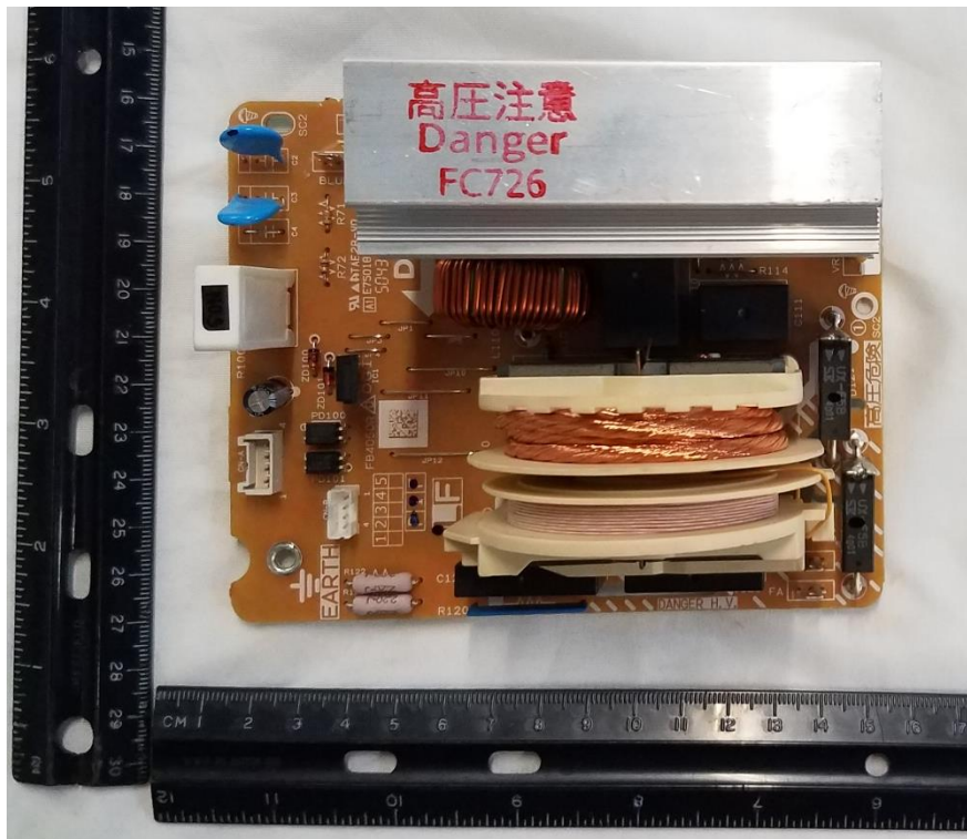
Figure 6. Inverter Top Side
