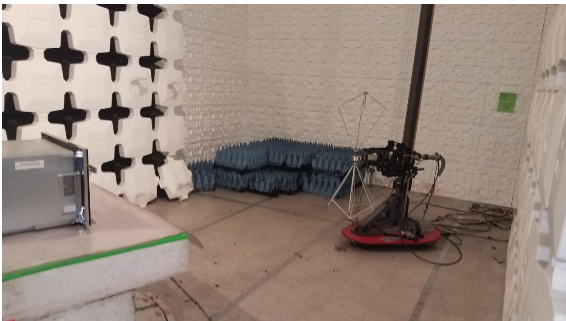
Figure 2. Radiated Emissions Measurement Photo, 30 to 200 MHz
