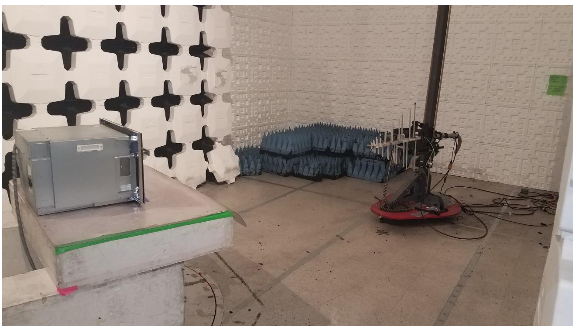
Figure 3. Radiated Emissions Measurement Photo, 200 to 1000 MHz
