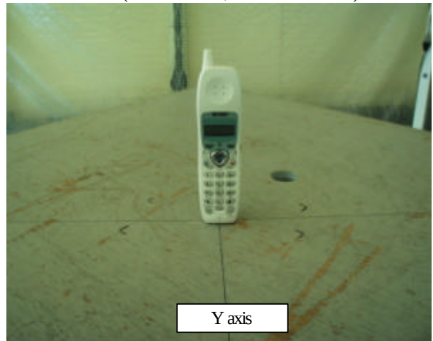
Worse case (30MHz-1GHz, Antenna: Vertical)
