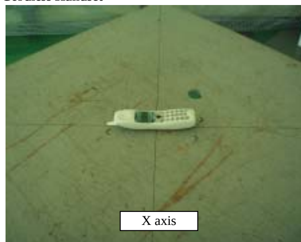
Worse case (30MHz-26GHz , Antenna: Horizontal)
