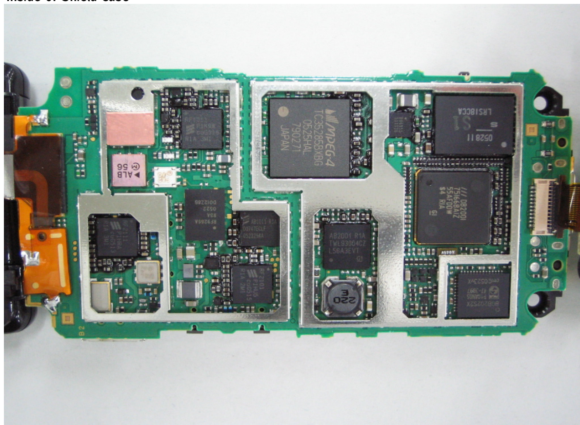
Inside of Shield case
