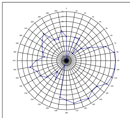
Antenna 0 vertical
