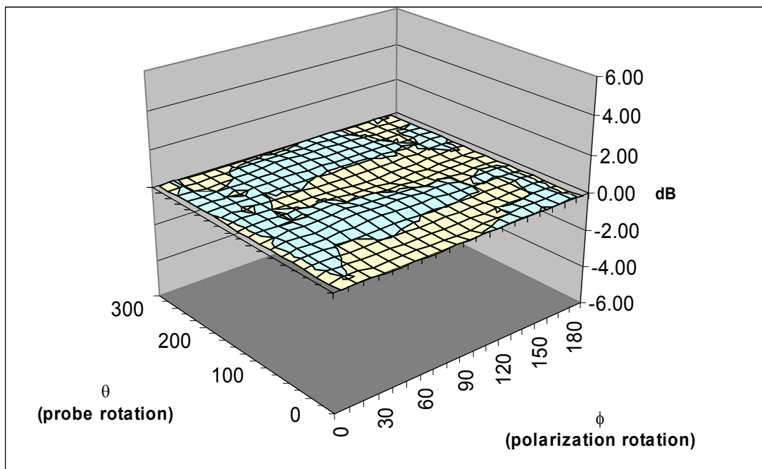
Figure 1 Surface Isotropy diagram of IXP-050 Probe S/N 0206 at 900MHz (rotational isotropy axial \pm 0.12 dB, spherical isotropy \pm 0.22 dB)
