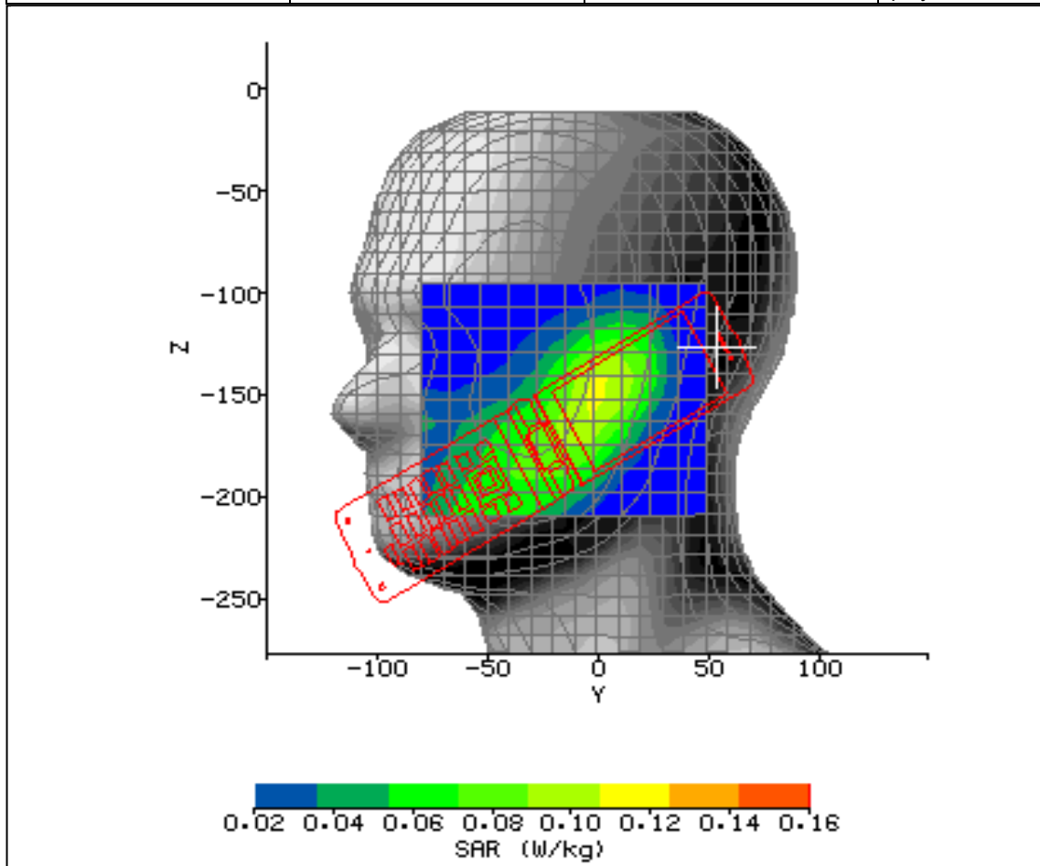
Figure 9: SAR Head Testing Results for the SH011 Mobile Handset at 824.7MHz.
