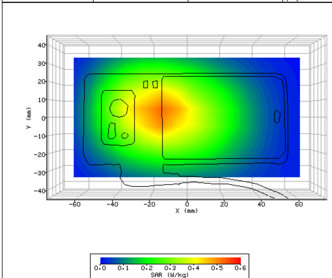
Figure 13: SAR Body Testing Results for the SH011 Mobile Handset at 824.7MHz.
