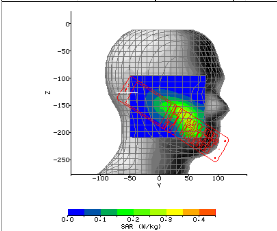
Figure 10: SAR Head Testing Results for the SH011 Mobile Handset at 824.7MHz.
