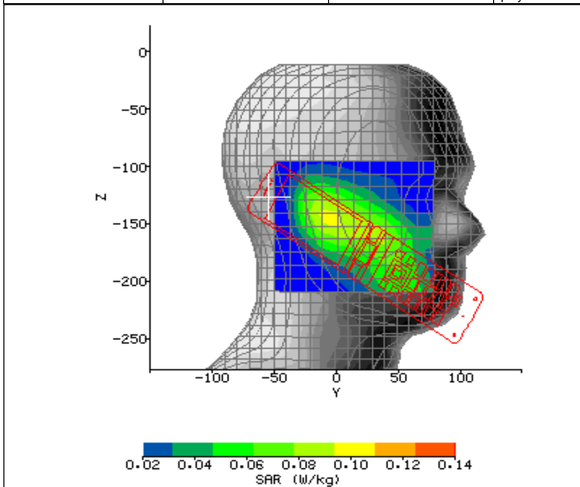
Figure 11: SAR Head Testing Results for the SH011 Mobile Handset at 824.7MHz.
