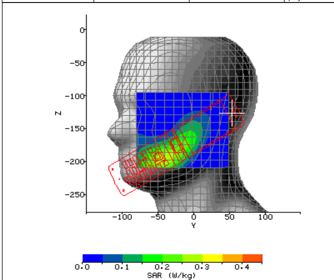
Figure 8: SAR Head Testing Results for the SH011 Mobile Handset at 824.7MHz.
