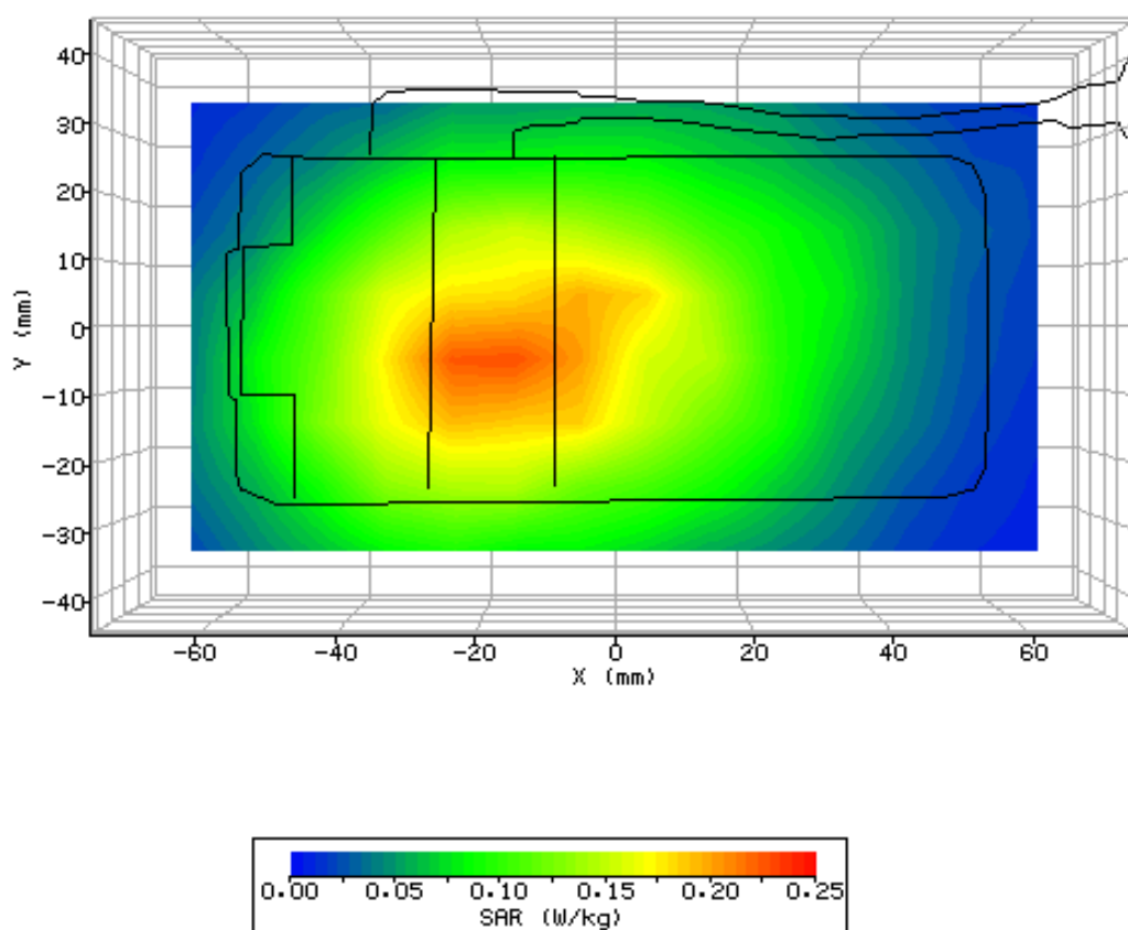
Figure 12: SAR Body Testing Results for the SH011 Mobile Handset at 824.7MHz.
