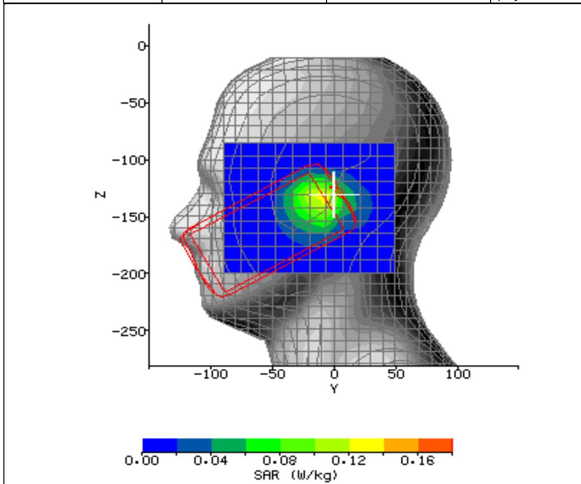
Figure 14: SAR Head Testing Results for the CDMA SHI13 Mobile Handset at 2412MHz.
