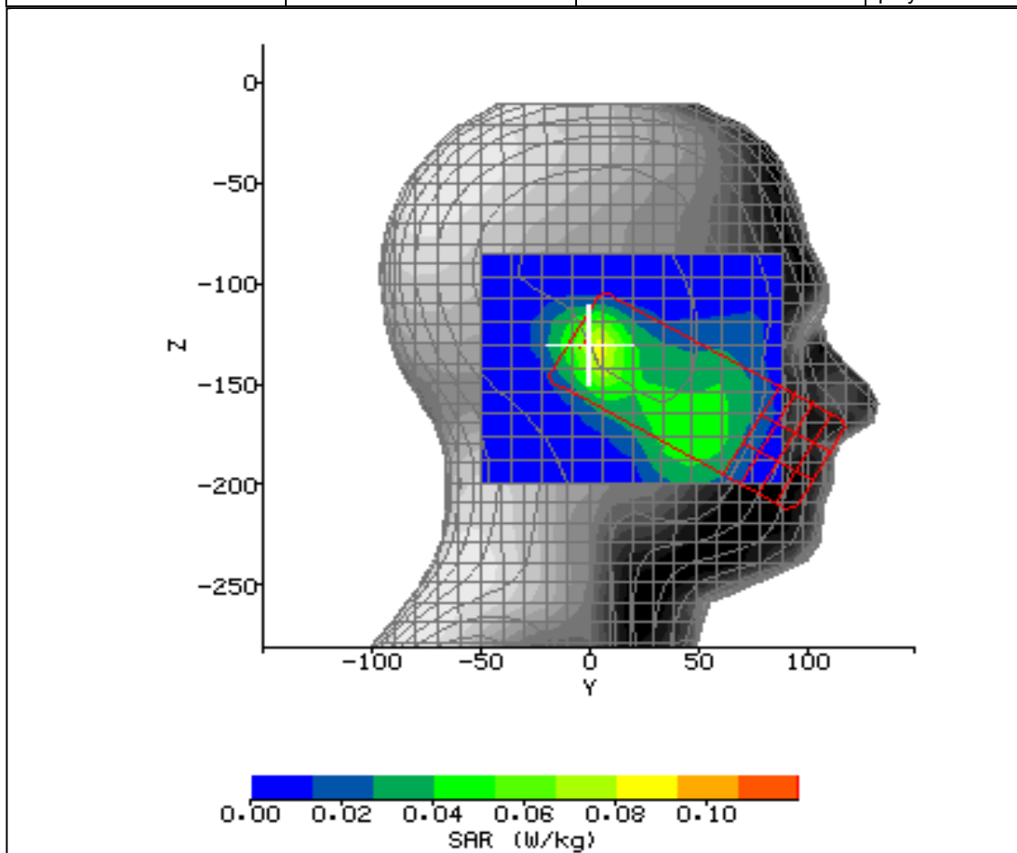
Figure 17: SAR Head Testing Results for the Sharp CDMA SHX12 Mobile Handset at 1880MHz.
