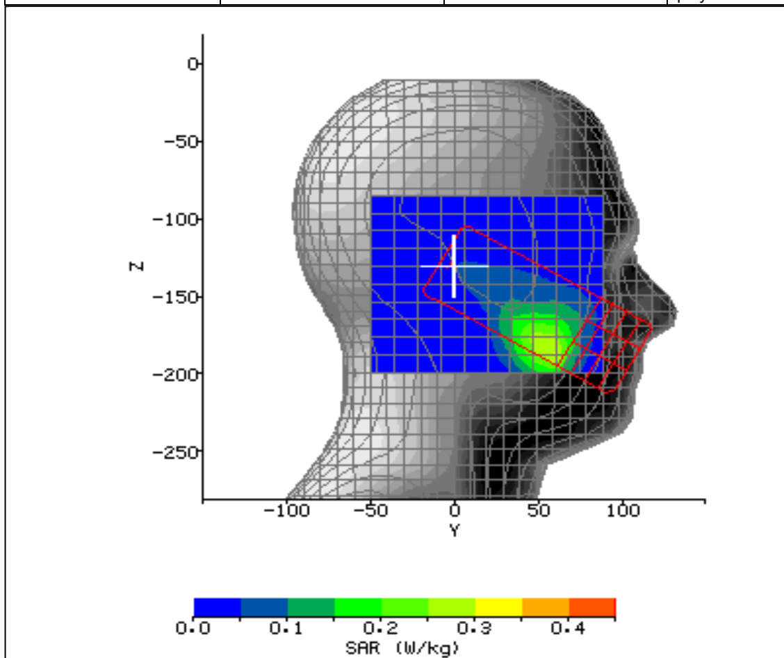
Figure 16: SAR Head Testing Results for the Sharp CDMA SHX12 Mobile Handset at 1880MHz.
