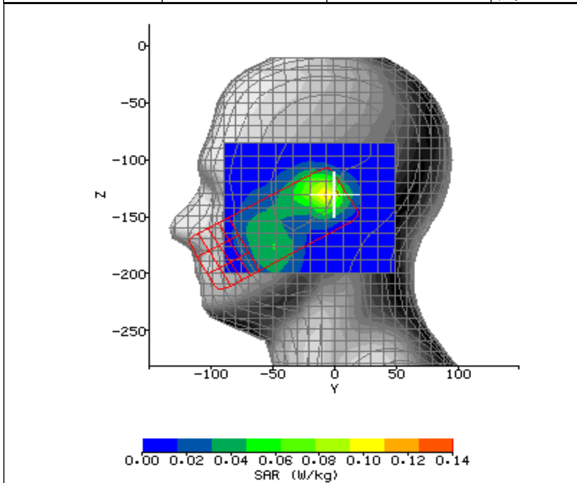
Figure 15: SAR Head Testing Results for the Sharp CDMA SHX12 Mobile Handset at 1880MHz.
