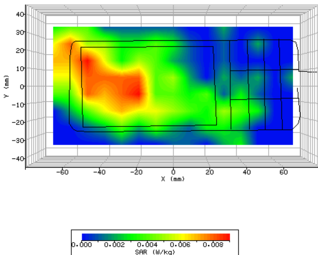
Figure 24: SAR Body Testing Results for the Sharp CDMA SHX12 Mobile Handset at 2437.0MHz.
