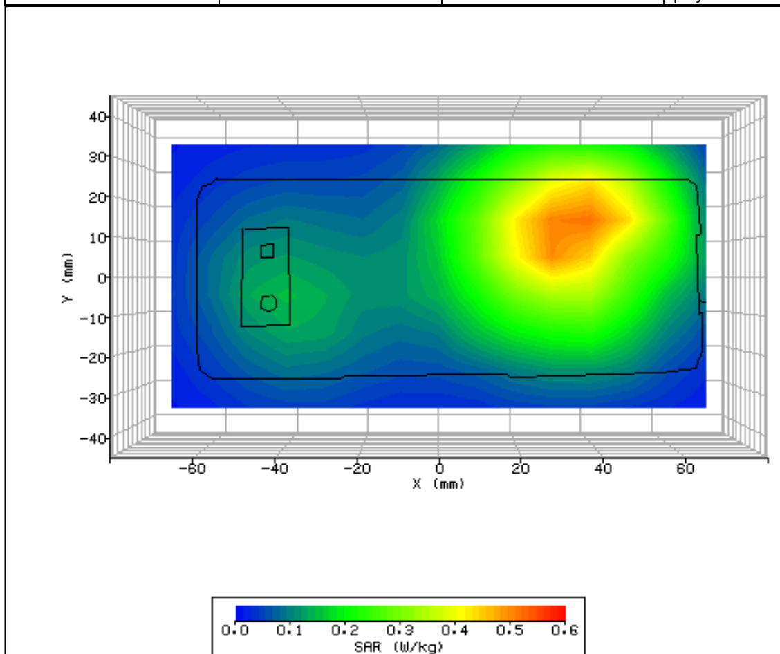
Figure 19: SAR Body Testing Results for the Sharp CDMA SHX12 Mobile Handset at 1880MHz.
