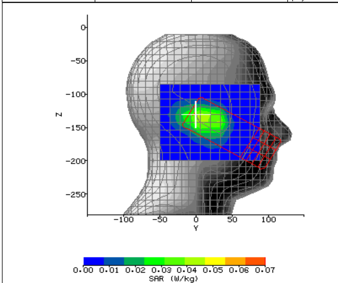
Figure 22: SAR Head Testing Results for the Sharp CDMA SHX12 Mobile Handset at 2437.0MHz.
