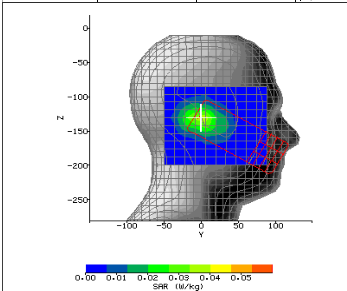
Figure 23: SAR Head Testing Results for the Sharp CDMA SHX12 Mobile Handset at 2437.0MHz.
