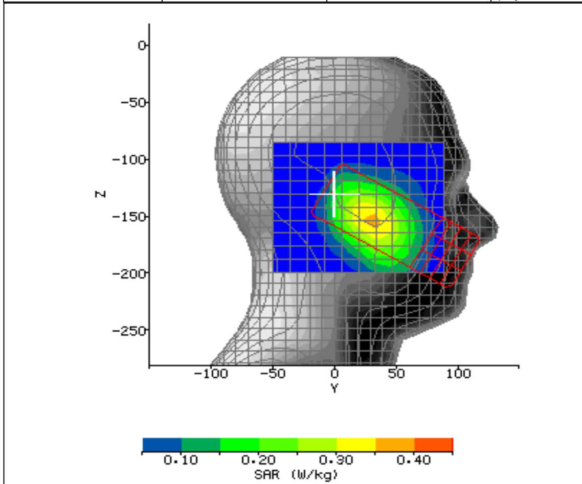
Figure 11: SAR Head Testing Results for the Sharp CDMA SHX12 Mobile Handset at 824.07MHz.
