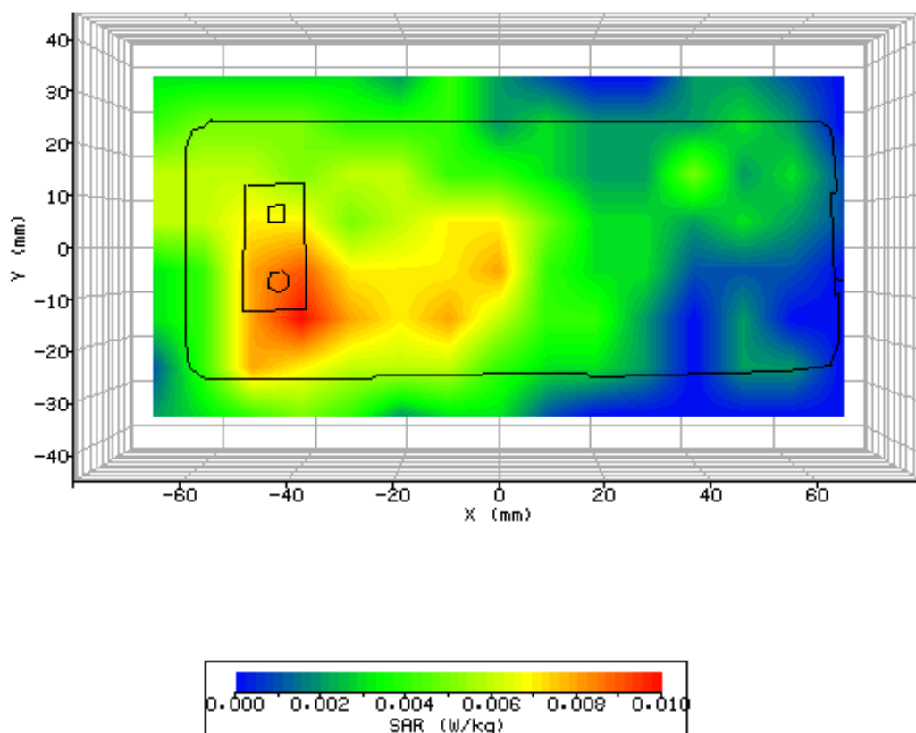
Figure 25: SAR Body Testing Results for the Sharp CDMA SHX12 Mobile Handset at 2437.0MHz.
