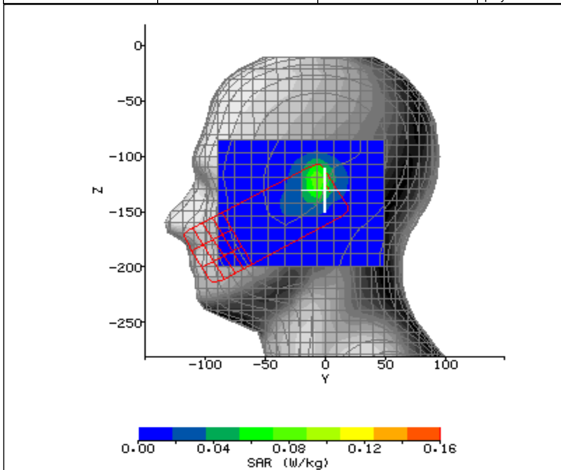
Figure 21: SAR Head Testing Results for the Sharp CDMA SHX12 Mobile Handset at 2437.0MHz.
