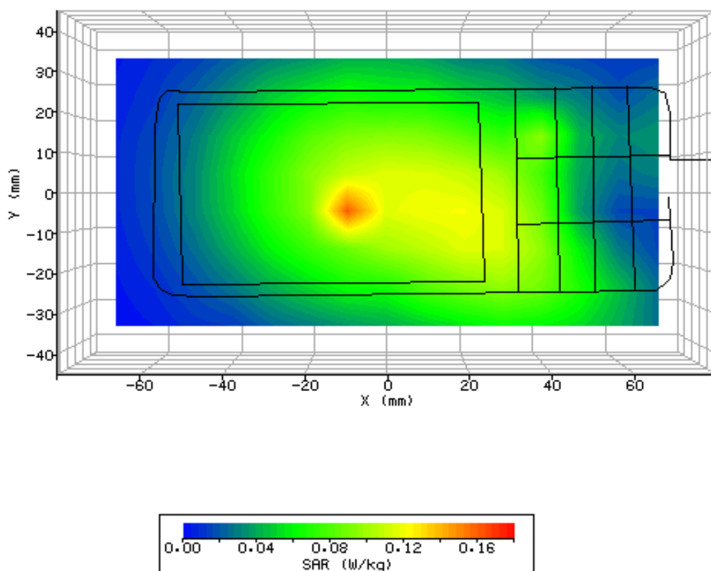
Figure 12: SAR Body Testing Results for the Sharp CDMA SHX12 Mobile Handset at 836.4MHz.
