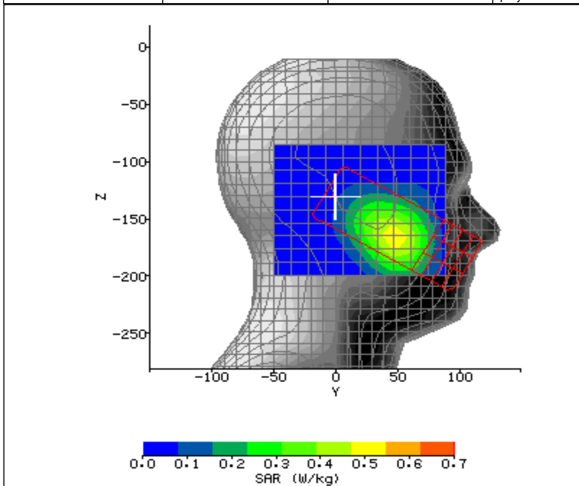
Figure 10: SAR Head Testing Results for the Sharp CDMA SHX12 Mobile Handset at 824.07MHz.
