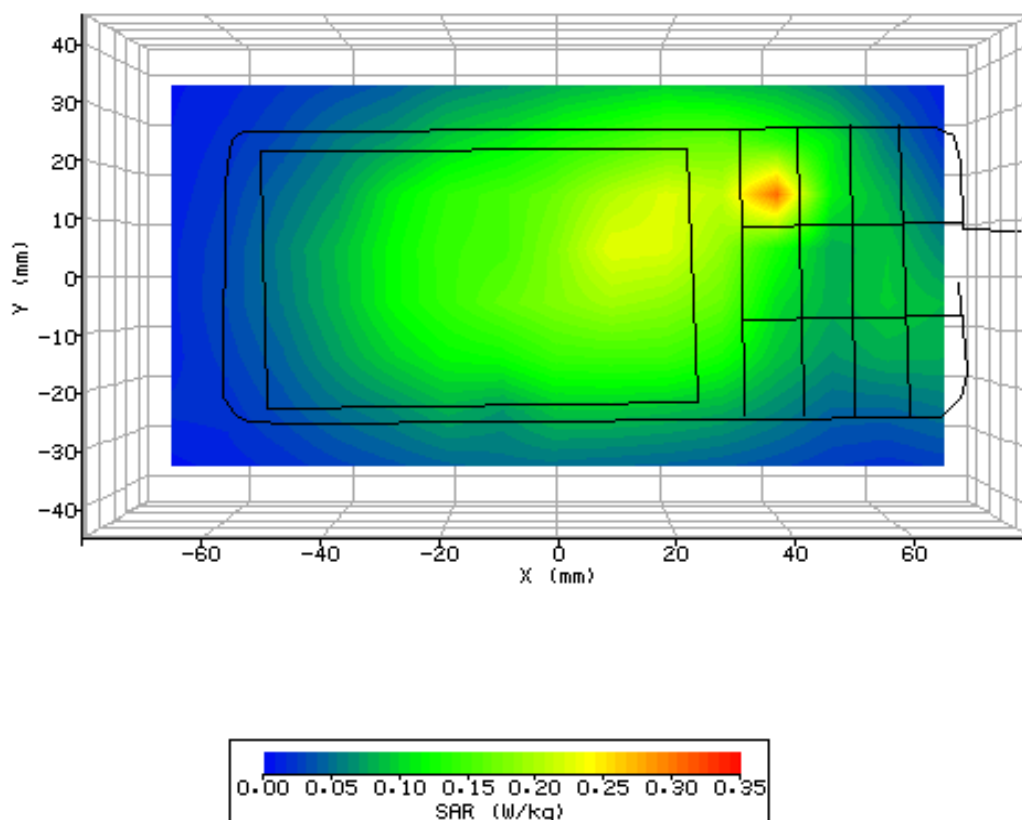
Figure 13: SAR Body Testing Results for the Sharp CDMA SHX12 Mobile Handset at 836.4MHz.
