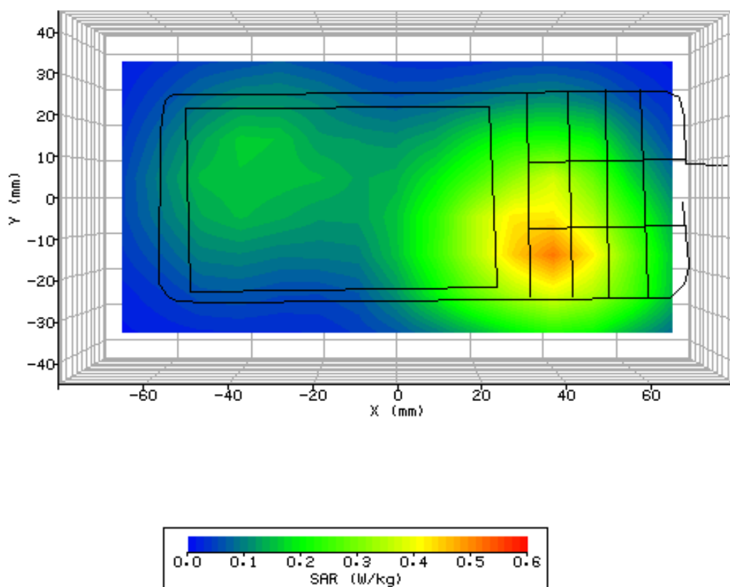
Figure 18: SAR Body Testing Results for the Sharp CDMA SHX12 Mobile Handset at 1880MHz.
