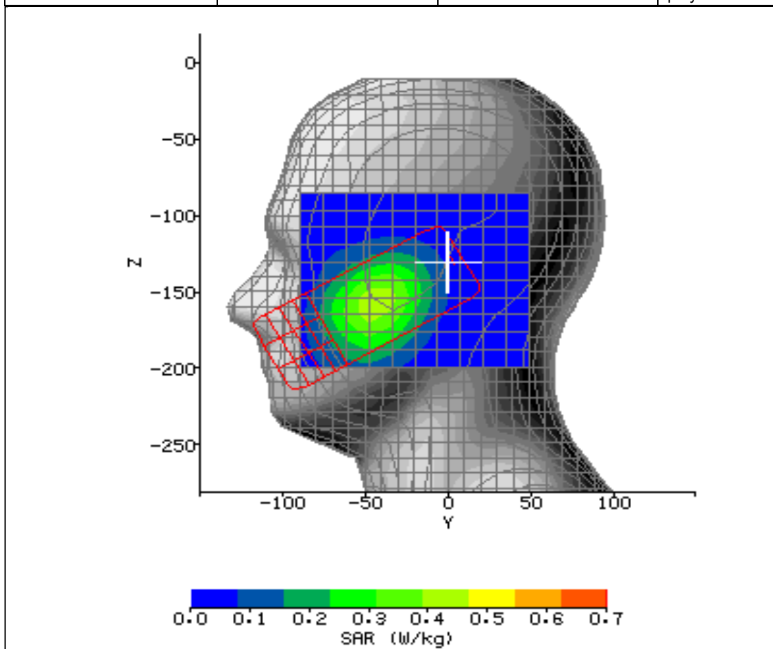
Figure 8: SAR Head Testing Results for the Sharp CDMA SHX12 Mobile Handset at 824.07MHz.
