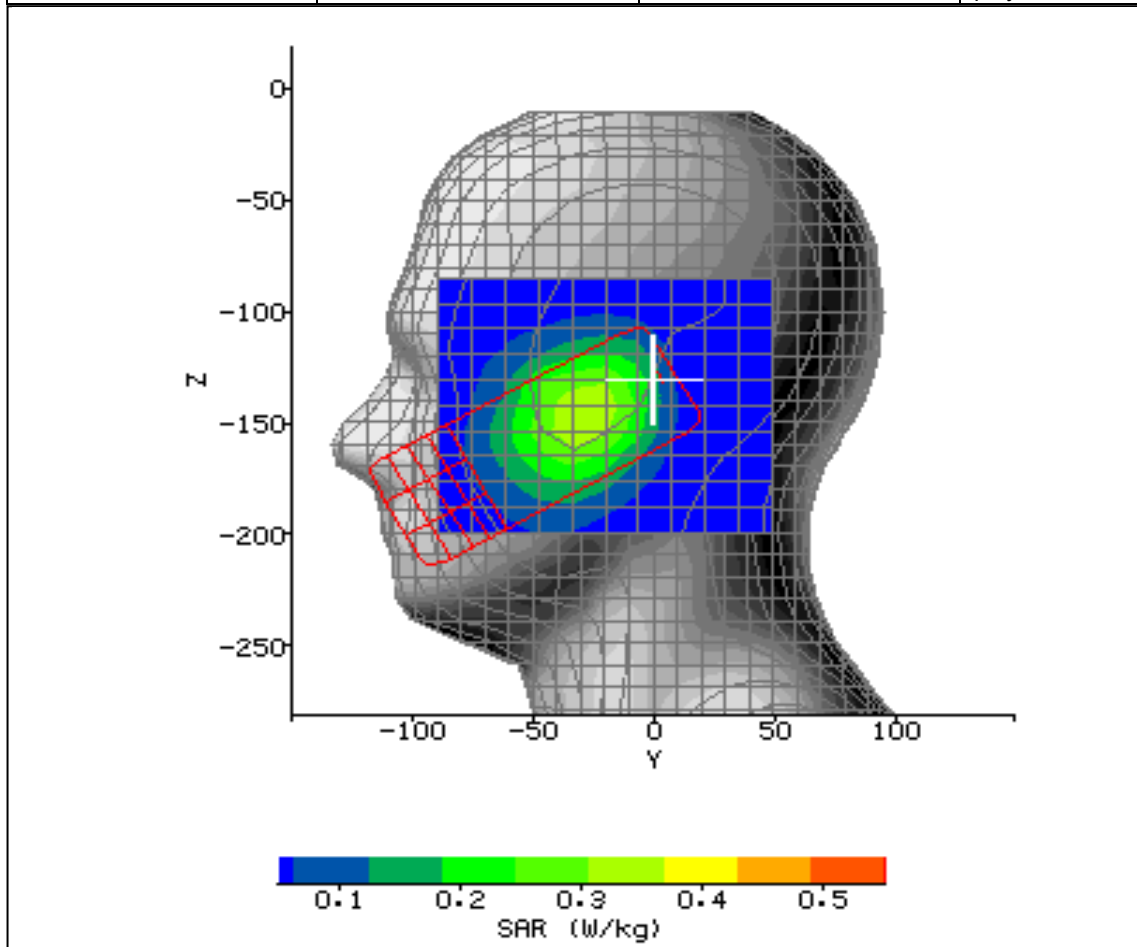
Figure 9: SAR Head Testing Results for the Sharp CDMA SHX12 Mobile Handset at 824.07MHz.
