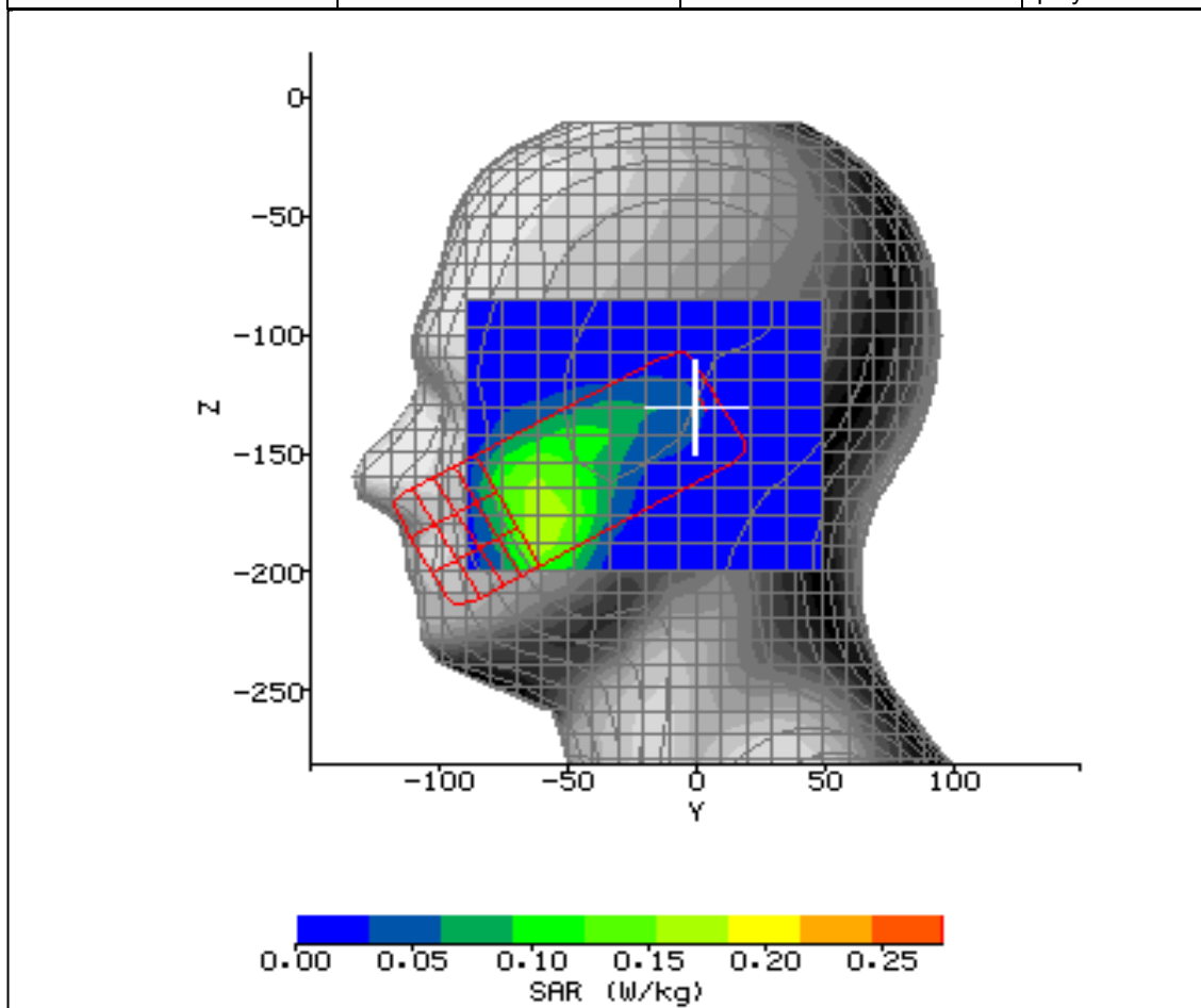
Figure 14: SAR Head Testing Results for the Sharp CDMA SHX12 Mobile Handset at 1880MHz.
