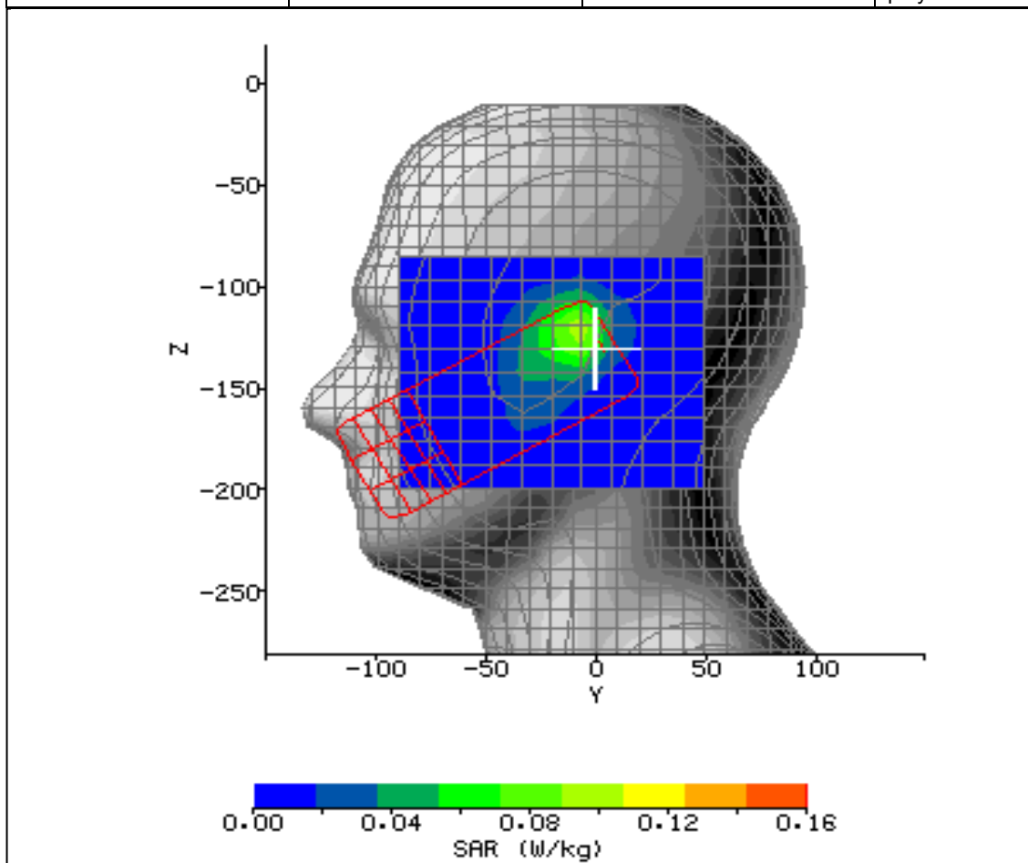
Figure 20: SAR Head Testing Results for the Sharp CDMA SHX12 Mobile Handset at 2437.0MHz.
