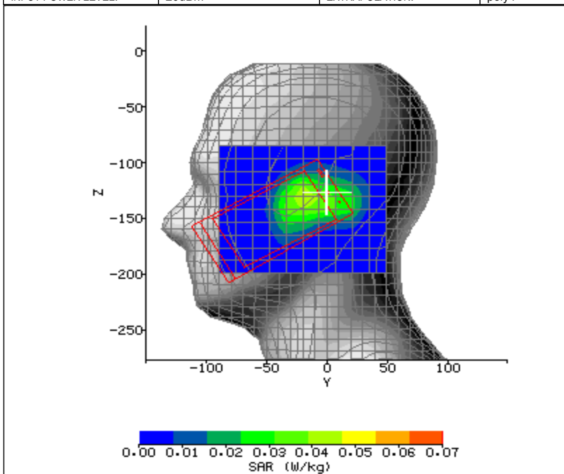
Figure 16: SAR Head Testing Results for the CDMA SHI11 Mobile Handset at 2437.0MHz.
