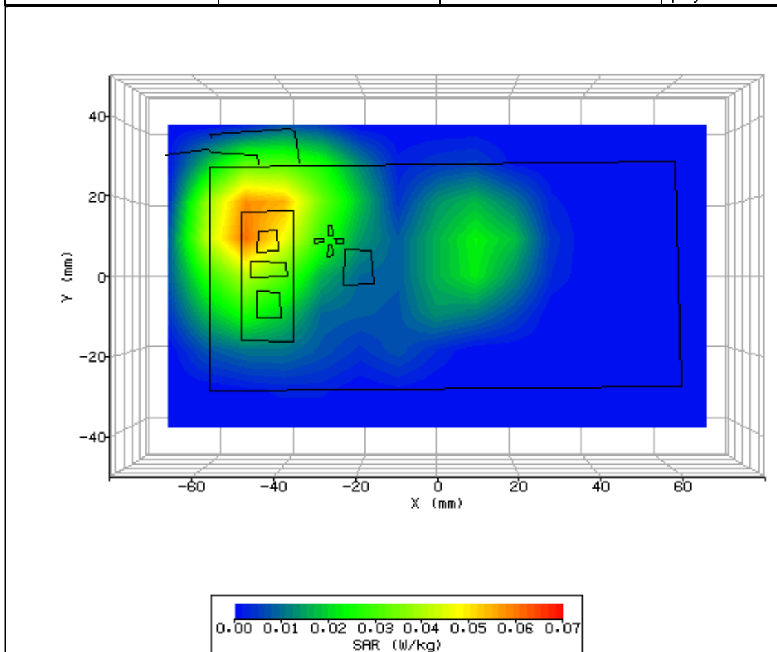
Figure 21: SAR Body Testing Results for the CDMA SHI11 Mobile Handset at 2437.0MHz.
