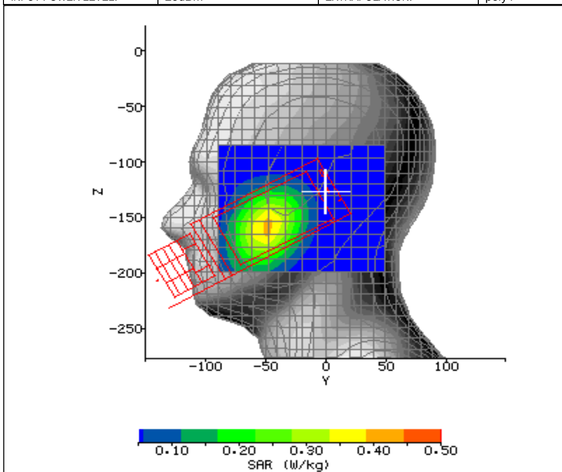
Figure 12: SAR Head Testing Results for the CDMA SHI11 Mobile Handset at 824.7MHz.
