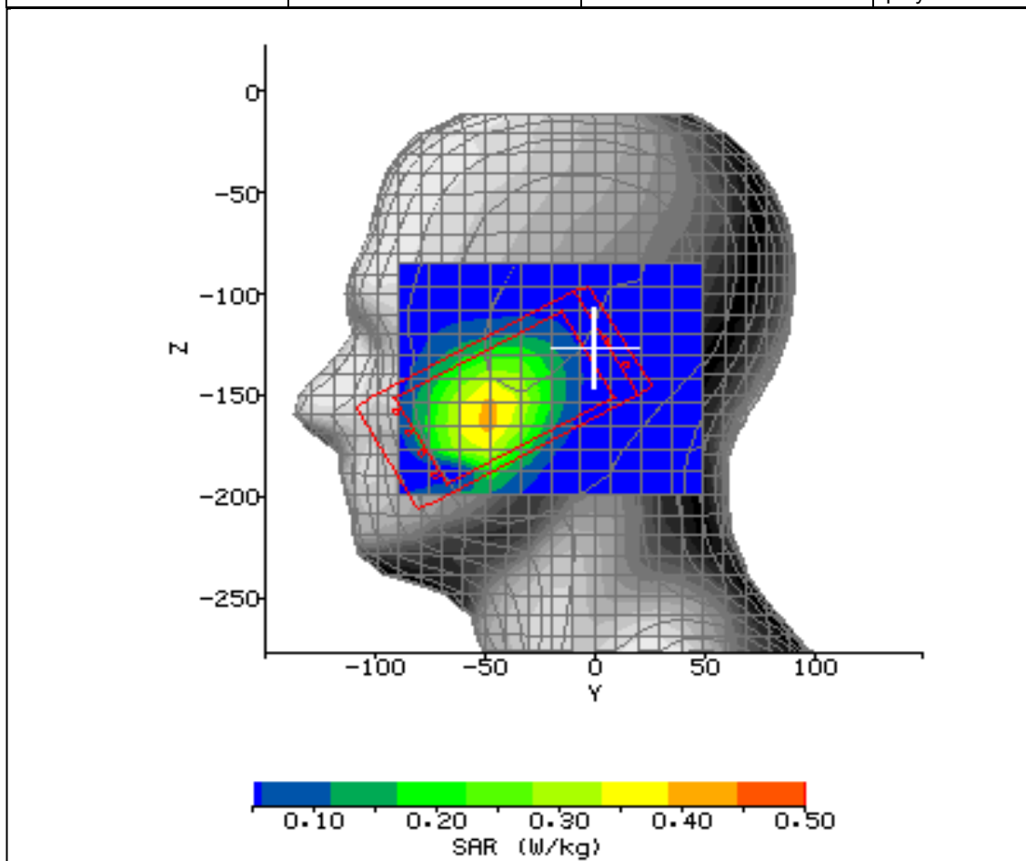
Figure 8: SAR Head Testing Results for the Sharp CDMA SHI14 Mobile Handset at 824.7MHz.
