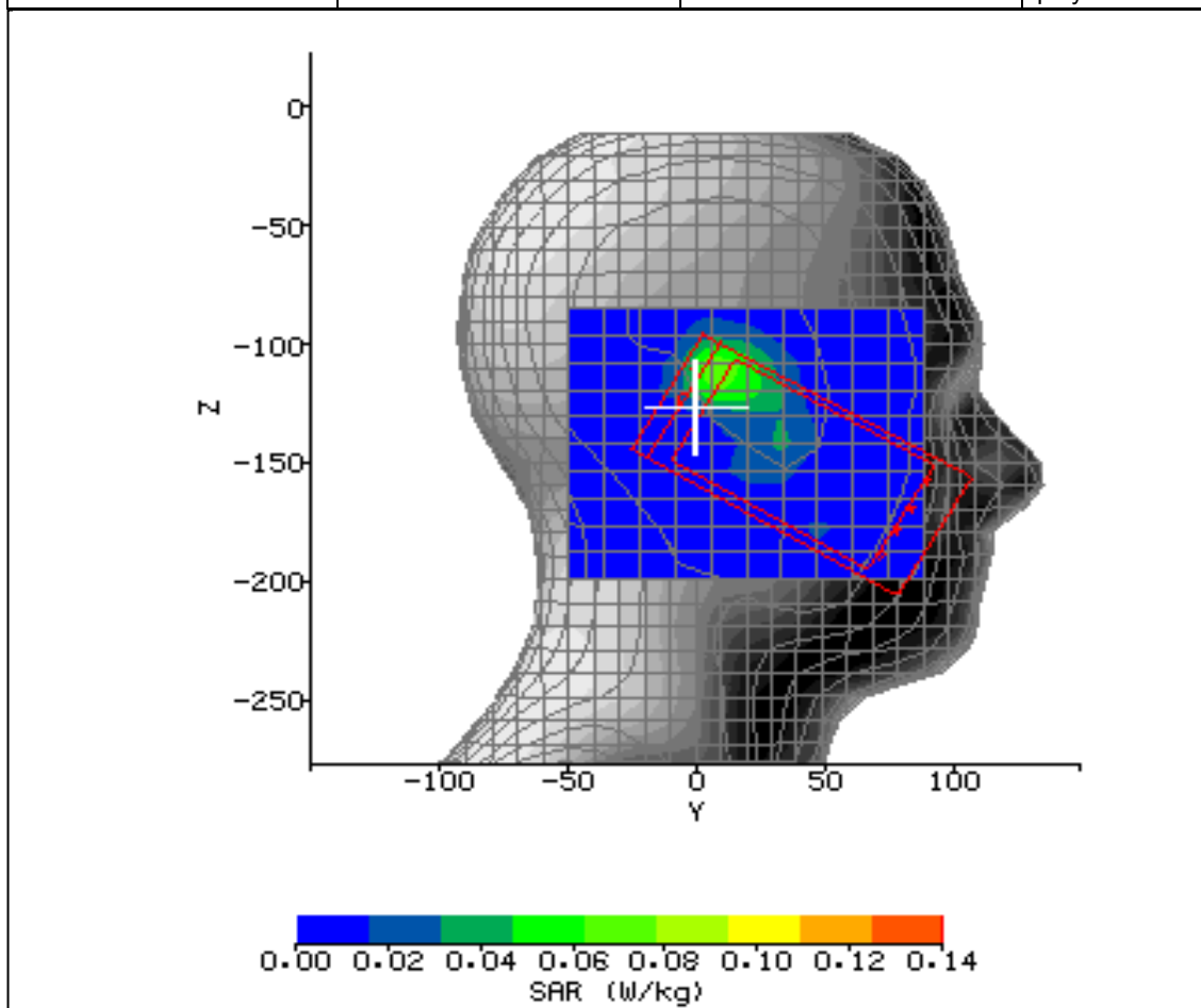
Figure 10: SAR Head Testing Results for the Sharp CDMA SHI14 Mobile Handset at 2437.0MHz.
