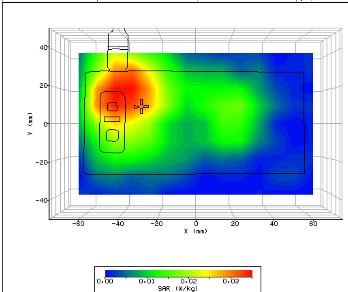
Figure 11: SAR Body Testing Results for the Sharp CDMA SHI14 Mobile Handset at 2437.0MHz.
