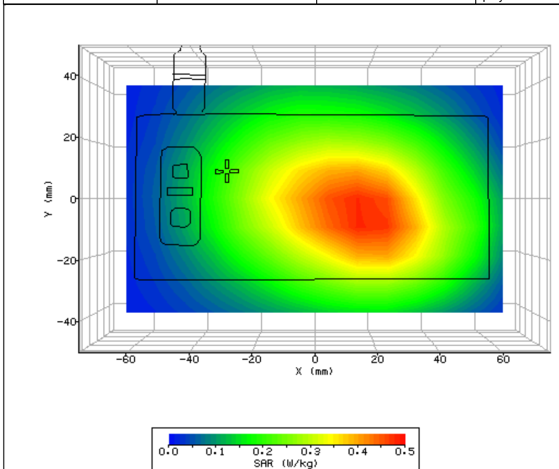
Figure 9: SAR Body Testing Results for the Sharp CDMA SHI14 Mobile Handset at 824.7MHz.
