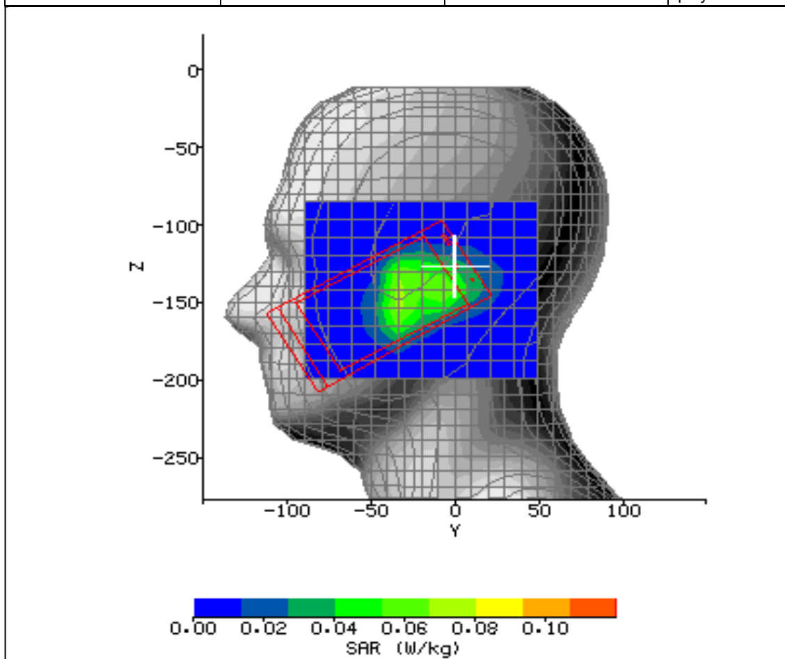
Figure 15: SAR Head Testing Results for the CDMA SHI11 Mobile Handset at 2437.0MHz.
