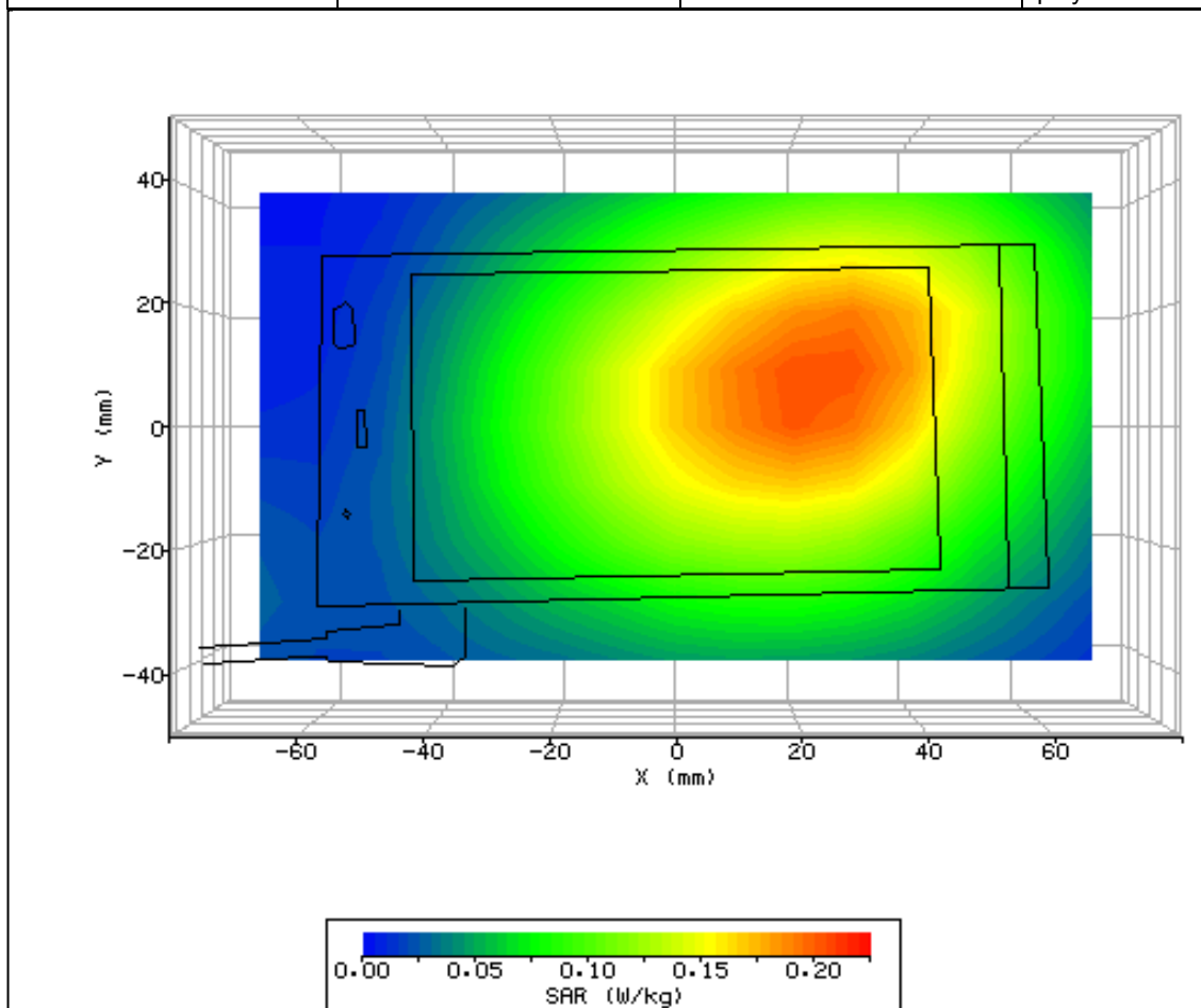
Figure 13: SAR Body Testing Results for the CDMA SHI11 Mobile Handset at 824.7MHz.
