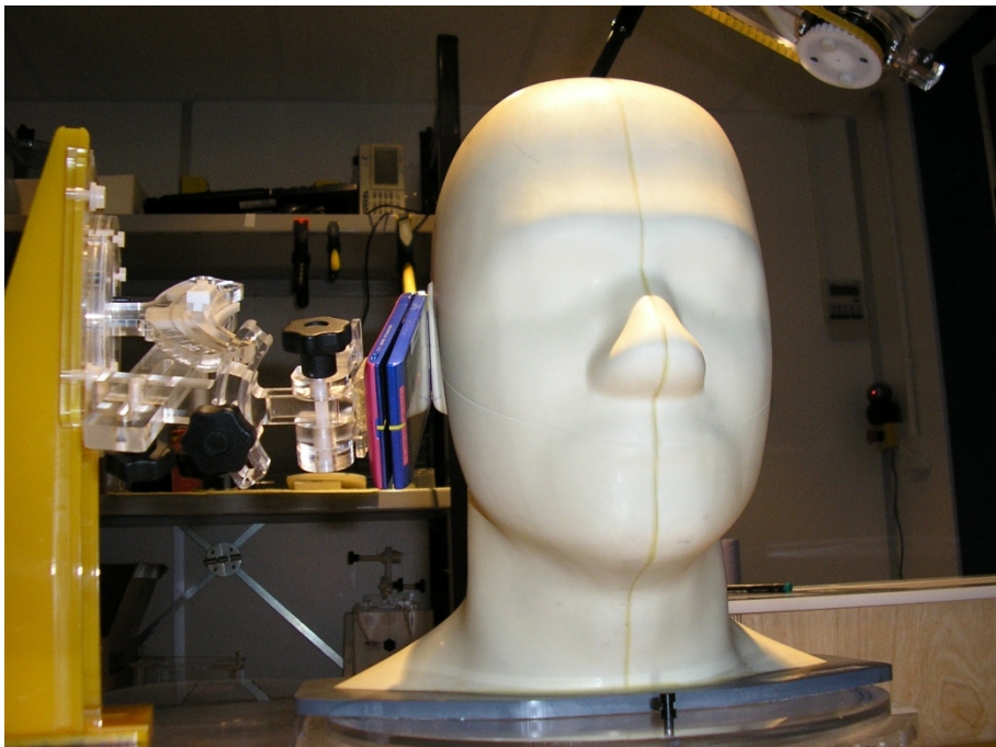
Figure 25 Right Hand 15°
