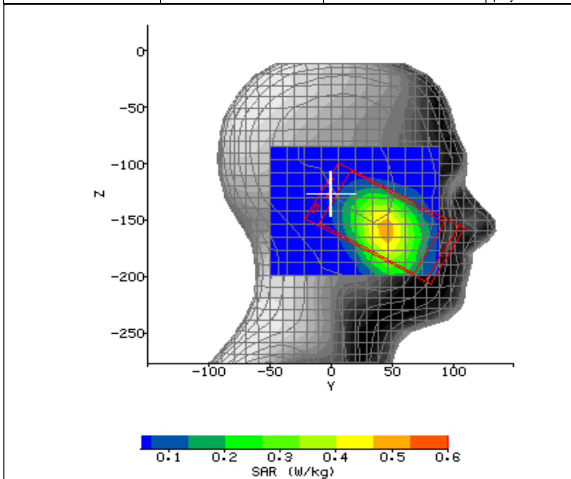
Figure 10: SAR Head Testing Results for the CDMA SHI11 Mobile Handset at 824.7MHz.
