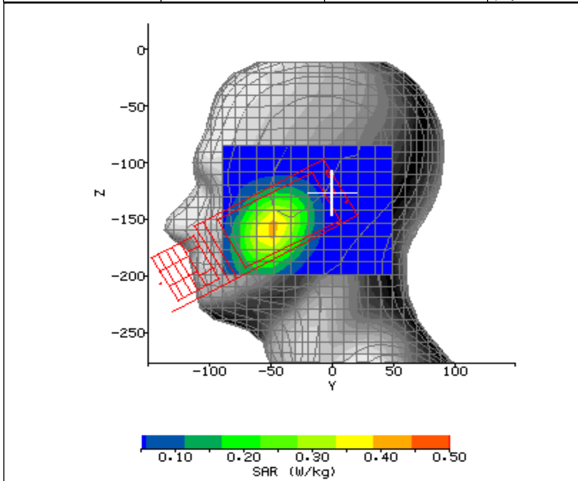
Figure 12: SAR Head Testing Results for the CDMA SHI11 Mobile Handset at 824.7MHz.
