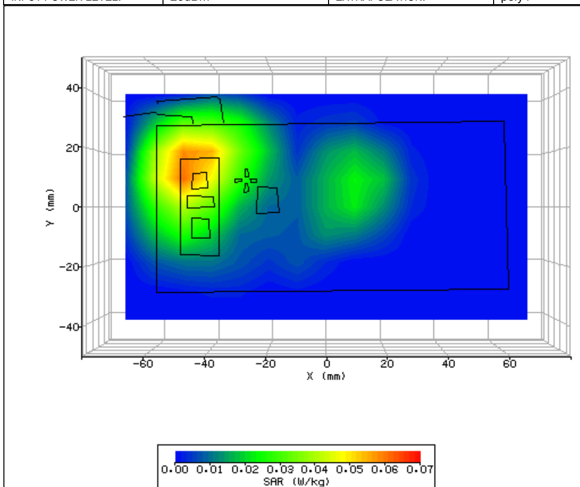
Figure 21: SAR Body Testing Results for the CDMA SHI11 Mobile Handset at 2437.0MHz.
