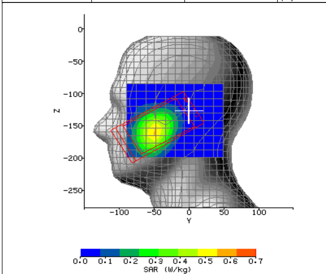
Figure 8: SAR Head Testing Results for the CDMA SHI11 Mobile Handset at 824.7MHz.
