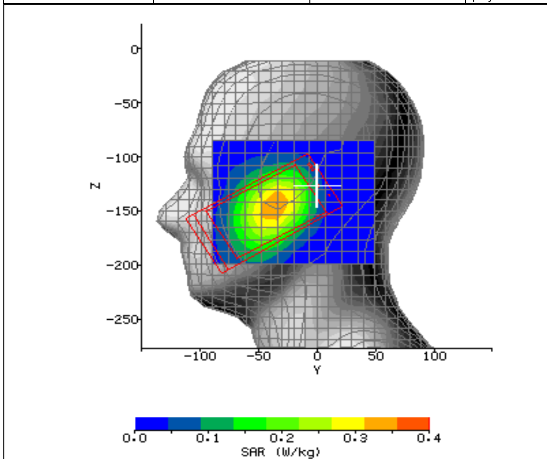
Figure 9: SAR Head Testing Results for the CDMA SHI11 Mobile Handset at 824.7MHz.
