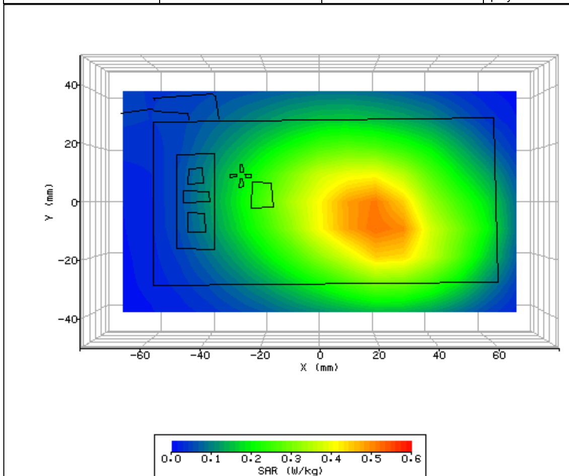
Figure 14: SAR Body Testing Results for the CDMA SHI11 Mobile Handset at 824.7MHz.
