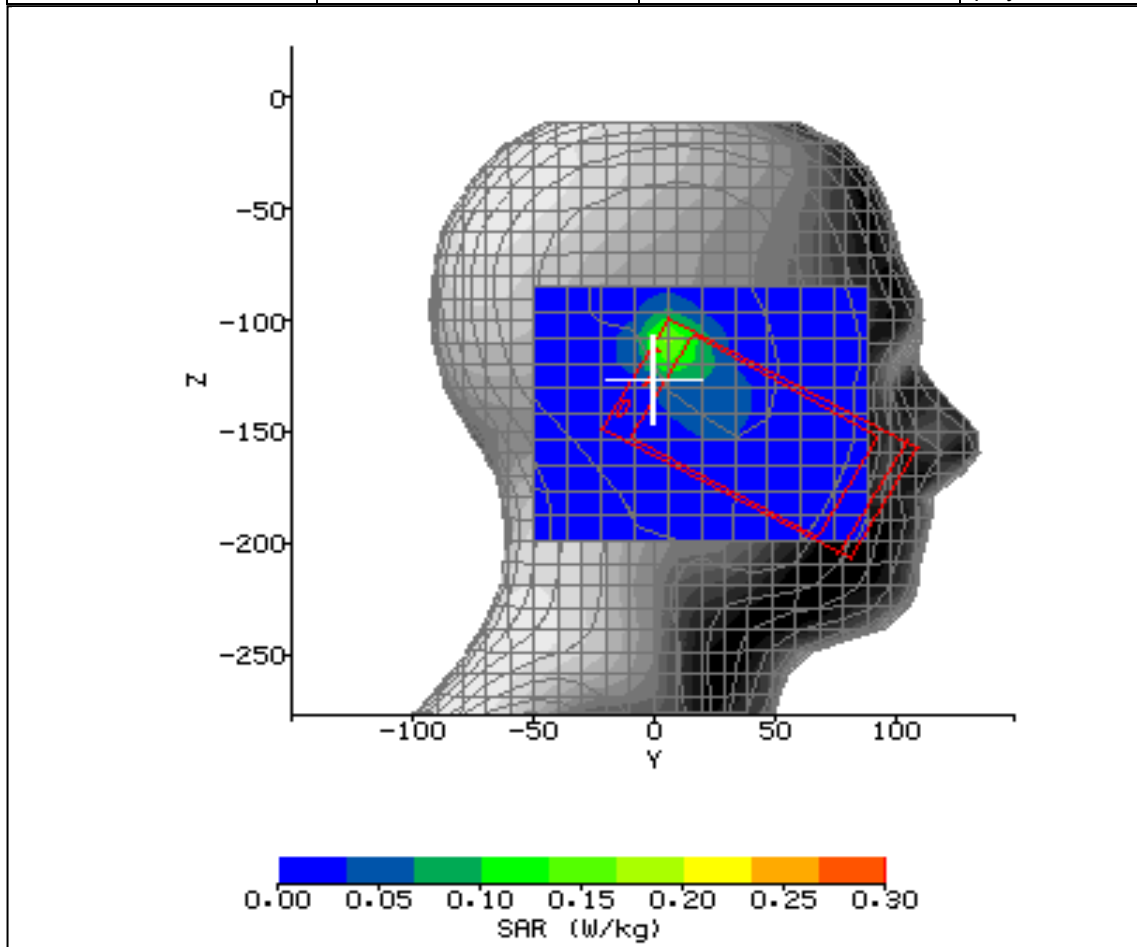
Figure 18: SAR Head Testing Results for the CDMA SHI11 Mobile Handset at 2437.0MHz.
