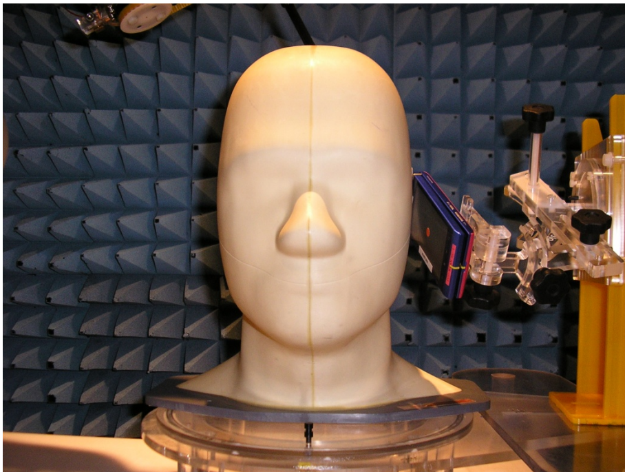
Figure 23 Left Hand 15°
