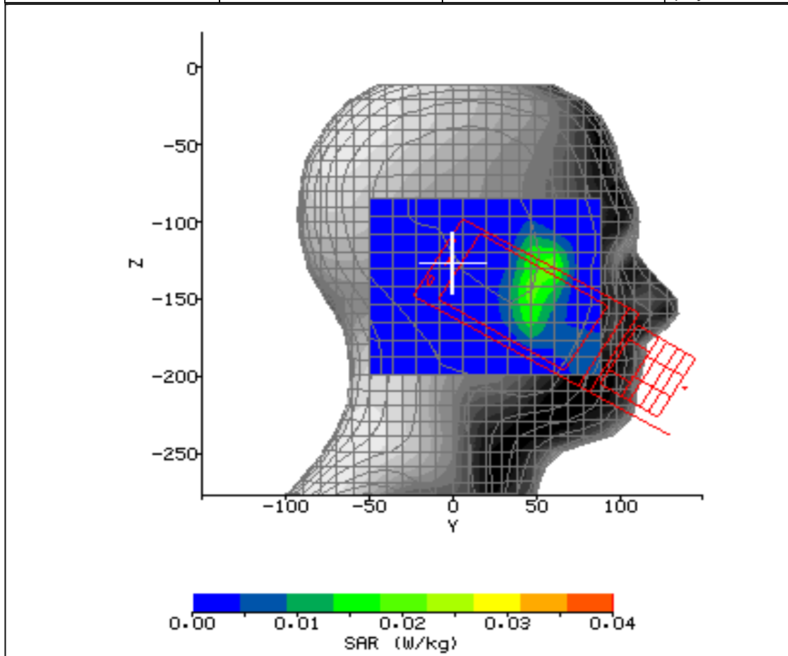
Figure 19: SAR Head Testing Results for the CDMA SHI11 Mobile Handset at 2437.0MHz.
