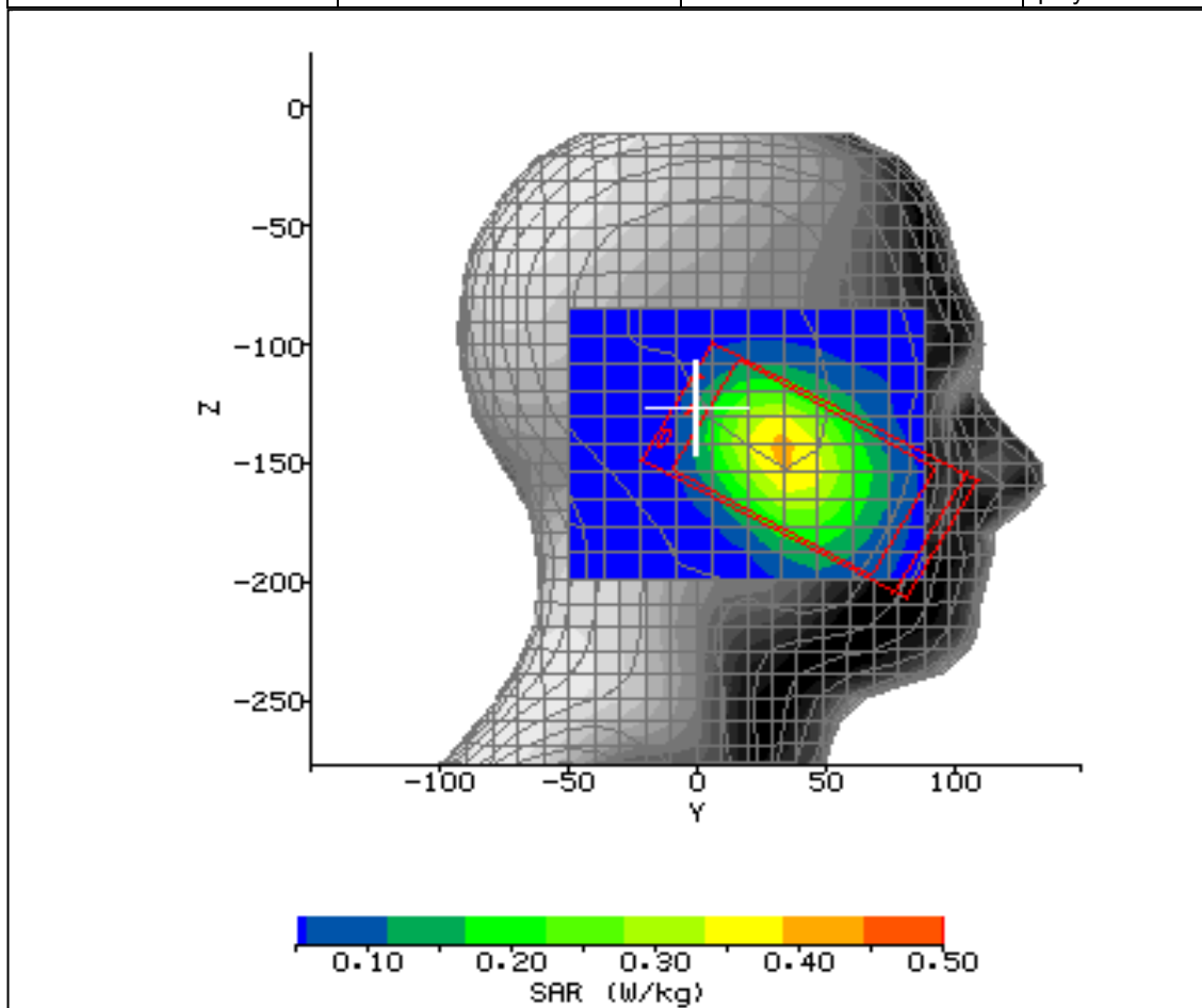
Figure 11: SAR Head Testing Results for the CDMA SHI11 Mobile Handset at 824.7MHz.
