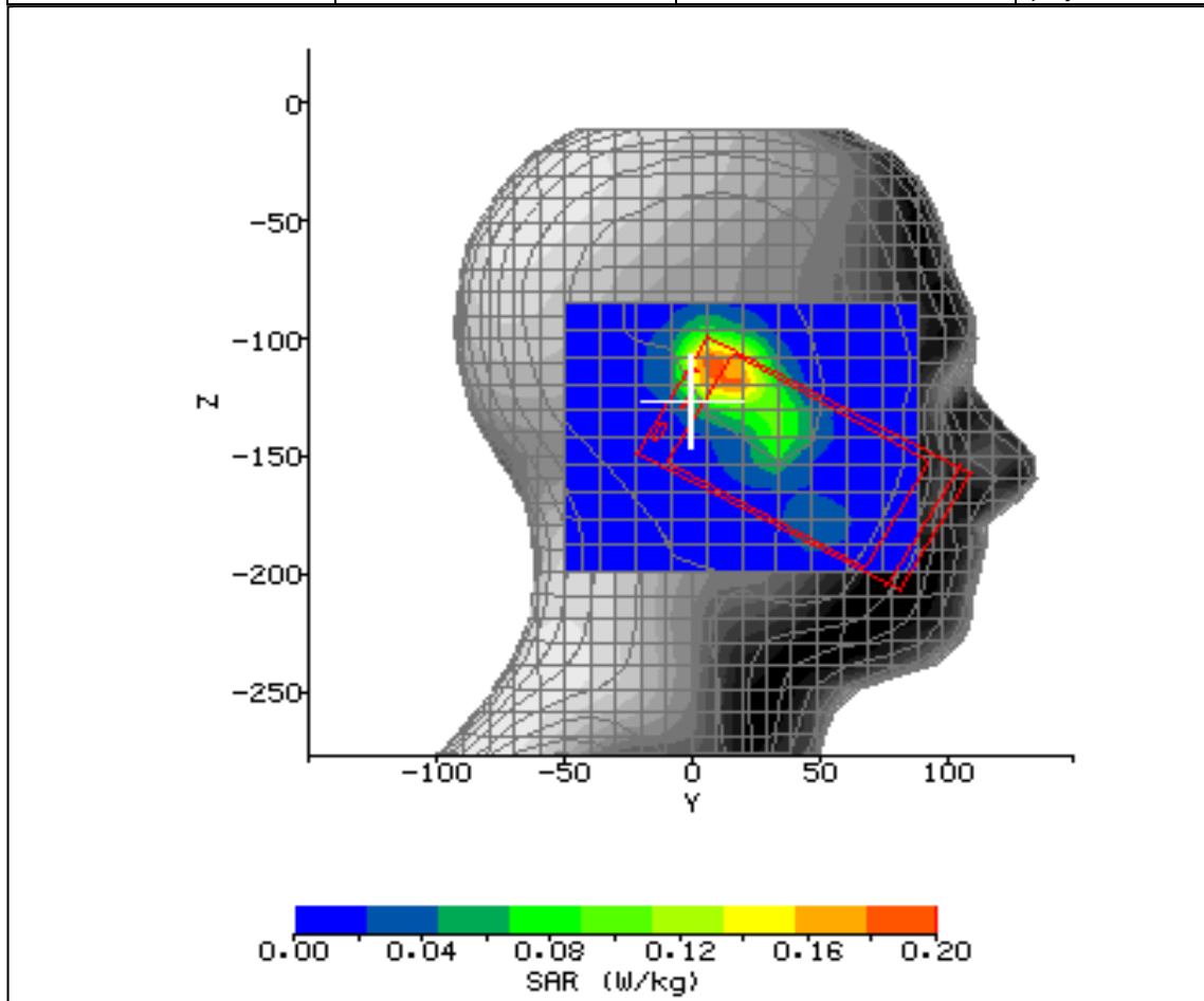
Figure 17: SAR Head Testing Results for the CDMA SHI11 Mobile Handset at 2437.0MHz.
