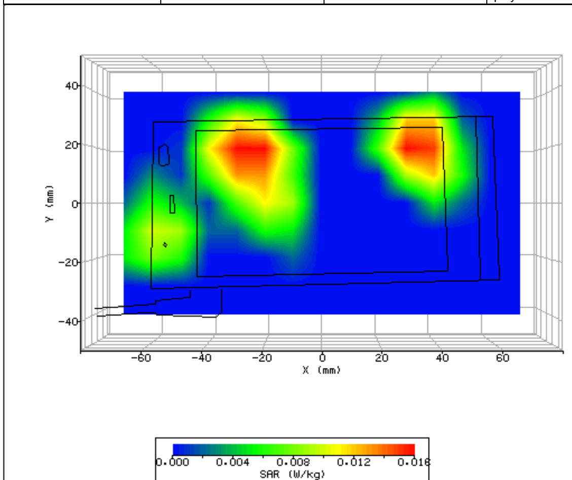
Figure 20: SAR Body Testing Results for the CDMA SHI11 Mobile Handset at 2437.0MHz.
