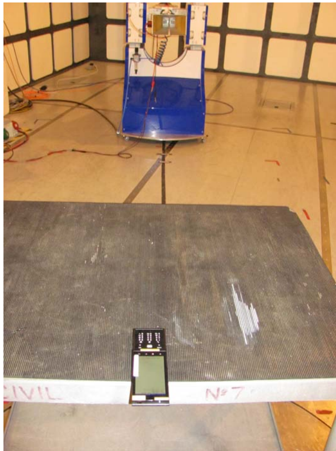
1GHz-18GHz – Radiated Emissions
