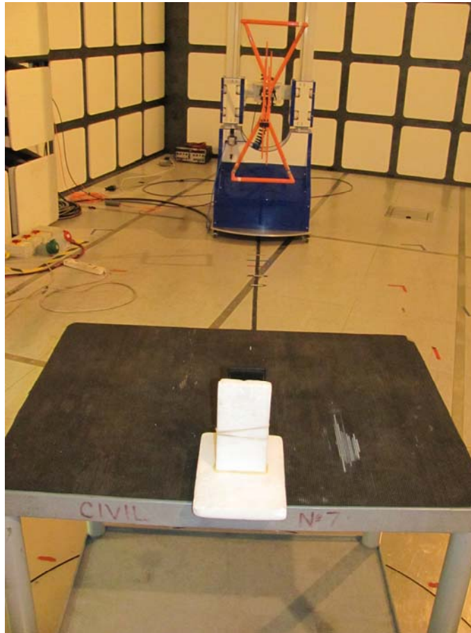
30MHz-1GHz Radiated Emissions
