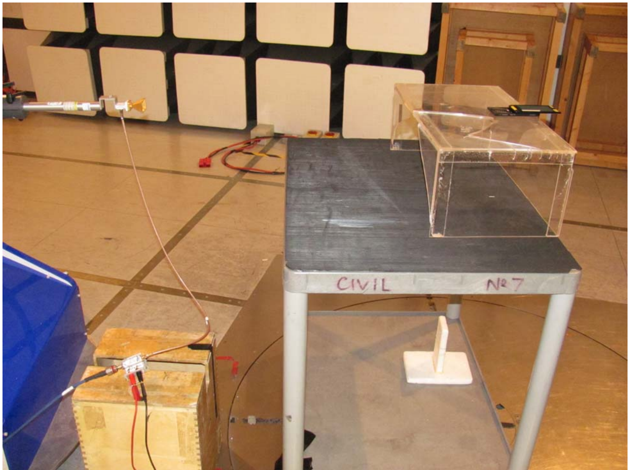
18GHz-25GHz – Radiated Emissions
