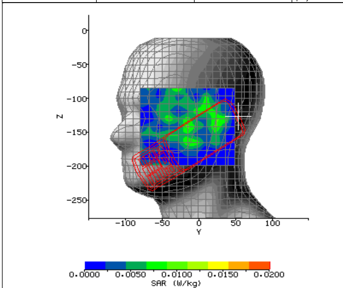
Figure 22: SAR Head Testing Results for the Sharp CDMA SHI15 at 2412MHz.
