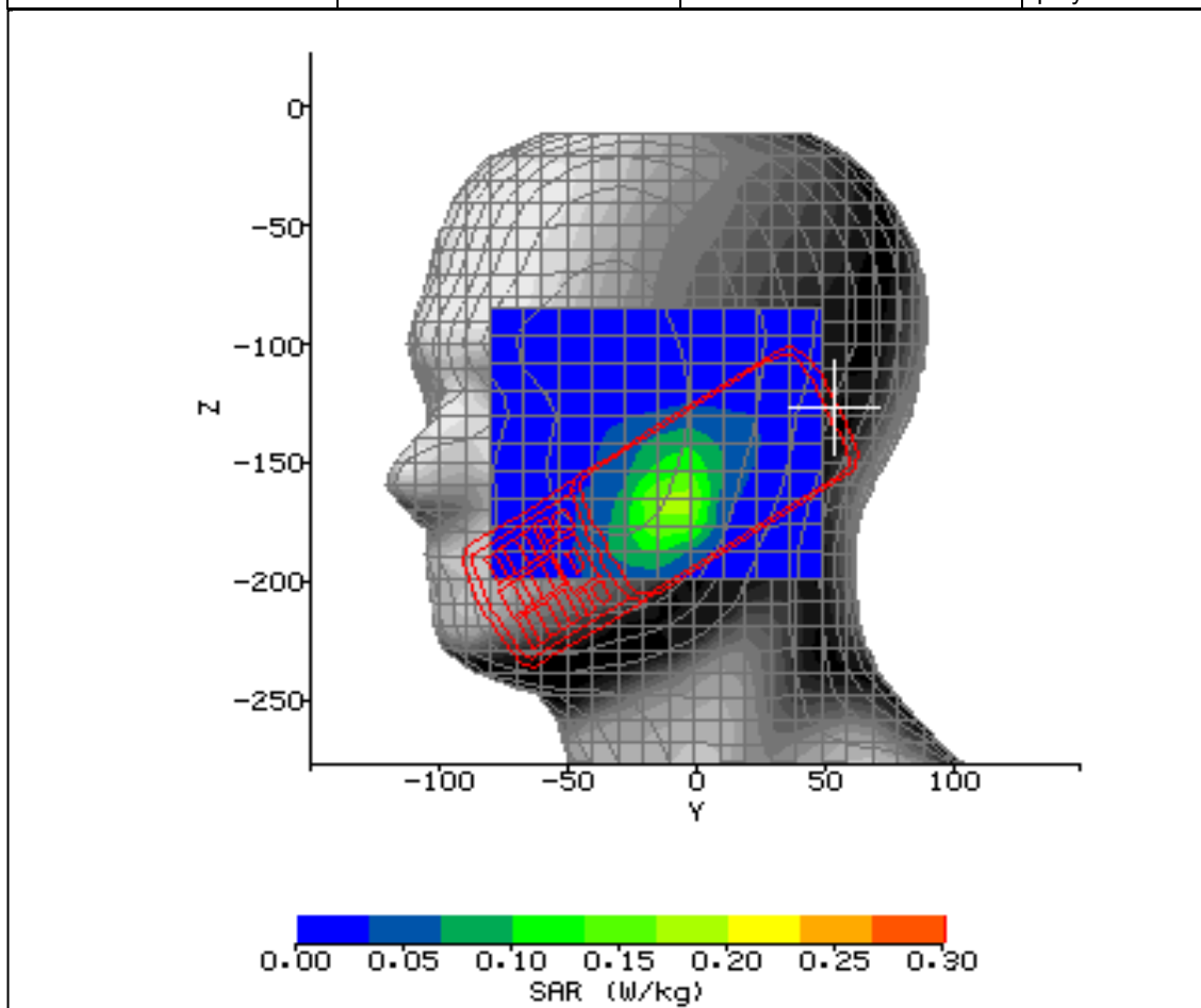
Figure 15: SAR Head Testing Results for the Sharp CDMA SHI15 at 1850.2MHz.
