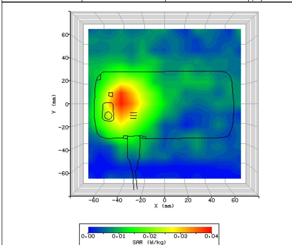
Figure 28: SAR Body Testing Results for the Sharp CDMA SHI15 at 2412MHz.
