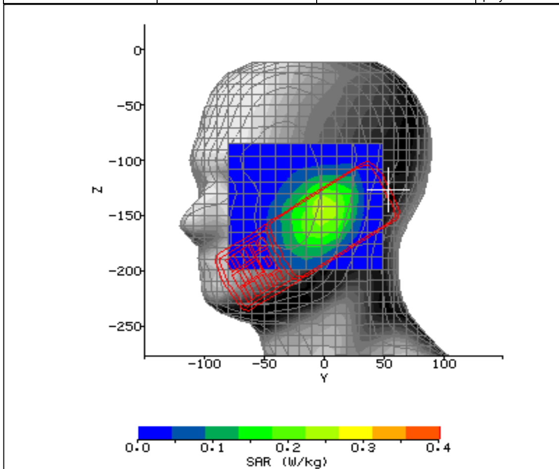
Figure 9: SAR Head Testing Results for the Sharp CDMA SHI15 at 848.31MHz.
