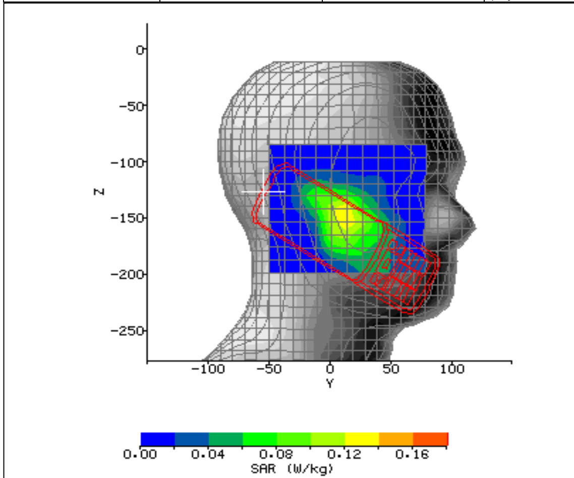
Figure 17: SAR Head Testing Results for the Sharp CDMA SHI15 at 1850.2MHz.
