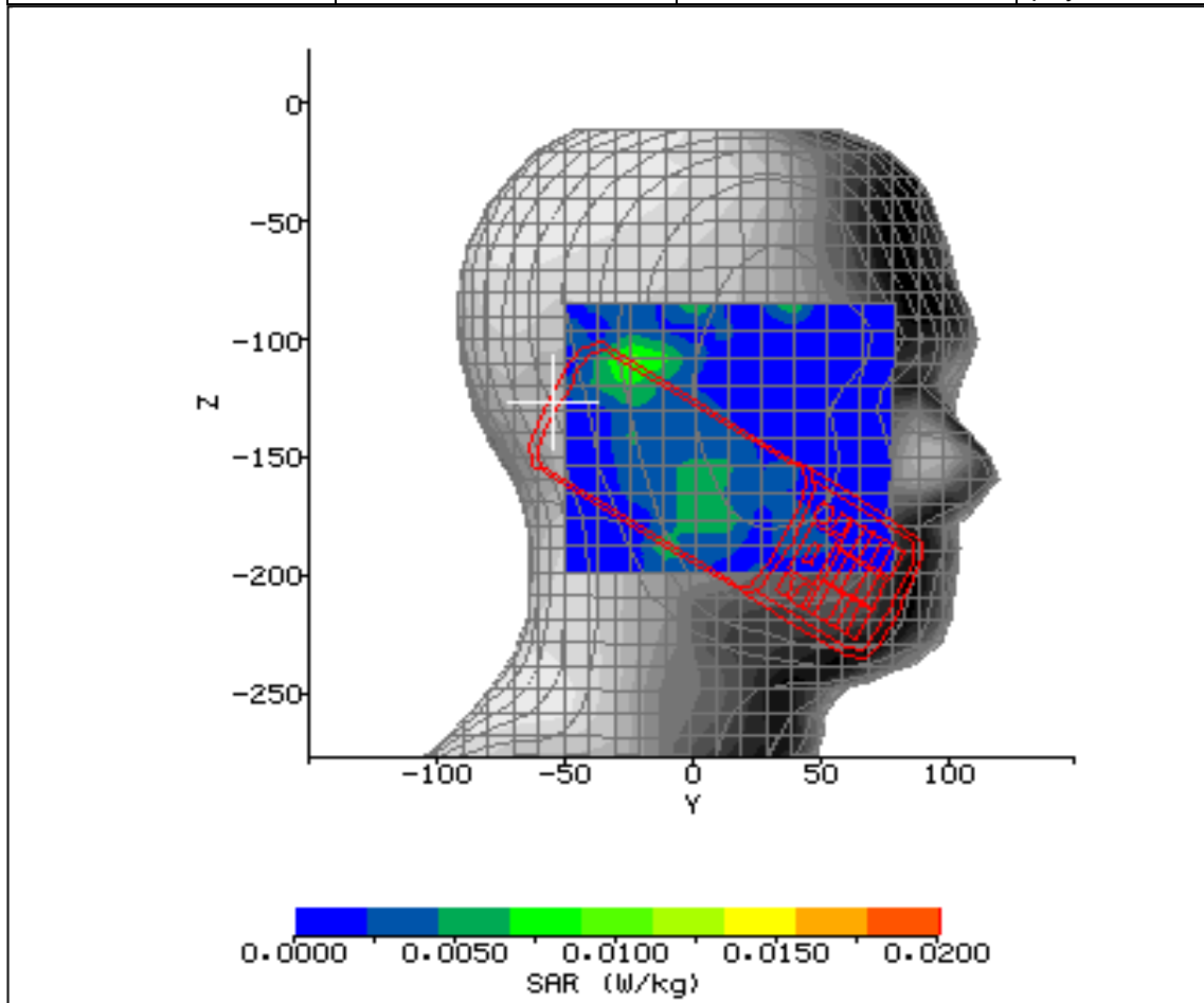
Figure 25: SAR Head Testing Results for the Sharp CDMA SHI15 at 2412MHz.
