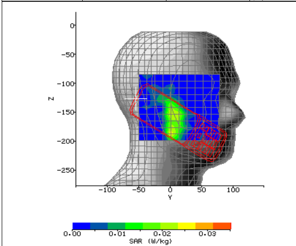
Figure 24: SAR Head Testing Results for the Sharp CDMA SHI15 at 2412MHz.
