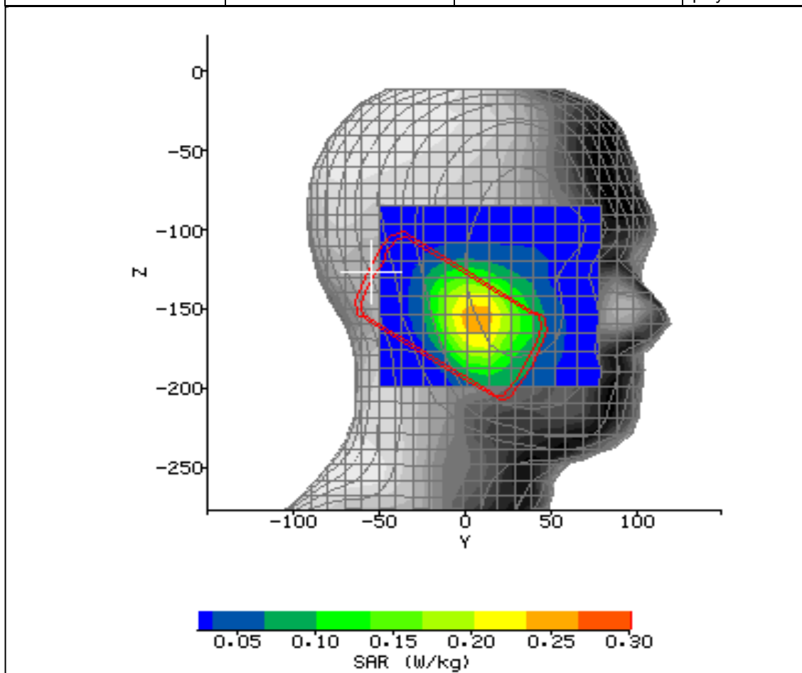
Figure 12: SAR Head Testing Results for the Sharp CDMA SHI15 at 848.31MHz.
