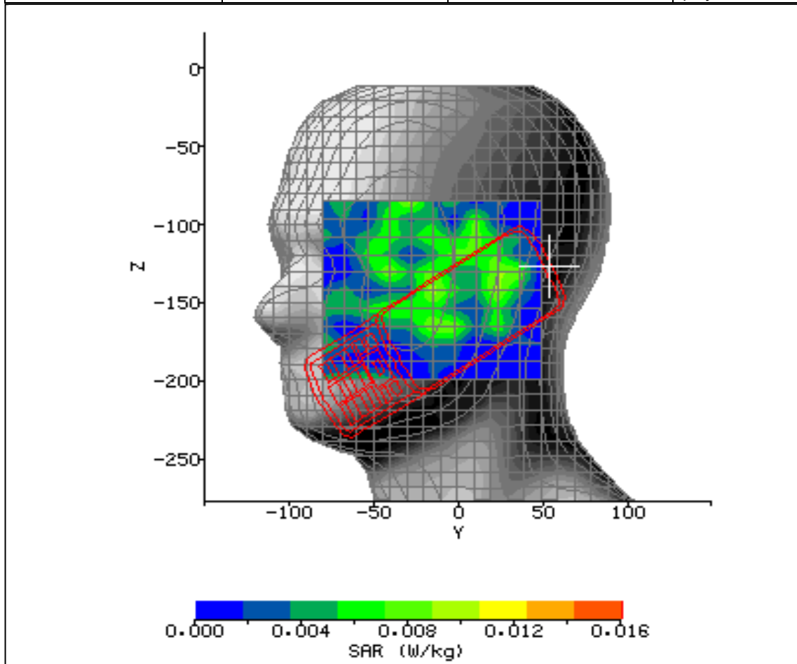
Figure 23: SAR Head Testing Results for the Sharp CDMA SHI15 at 2412MHz.
