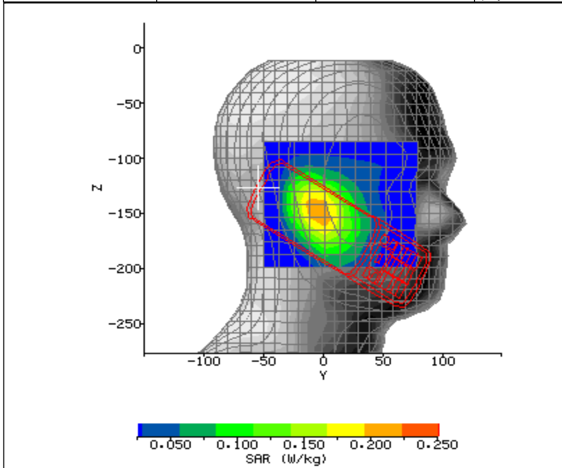
Figure 11: SAR Head Testing Results for the Sharp CDMA SHI15 at 848.31MHz.
