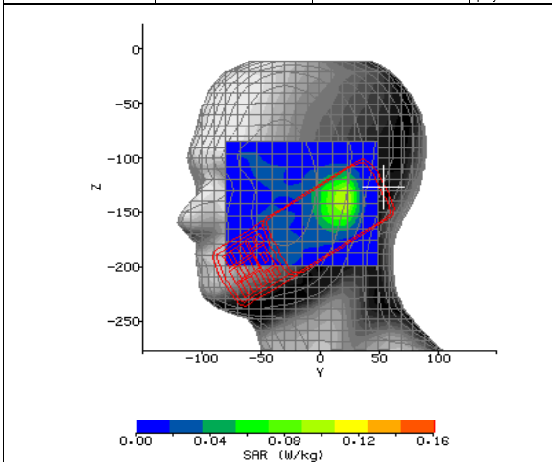
Figure 16: SAR Head Testing Results for the Sharp CDMA SHI15 at 1850.2MHz.
