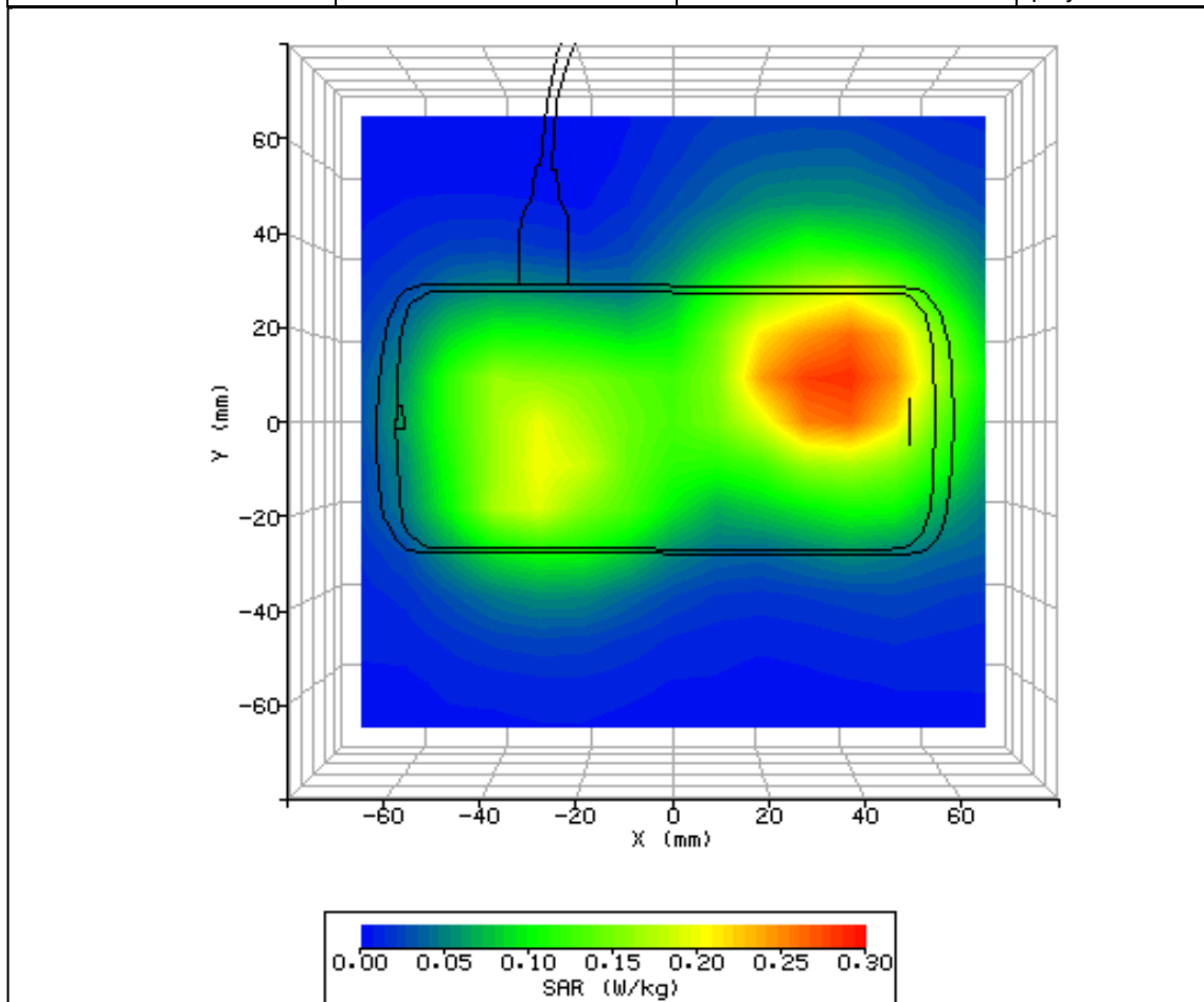
Figure 20: SAR Body Testing Results for the Sharp CDMA SHI15 at 1850.2MHz.
