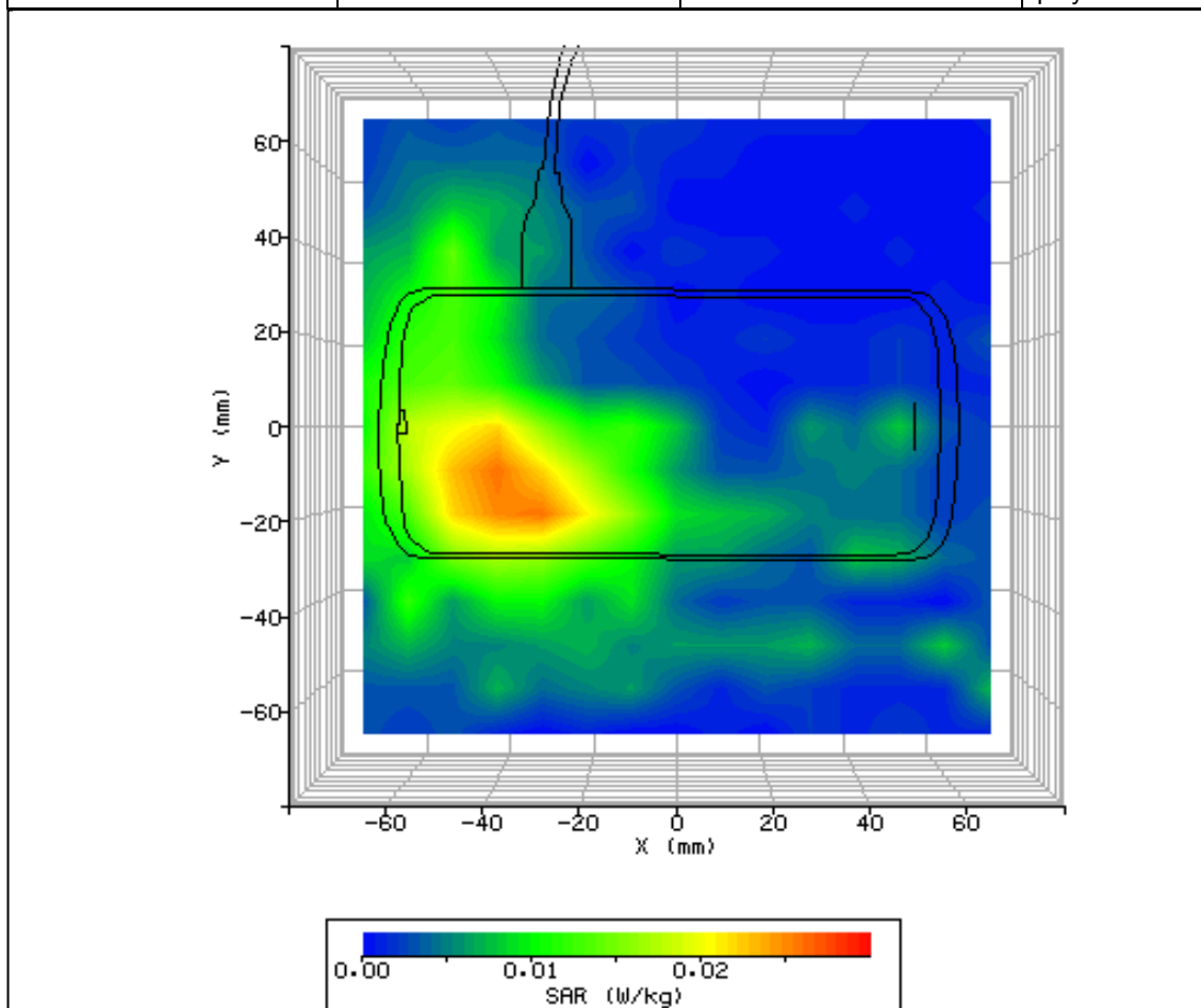
Figure 27: SAR Body Testing Results for the Sharp CDMA SHI15 at 2412MHz.
