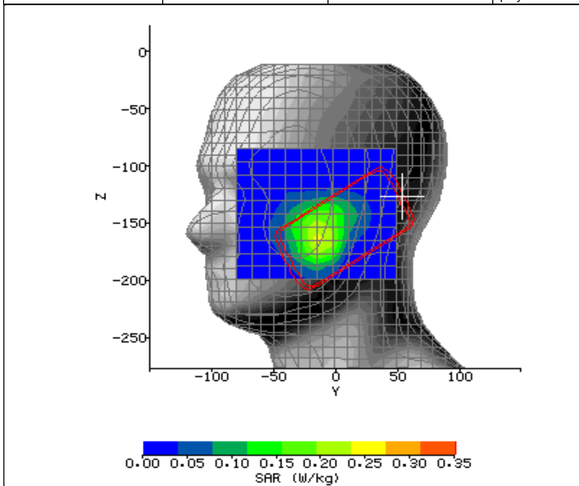
Figure 19: SAR Head Testing Results for the Sharp CDMA SHI15 at 1850.2MHz.
