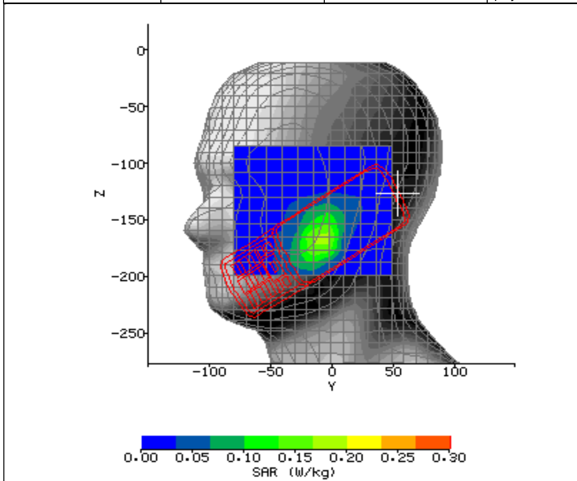
Figure 15: SAR Head Testing Results for the Sharp CDMA SHI15 at 1850.2MHz.
