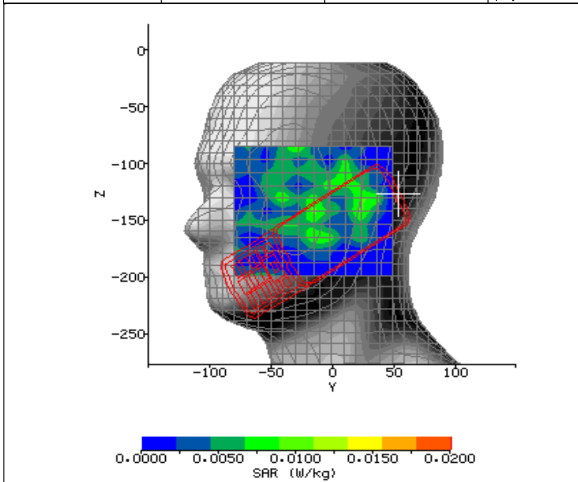
Figure 22: SAR Head Testing Results for the Sharp CDMA SHI15 at 2412MHz.
