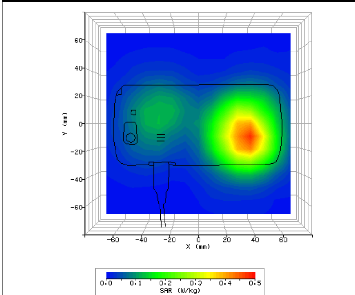
Figure 21: SAR Body Testing Results for the Sharp CDMA SHI15 at 1850.2MHz.
