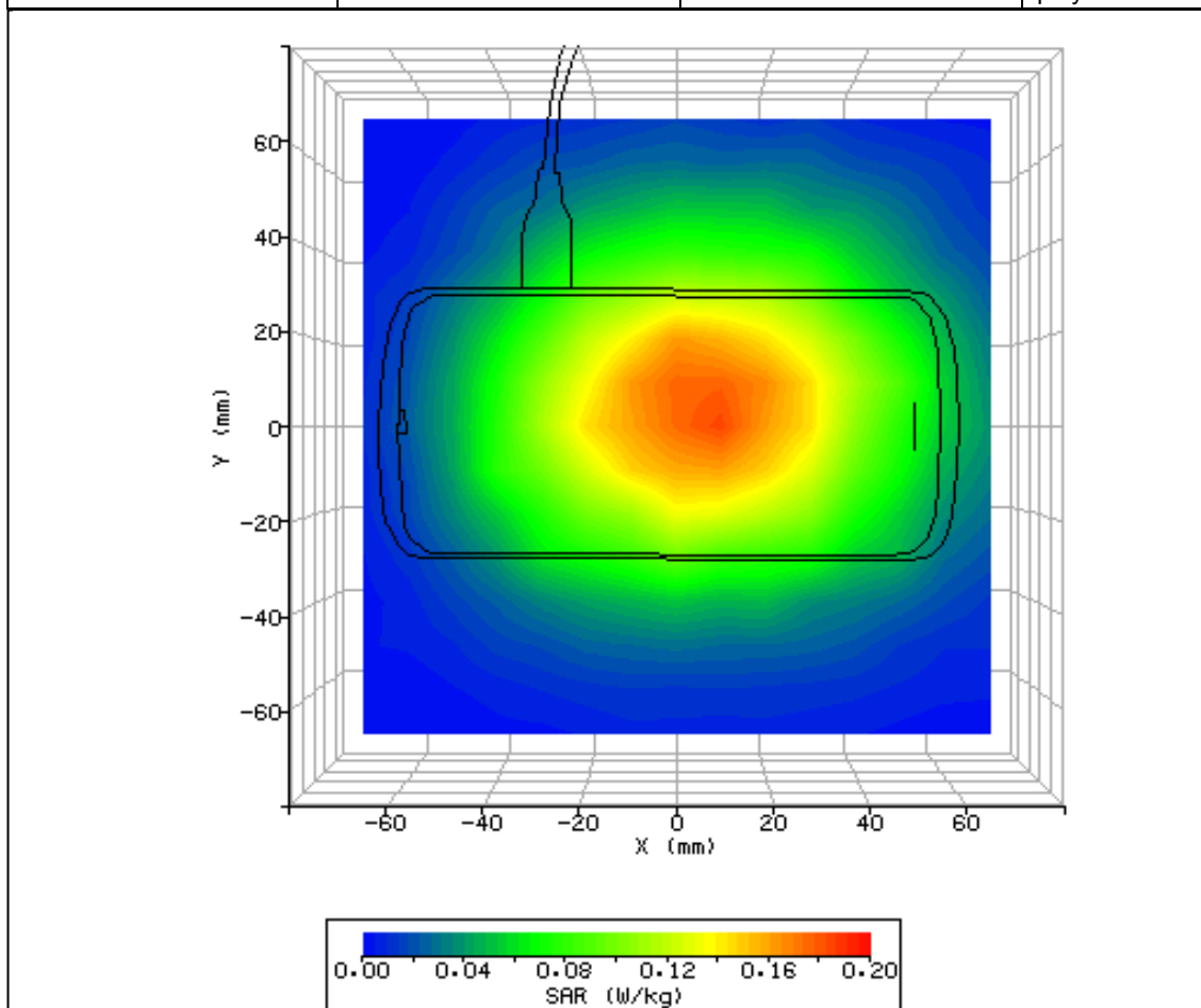
Figure 13: SAR Body Testing Results for the Sharp CDMA SHI15 at 848.31MHz.
