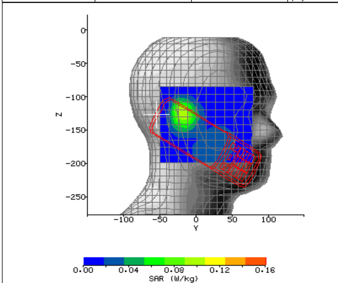
Figure 18: SAR Head Testing Results for the Sharp CDMA SHI15 at 1850.2MHz.
