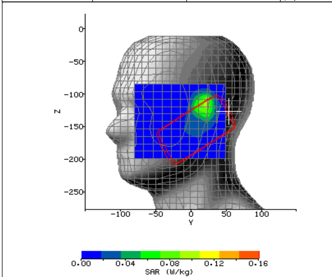
Figure 26: SAR Head Testing Results for the Sharp CDMA SHI15 at 2412MHz.
