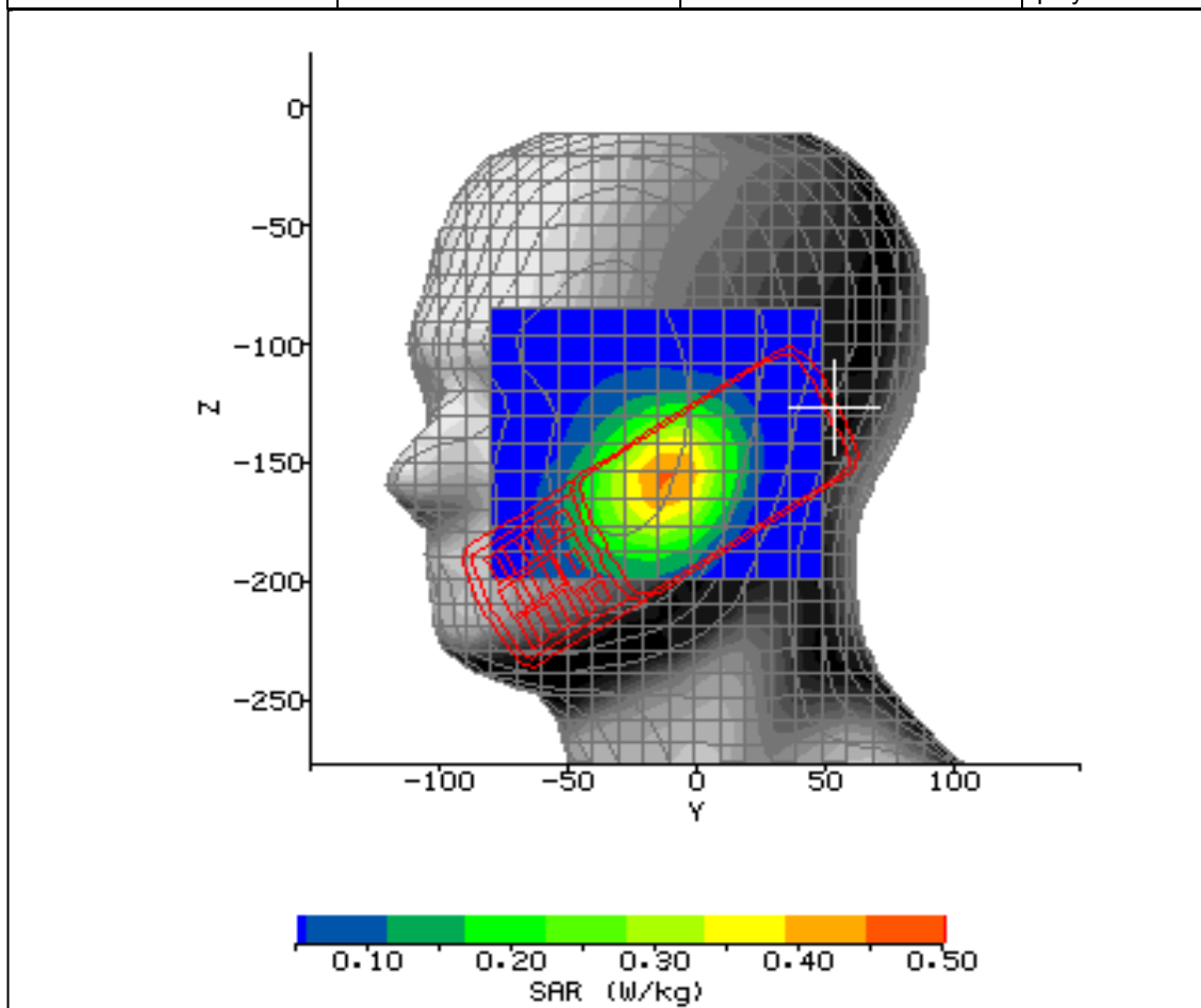
Figure 8: SAR Head Testing Results for the Sharp CDMA SHI15 at 848.31MHz.
