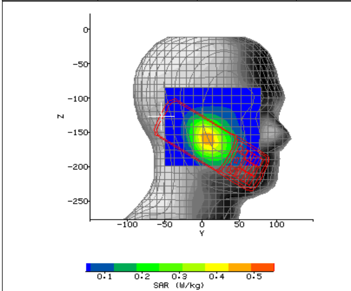
Figure 10: SAR Head Testing Results for the Sharp CDMA SHI15 at 848.31MHz.
