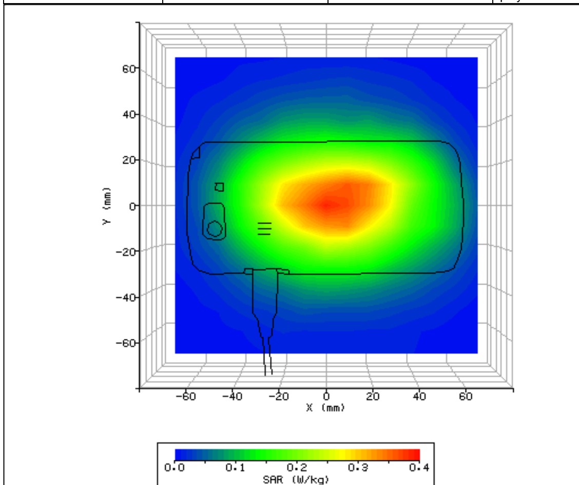
Figure 14: SAR Body Testing Results for the Sharp CDMA SHI15 at 848.31MHz.
